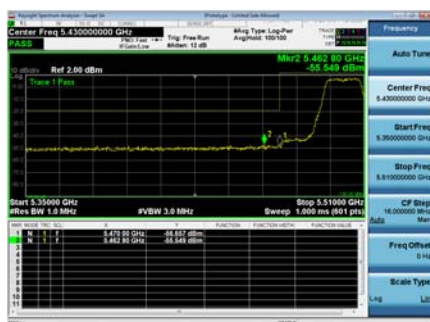
Antenna C
