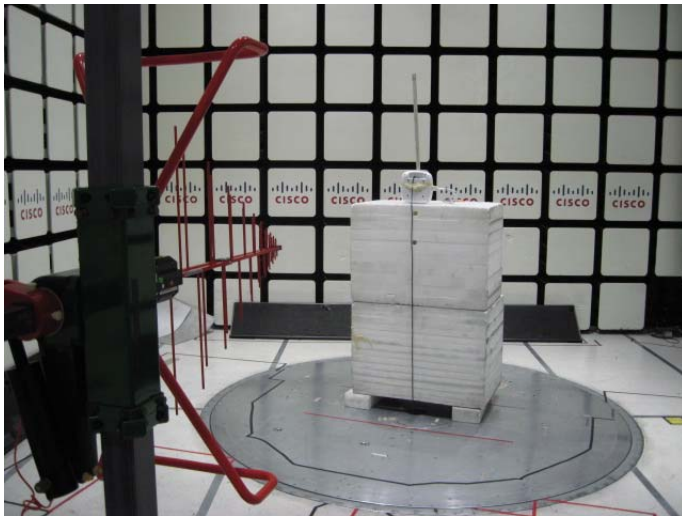
Title: Radiated Emissions Configuration Photograph 30MHz-1GHz
