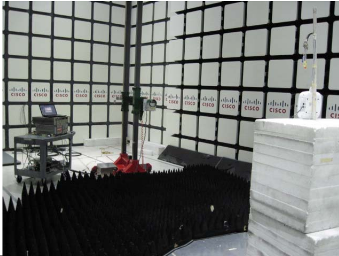
Title: Radiated Emissions Configuration Photograph 18GHz to 40GHz
