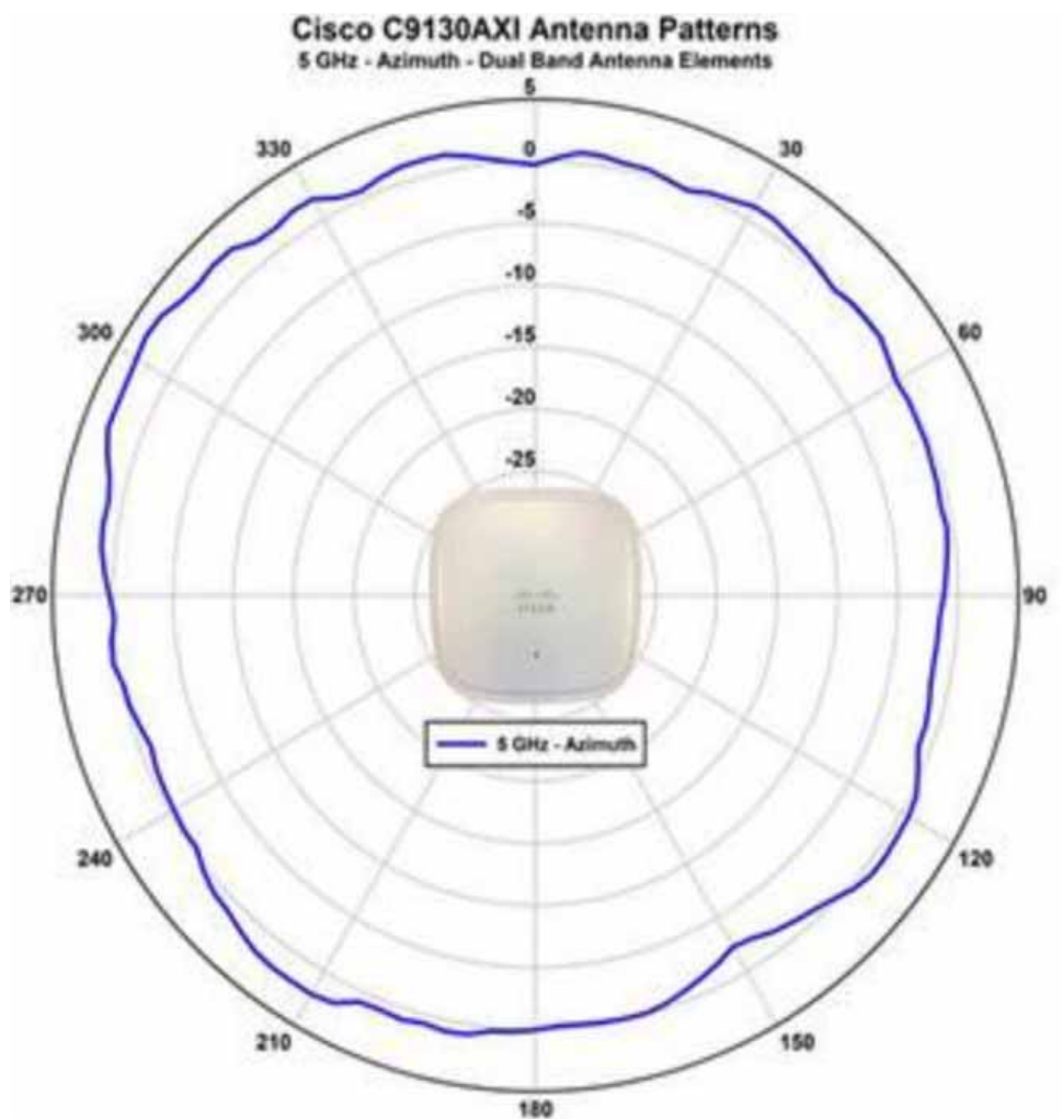
Figure 3-7 C9130AXI - Dual-band Antenna radiation pattern (5 GHz Azimuth)
