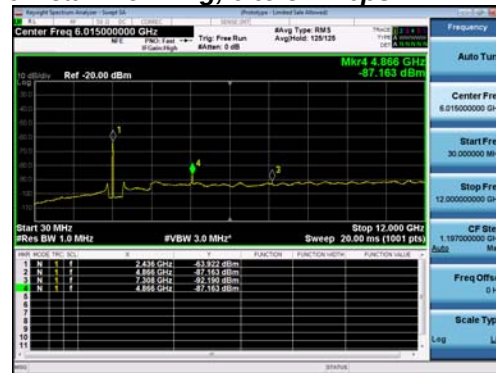
Antenna B
