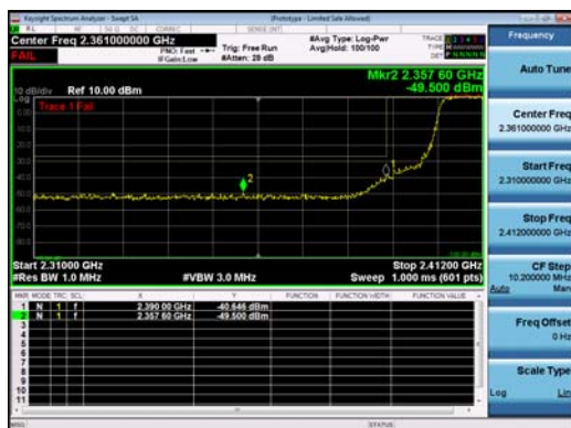
Antenna C
