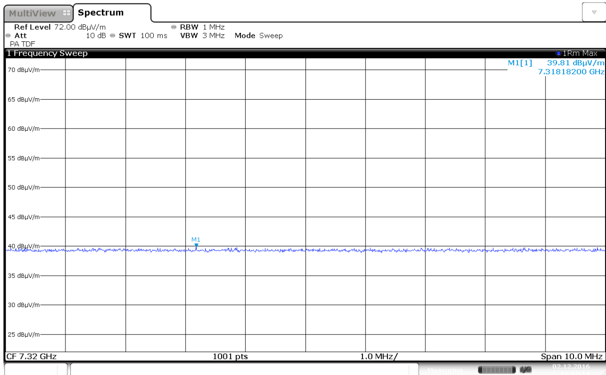
Radiated Emissions, 7320MHz, 2440MHz, HP, @1m
