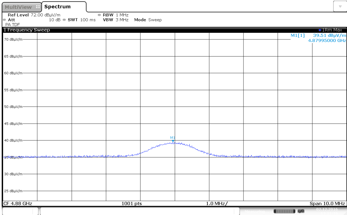
Radiated Emissions, 4880MHz, 2440MHz, HP, @1m
