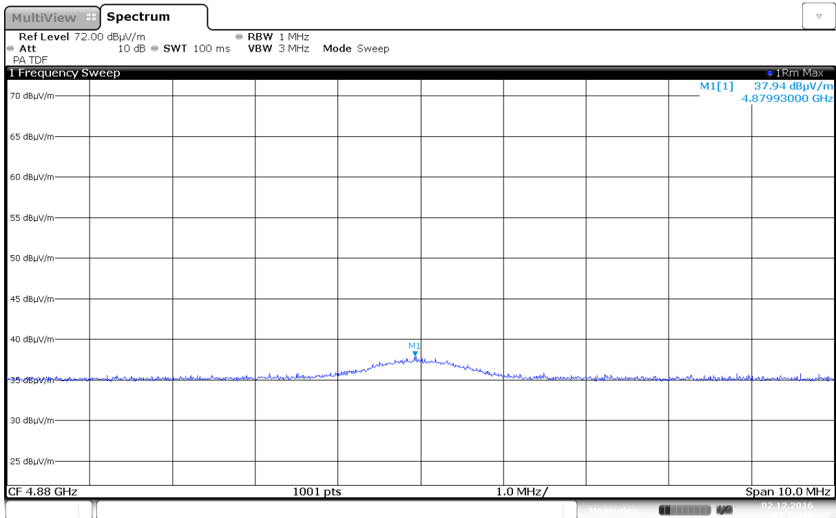
Radiated Emissions, 4880MHz, 2440MHz, VP, @1m
