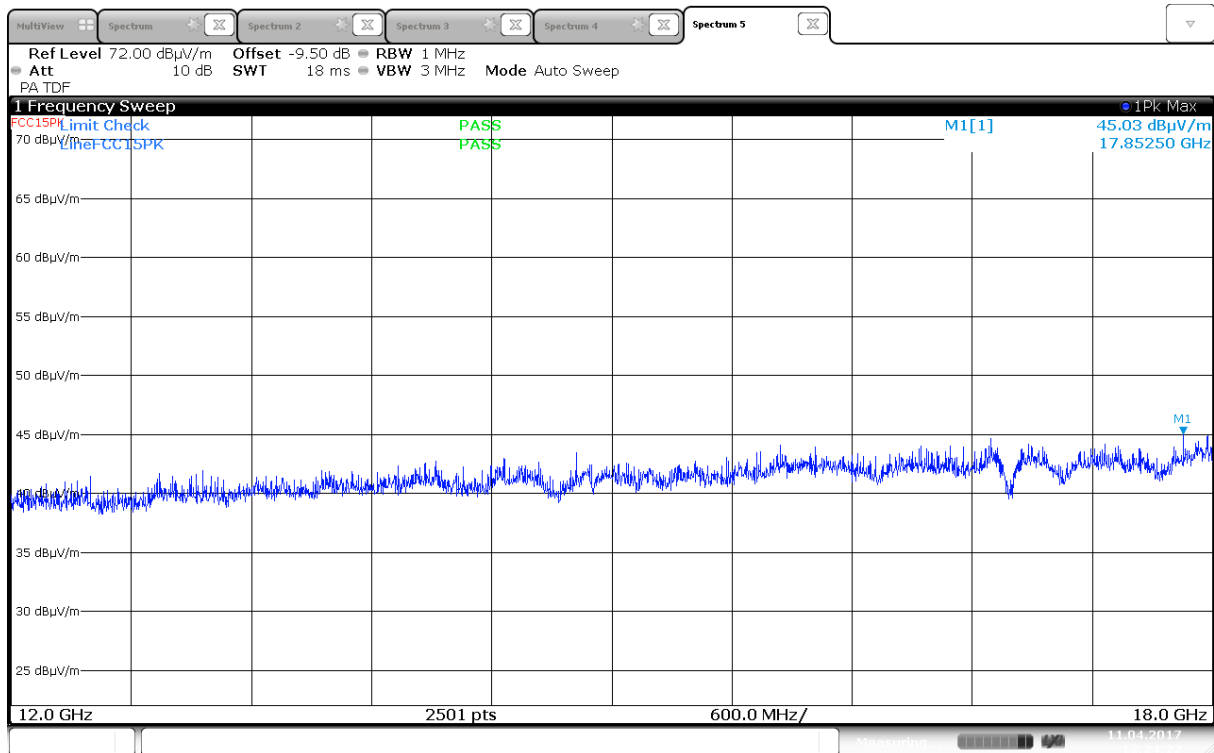
Radiated Emissions, 12000 -18000 MHz, 2437MHz, 802.11n, MCS0, MIMO, HP, @1m
