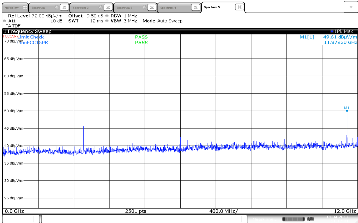
Radiated Emissions, 8000 -12000 MHz, 2437MHz, 802.11n, HT20, MIMO, HP, @1m
