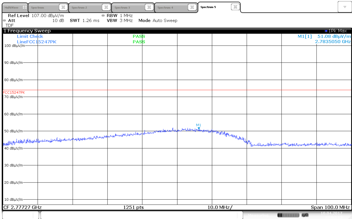
Radiated Emissions Pk, 2779MHz, 2452MHz (Max: HP) (Same for all RF-modulations and frequencies)
