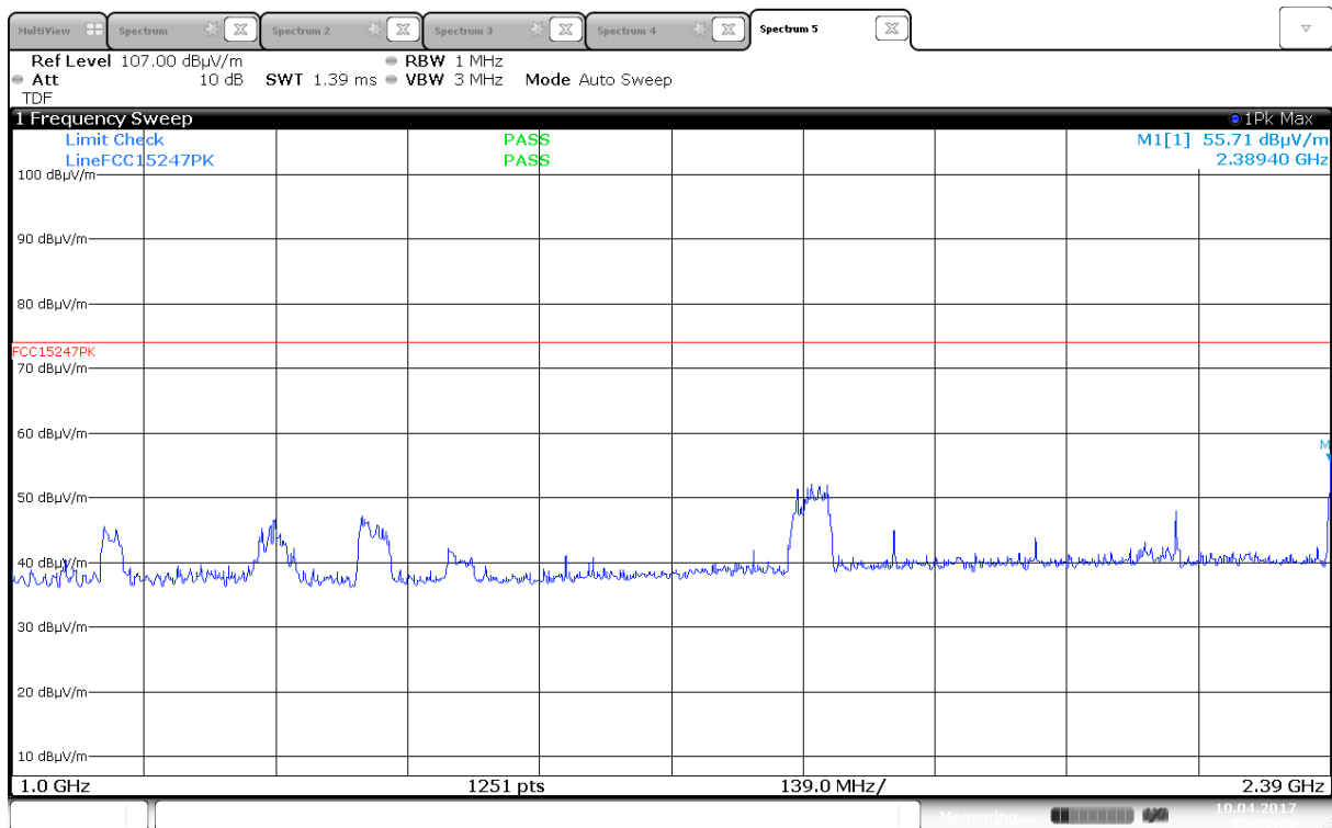
Radiated Emissions, 1000 -2390 MHz, 2412MHz, 802.11g, 6Mb, Ant0, HP
