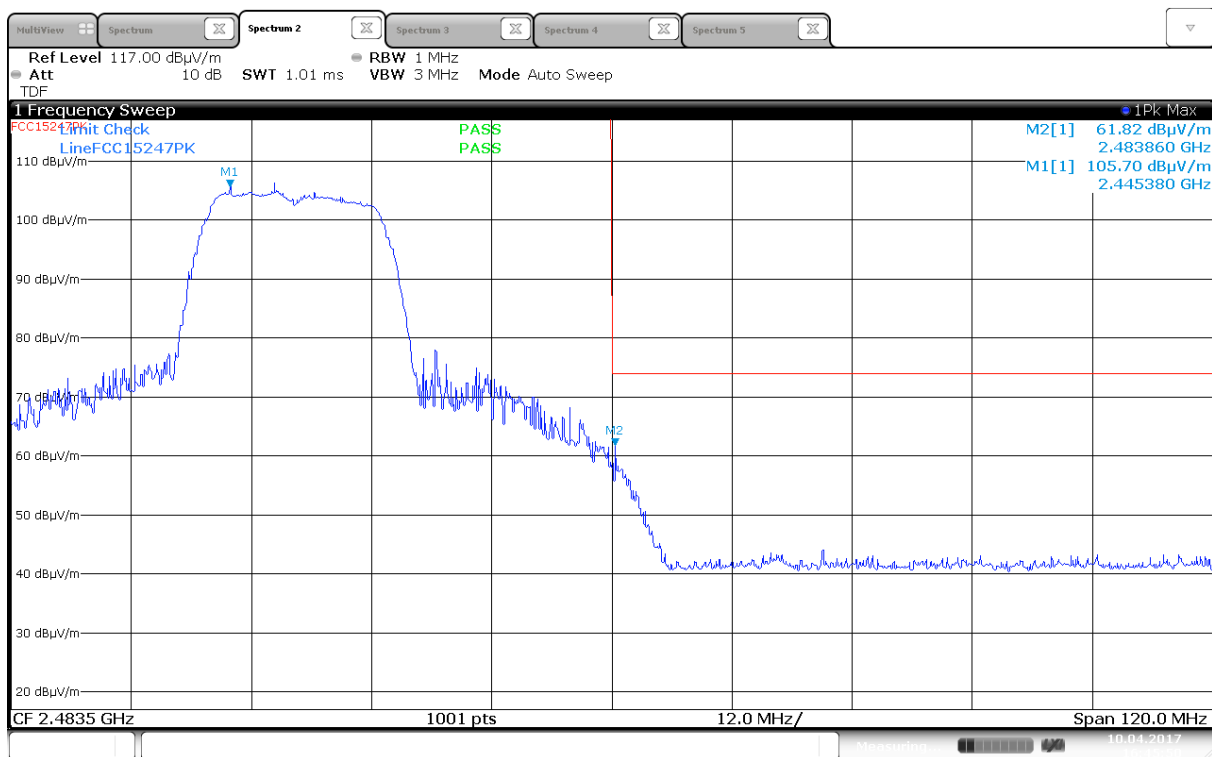
Upper Band Edge, Peak, 2452 MHz, 802.11n, MCS0, MIMO (Max: HP)
