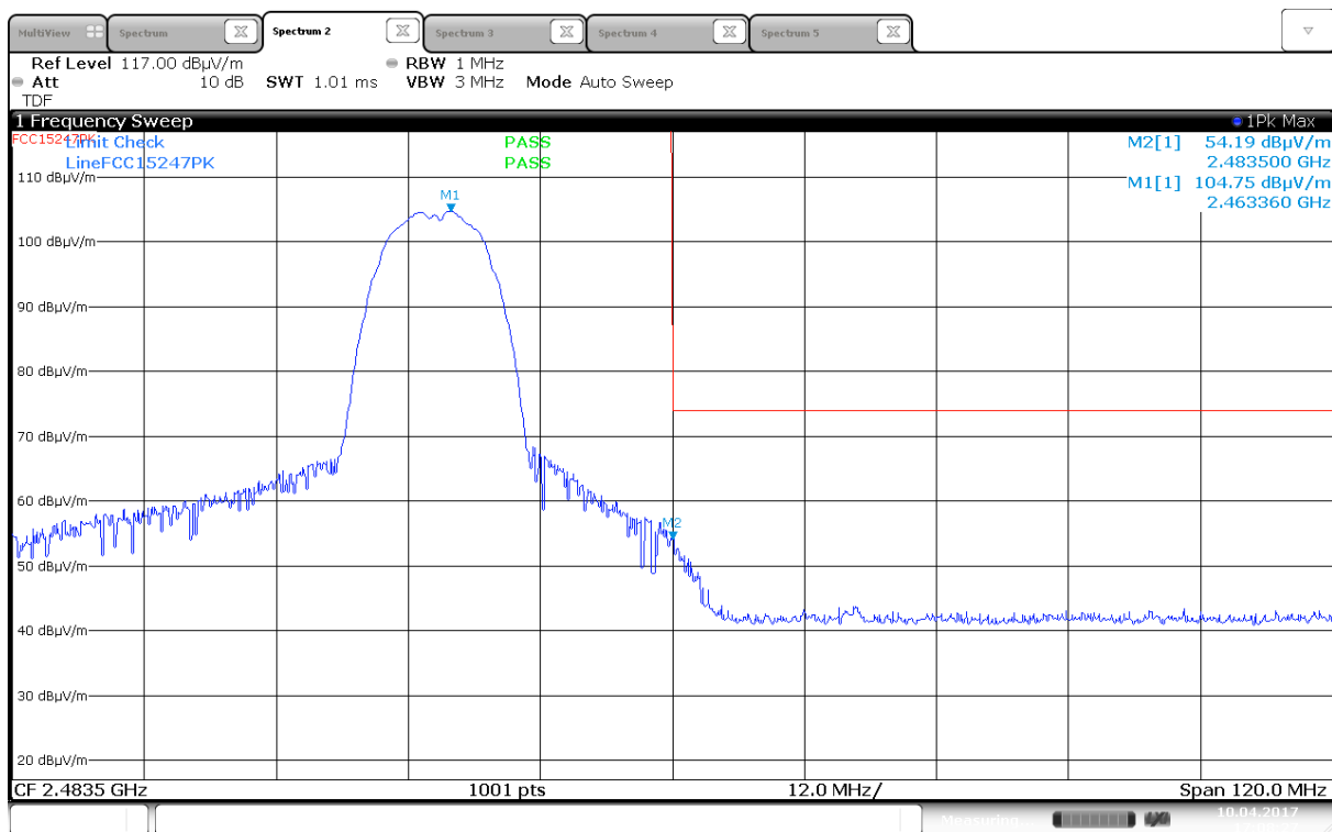
Upper Band Edge, Peak, 2462 MHz, 802.11b, 1Mbps, (Max: Ant 0, HP)
