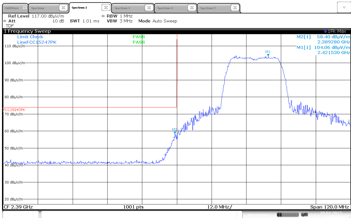
Lower Band Edge, Peak, 2417 MHz, 802.11n, MCS0, MIMO (Max: HP)
