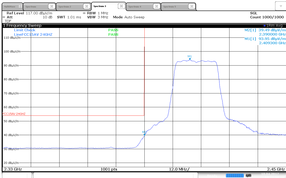
Lower Band Edge, Average, 2412 MHz, 802.11n, MCS0, MIMO (Max: HP)
