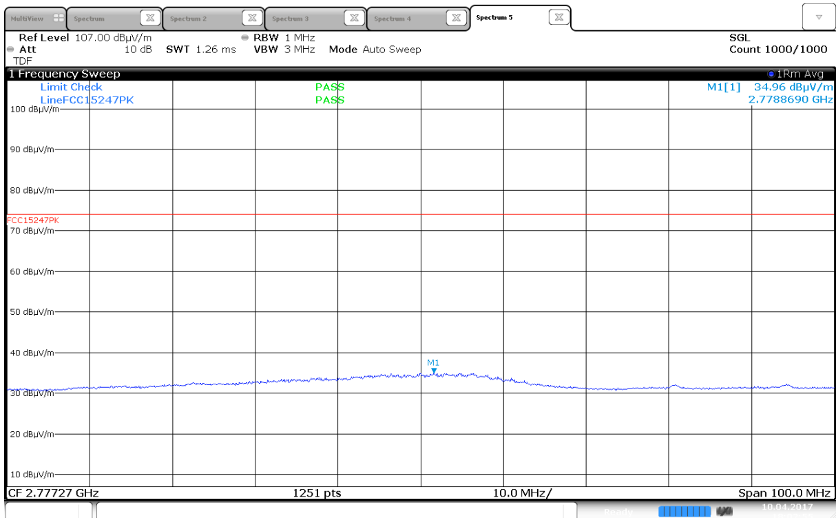
Radiated Emissions Av, 2779MHz, 2452MHz (Max: HP) (Same for all RF-modulations and frequencies)
