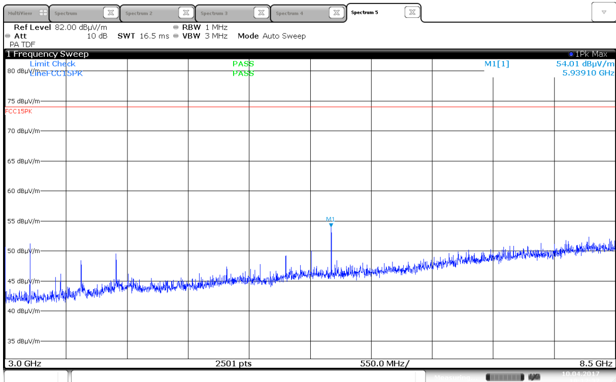
Radiated Emissions, 3000 -8500 MHz, 2437MHz, 802.11n, HT20, MIMO, VP
