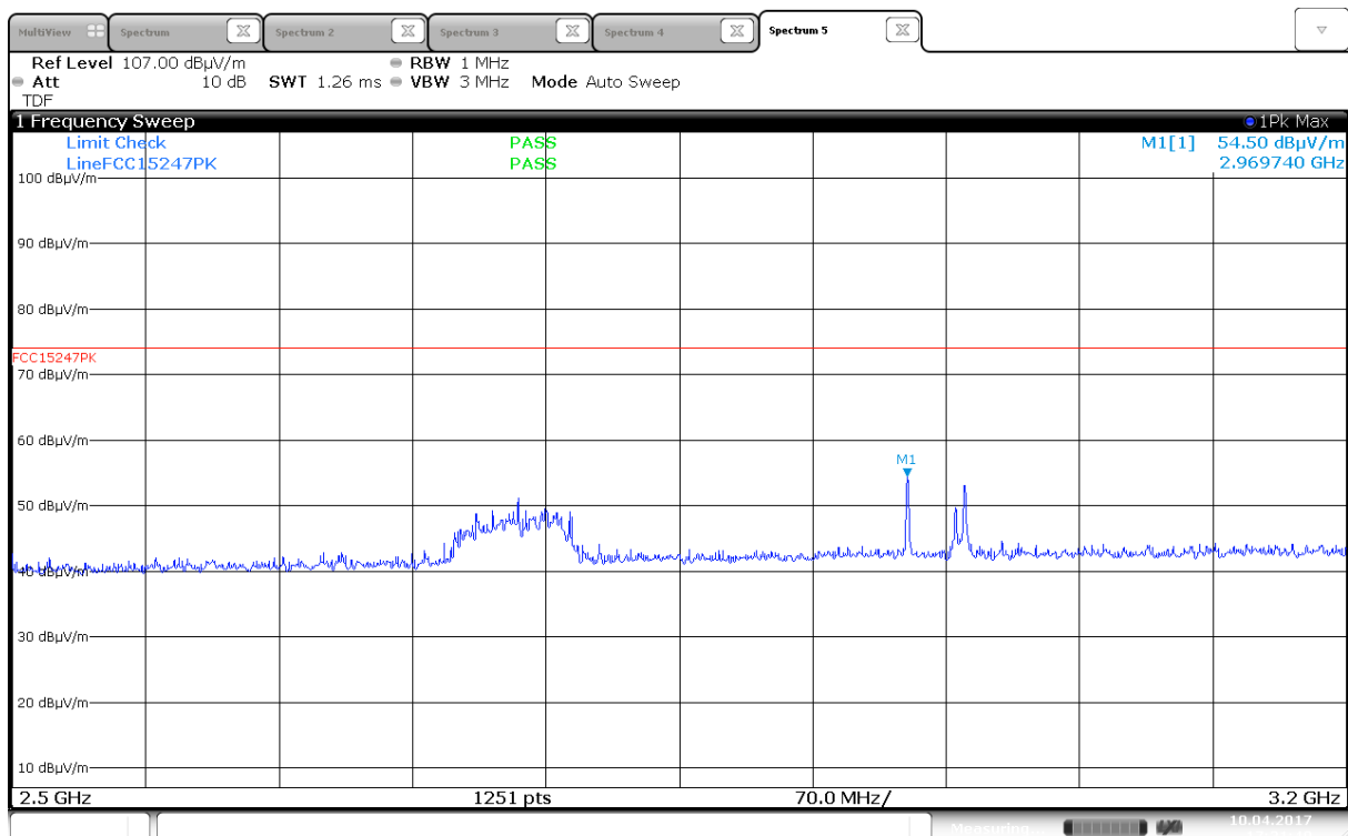
Radiated Emissions, 2500 -3200 MHz, 2462MHz, 802.11n, MCS0, MIMO, VP
