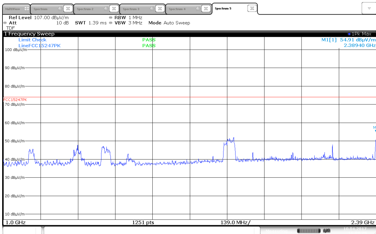
Radiated Emissions, 1000 -2390 MHz, 2412MHz, 802.11n, MCS0, MIMO, HP
