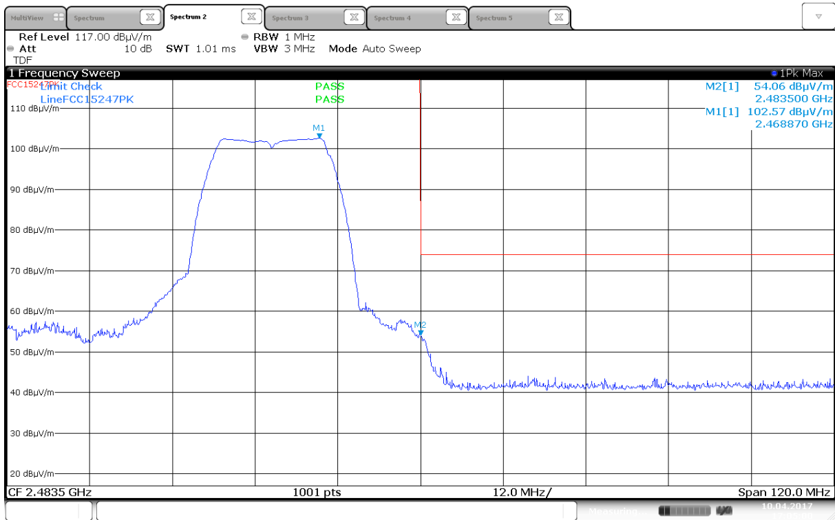
Upper Band Edge, Peak, 2462 MHz, 802.11g, 6Mbps, (Max: Ant 0, HP)
