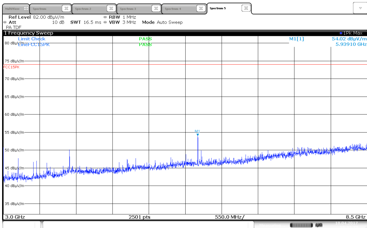
Radiated Emissions, 3000 -8500 MHz, 2437MHz, 802.11b, 1Mbps, Ant1, VP
