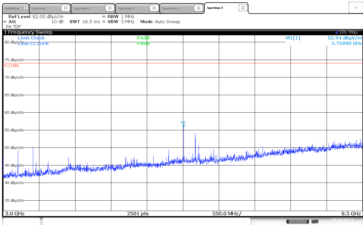
Radiated Emissions, 3000 -8500 MHz, 2437MHz, 802.11b, 1Mbps, Ant0, HP
