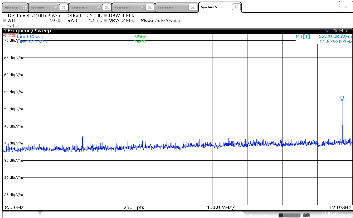
Radiated Emissions, 8000 -12000 MHz, 2437MHz, 802.11n, HT20, MIMO, VP, @1m
