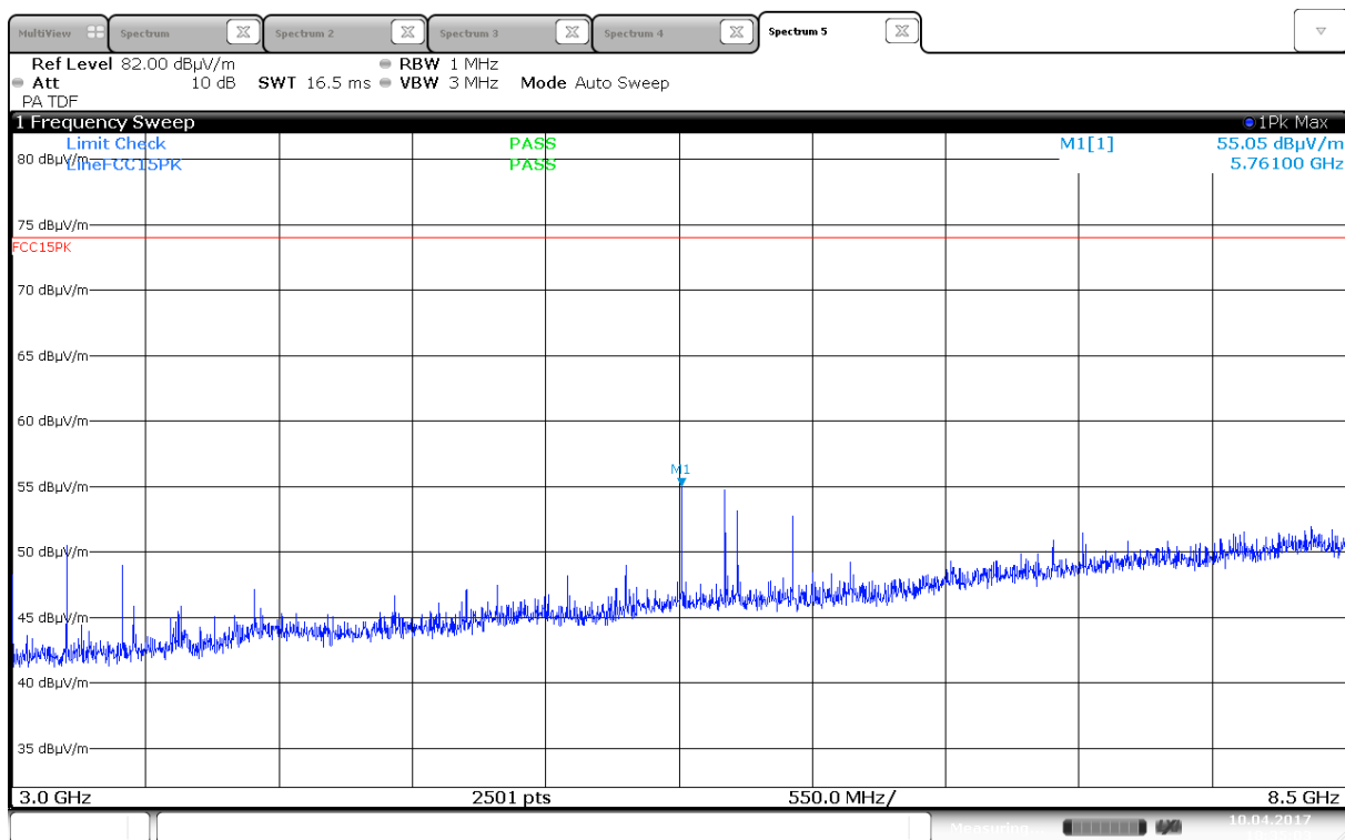
Radiated Emissions, 3000 -8500 MHz, 2437MHz, 802.11b, 1Mbps, Ant1, HP
