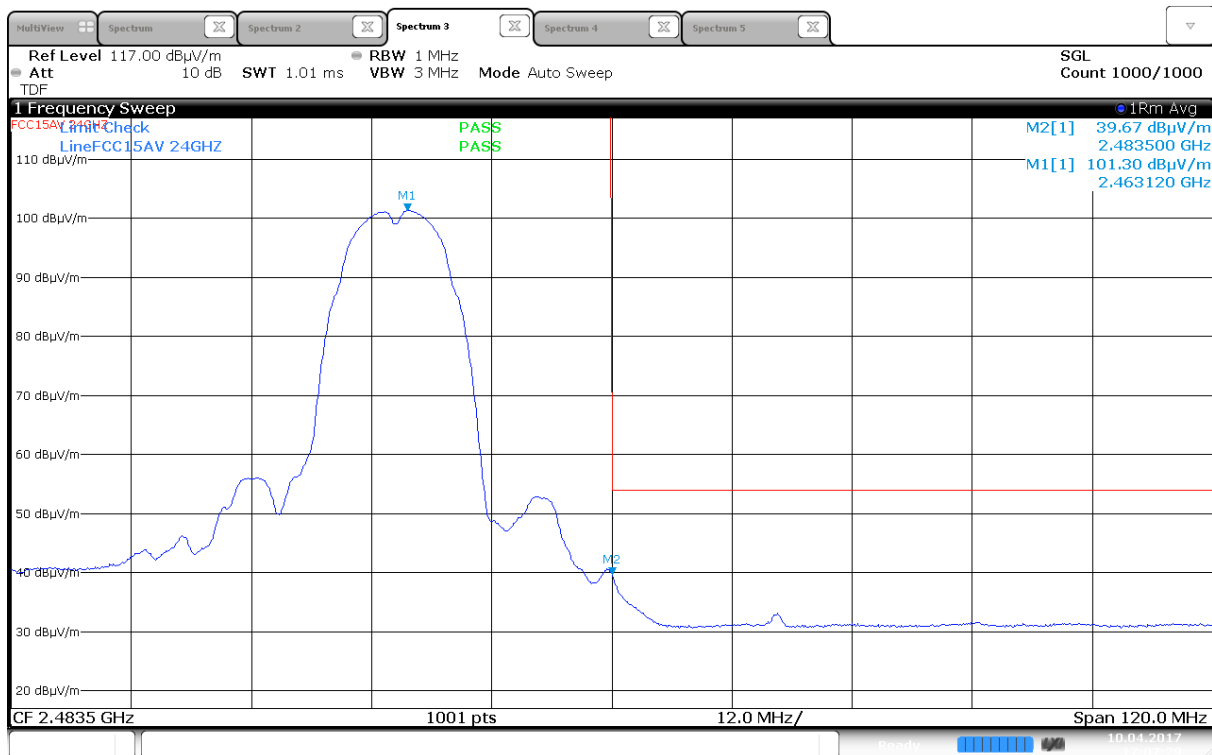
Upper Band Edge, Average, 2462 MHz, 802.11b, 1Mbps, (Max: Ant 0, HP)
