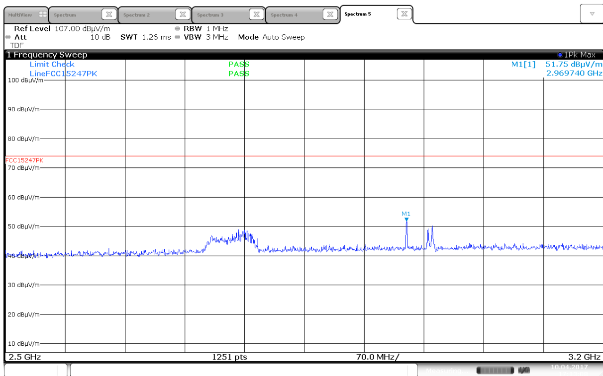
Radiated Emissions, 2500 -3200 MHz, 2462MHz, 802.11b, 1Mbps, Ant0, HP
