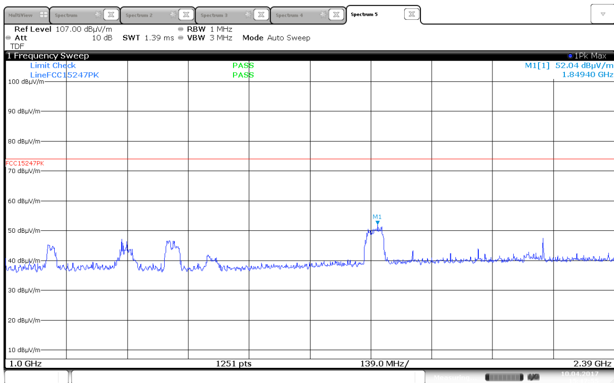
Radiated Emissions, 1000 -2390 MHz, 2412MHz, 802.11b, 1Mb, Ant1, HP
