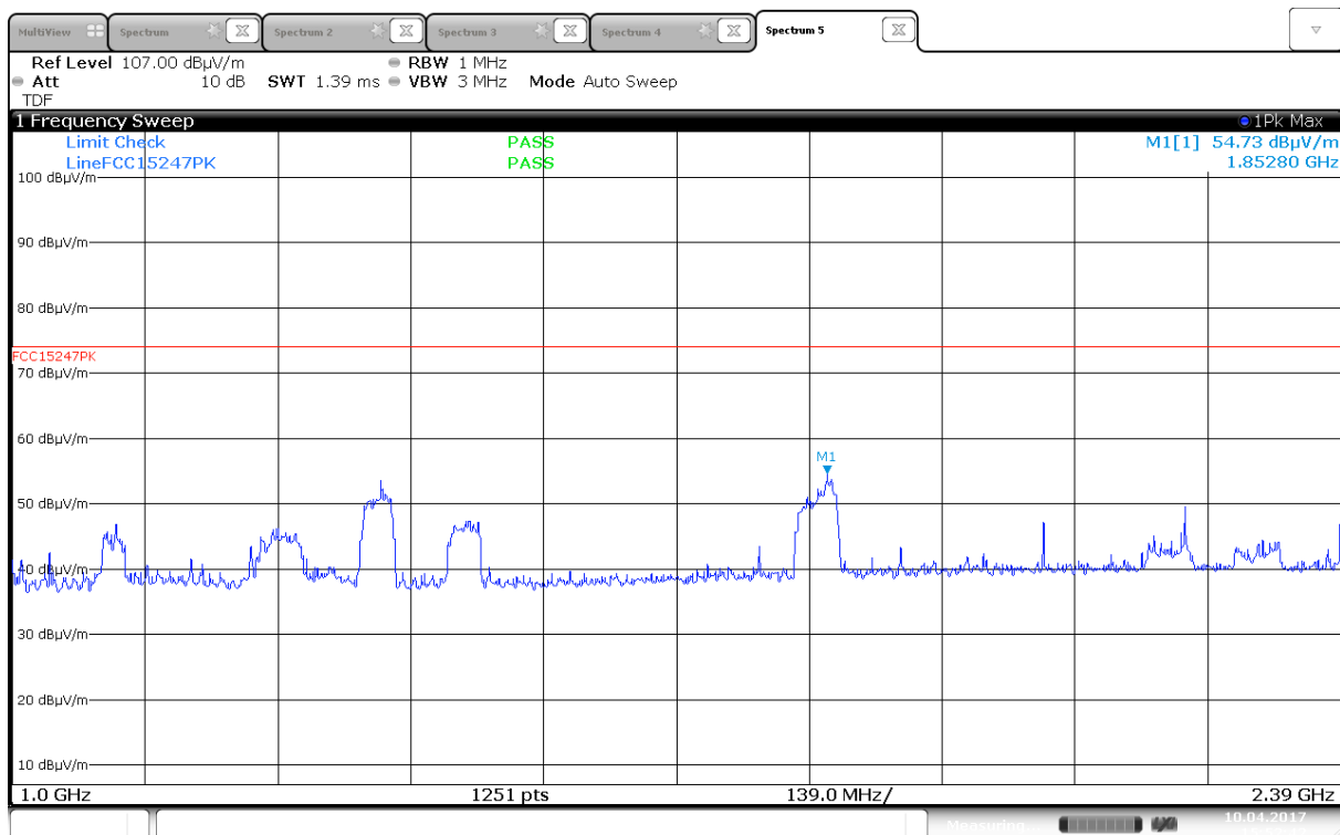
Radiated Emissions, 1000 -2390 MHz, 2412MHz, 802.11g, 6Mb, Ant1, VP
