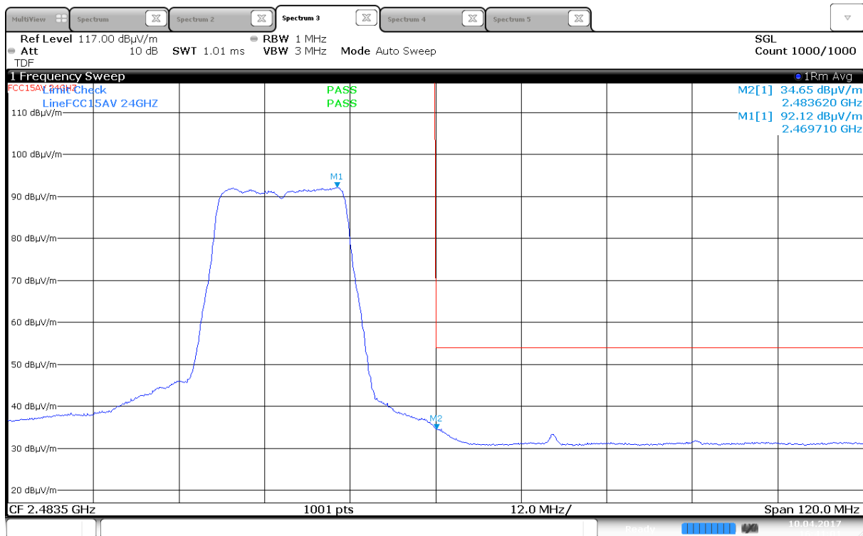
Upper Band Edge, Average, 2462 MHz, 802.11n, MCS0, MIMO (Max: HP)
