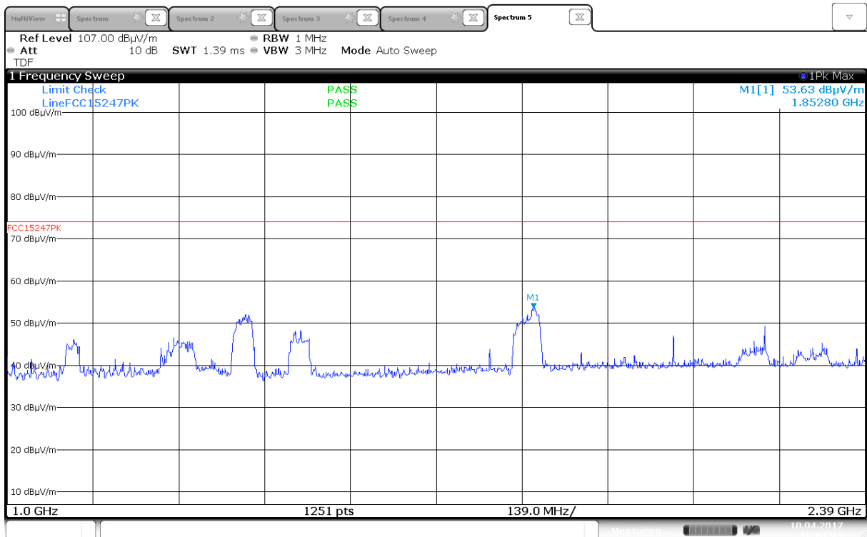
Radiated Emissions, 1000 -2390 MHz, 2412MHz, 802.11b, 1Mb, Ant0, VP
