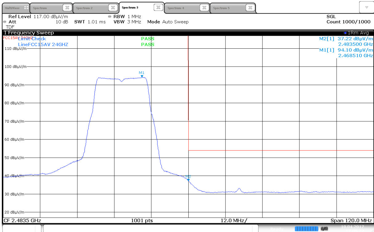
Upper Band Edge, Average, 2462 MHz, 802.11g, 6Mbps, (Max: Ant 0, HP)
