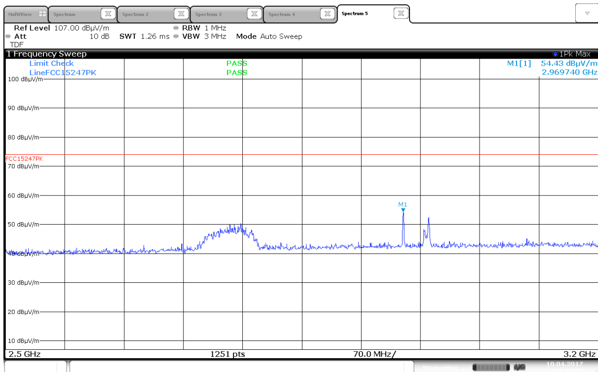
Radiated Emissions, 2500 -3200 MHz, 2462MHz, 802.11b, 1Mbps, Ant0, VP
