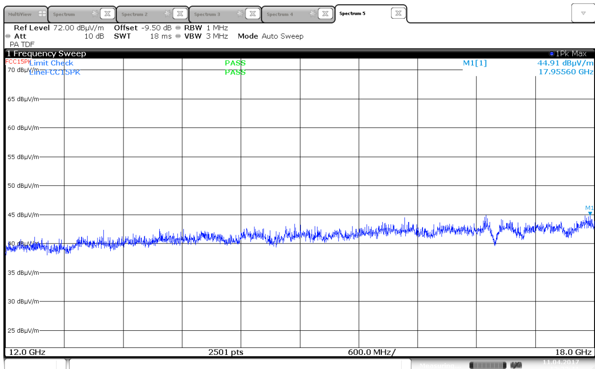
Radiated Emissions, 12000 -18000 MHz, 2437MHz, 802.11n, MCS0, MIMO, VP, @1m
