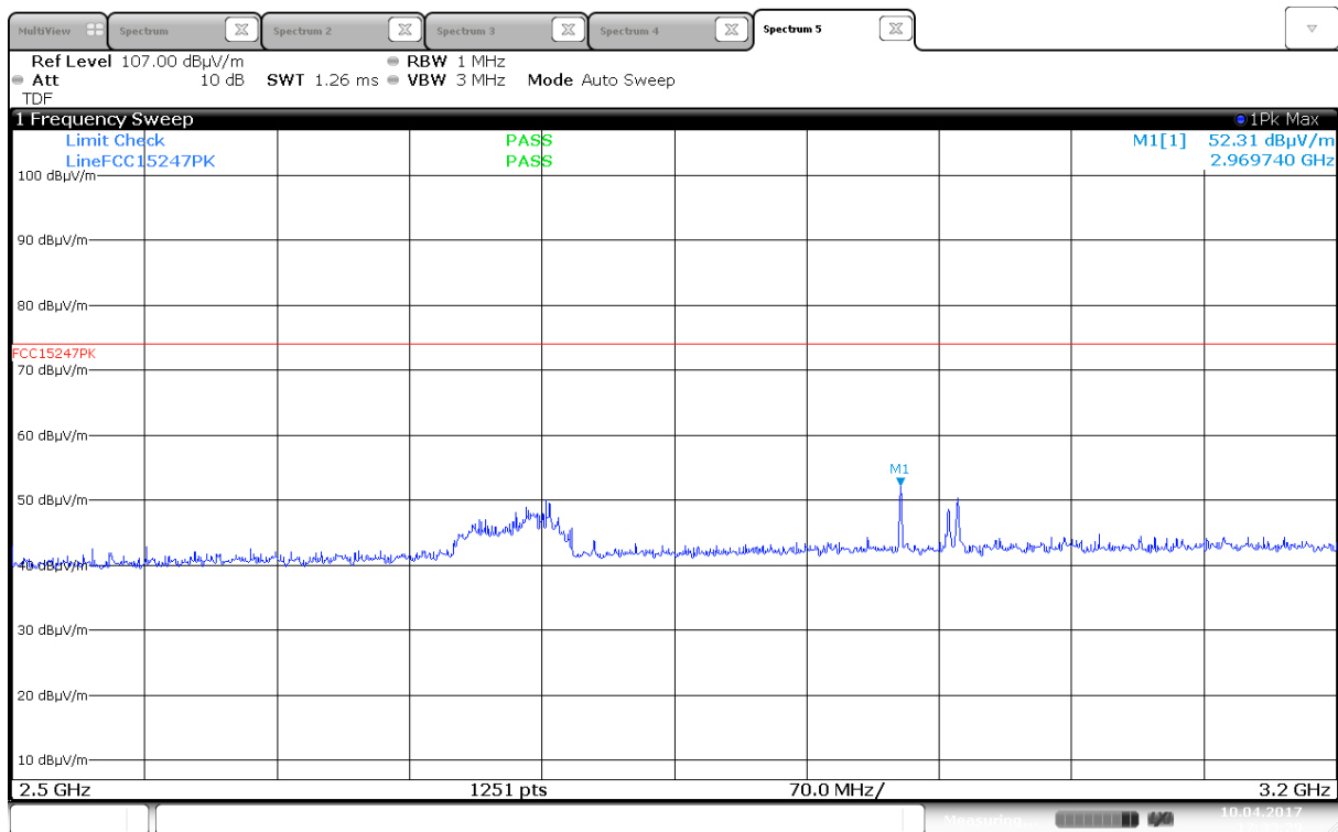
Radiated Emissions, 2500 -3200 MHz, 2462MHz, 802.11n, MCS0, MIMO, HP
