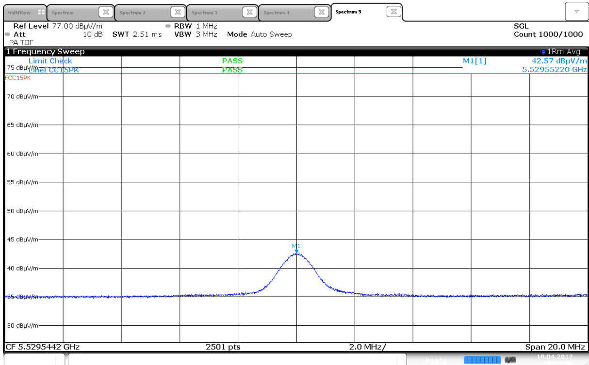
Radiated Emissions Av, 5530MHz, 2437MHz (Max: HP) (Same for all RF-modulations and frequencies)
