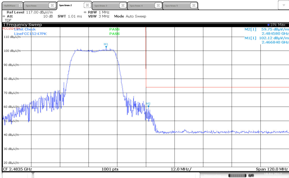
Upper Band Edge, Peak, 2462 MHz, 802.11n, MCS0, MIMO (Max: HP)
