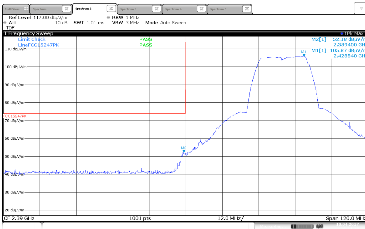
Lower Band Edge, Peak, 2422 MHz, 802.11g, 6Mbps, (Max: Ant 0, HP)
