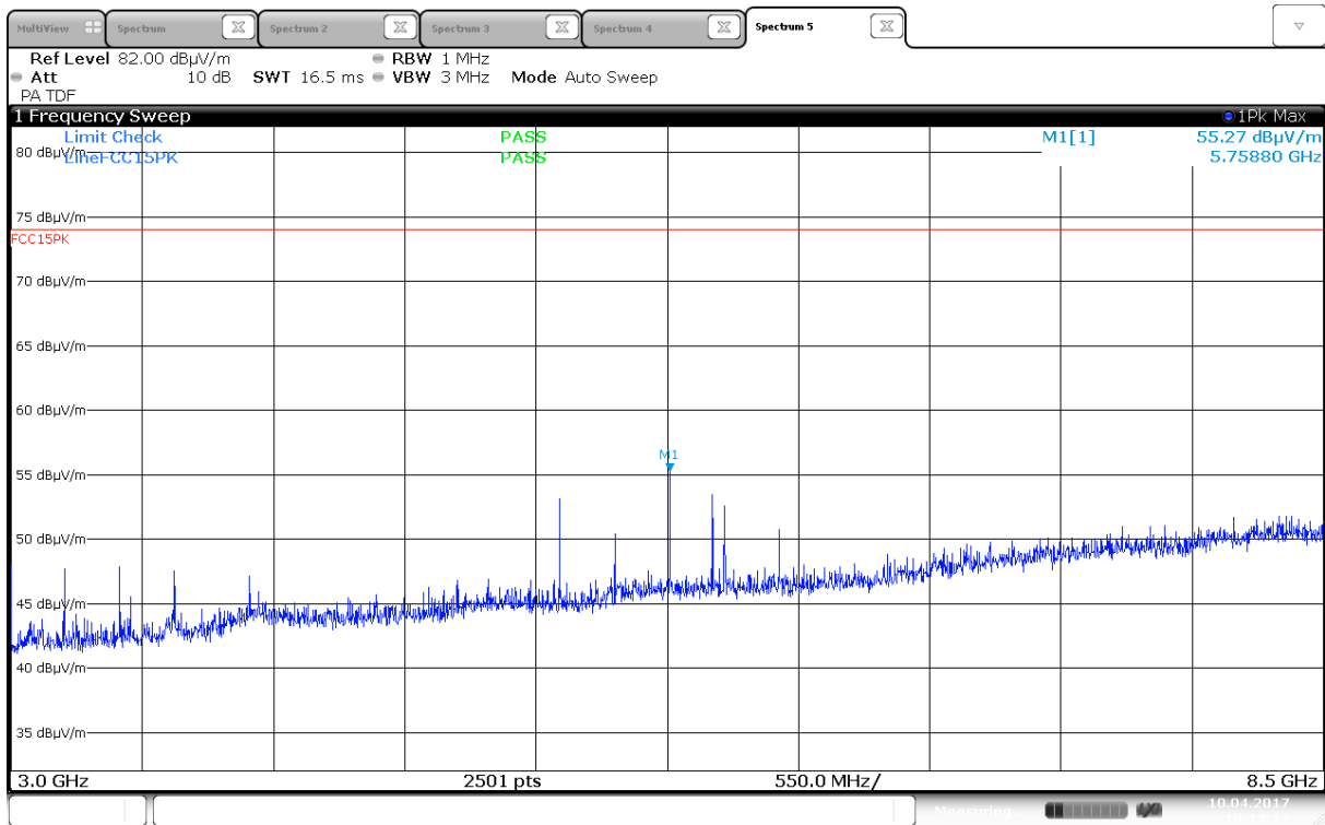
Radiated Emissions, 3000 -8500 MHz, 2437MHz, 802.11n, HT20, MIMO, HP
