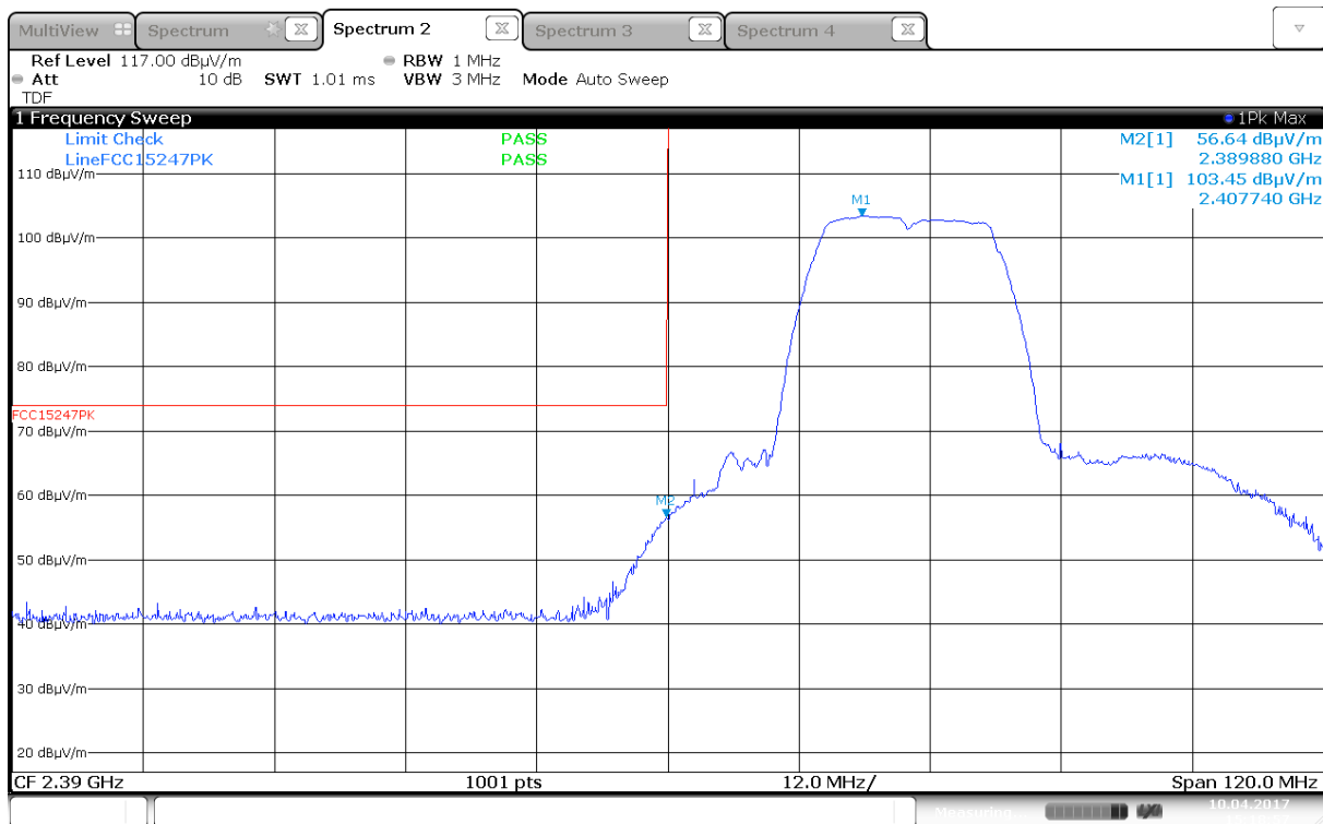
Lower Band Edge, Peak, 2412 MHz, 802.11g, 6Mbps, (Max: Ant 0, HP)
