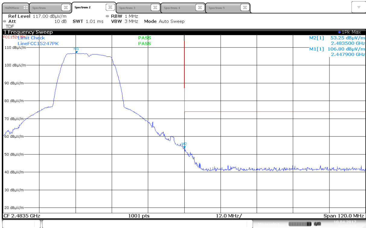
Upper Band Edge, Peak, 2452 MHz, 802.11g, 6Mbps, (Max: Ant 0, HP)
