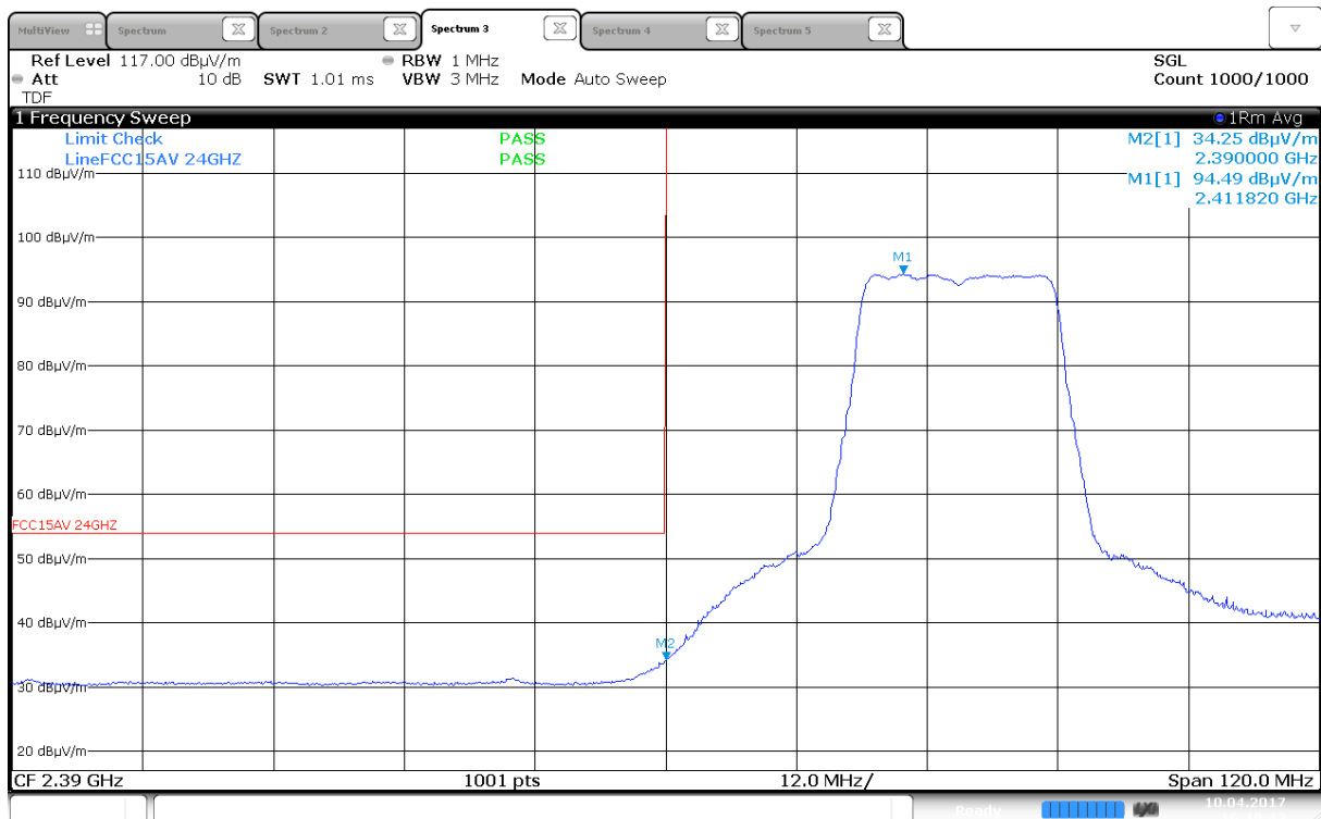
Lower Band Edge, Average, 2417 MHz, 802.11n, MCS0, MIMO (Max: HP)
