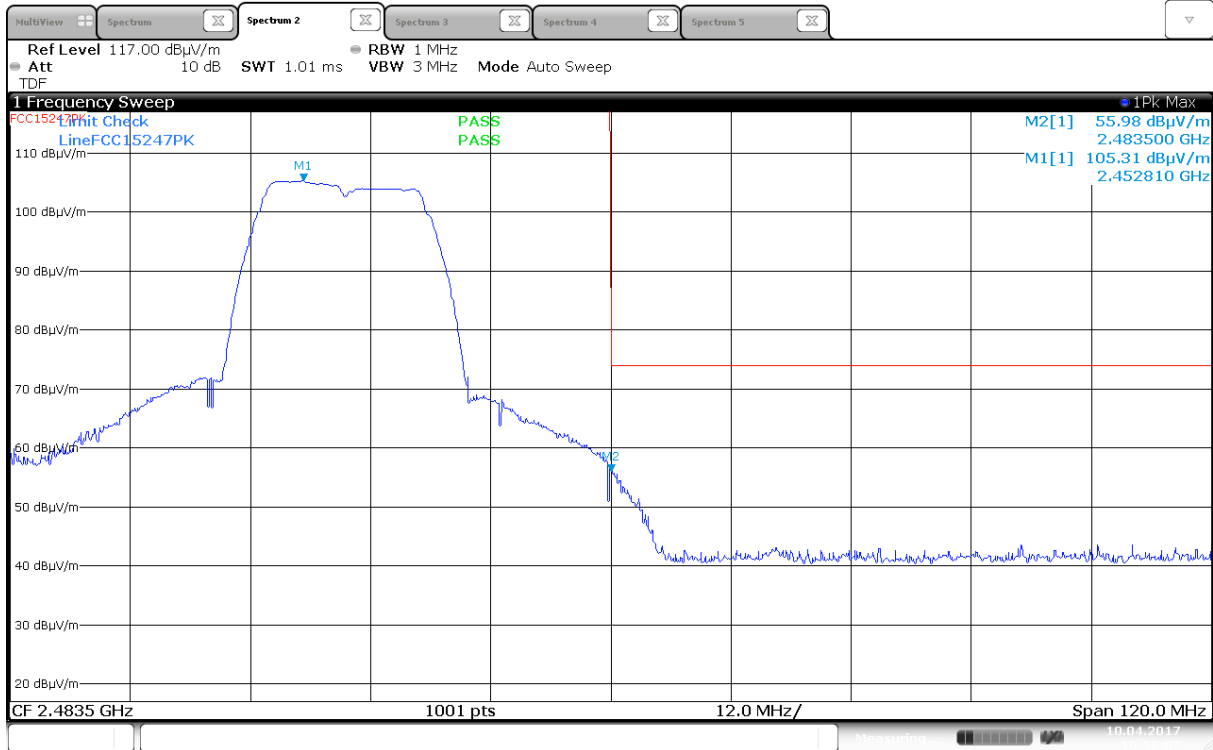
Upper Band Edge, Peak, 2457 MHz, 802.11g, 6Mbps, (Max: Ant 0, HP)
