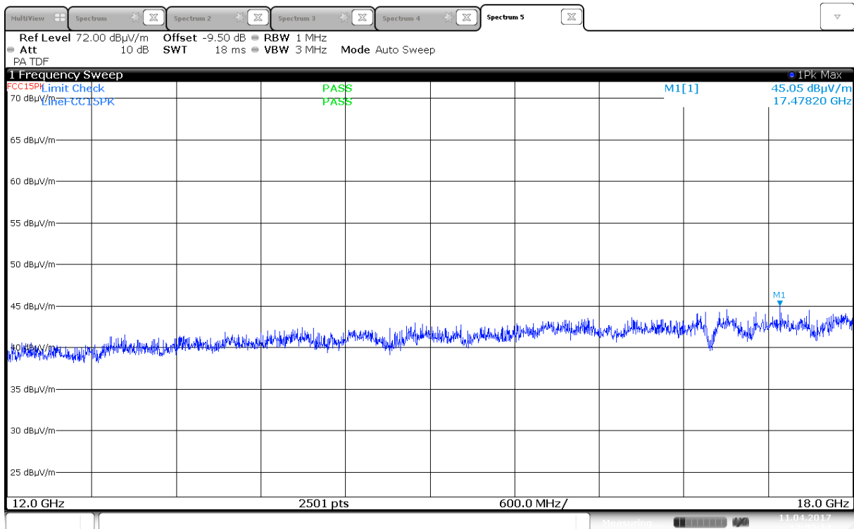
Radiated Emissions, 12000 -18000 MHz, 2437MHz, 802.11b, 1Mbps, Ant1, VP, @1m
