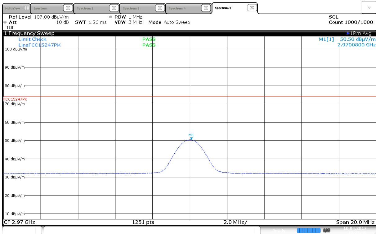
Radiated Emissions Av, 2970MHz, 2462MHz (Max: HP) (Same for all RF-modulations and frequencies)
