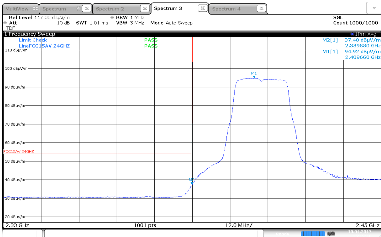
Lower Band Edge, Average, 2412 MHz, 802.11g, 6Mbps, (Max: Ant 0, HP)
