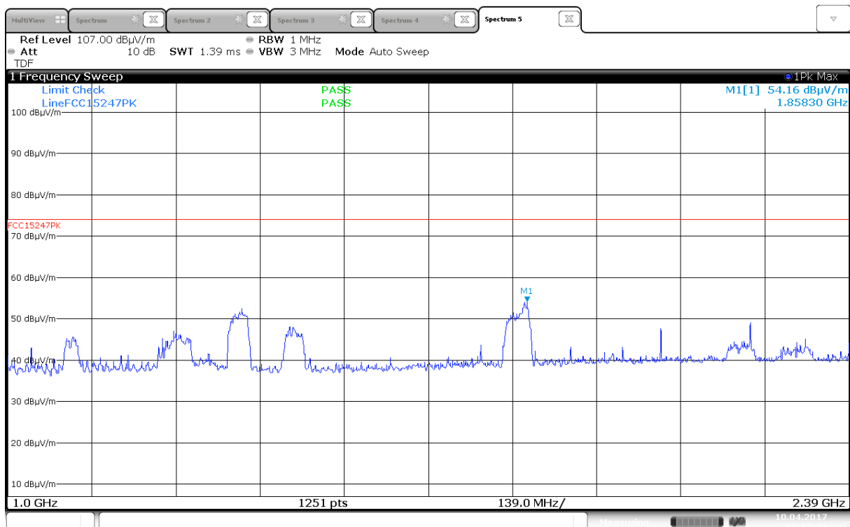
Radiated Emissions, 1000 -2390 MHz, 2412MHz, 802.11g, 6Mb, Ant0, VP
