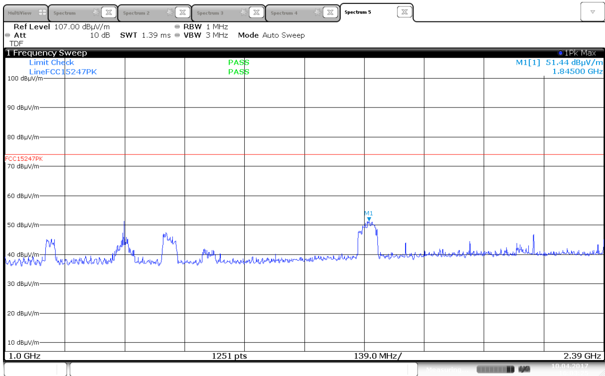
Radiated Emissions, 1000 -2390 MHz, 2412MHz, 802.11b, 1Mb, Ant0, HP
