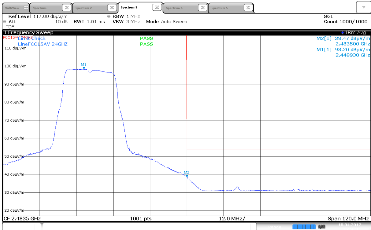
Upper Band Edge, Average, 2452 MHz, 802.11g, 6Mbps, (Max: Ant 0, HP)
