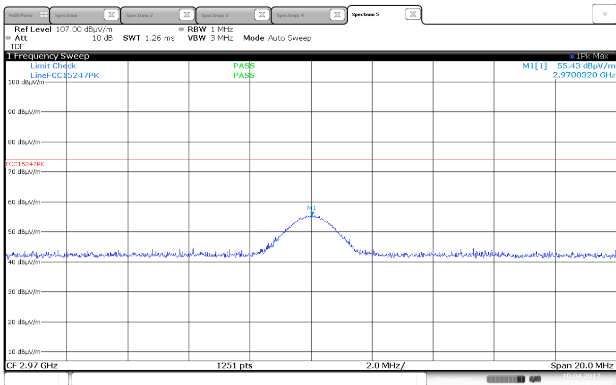
Radiated Emissions Pk, 2970MHz, 2462MHz (Max: HP) (Same for all RF-modulations and frequencies)
