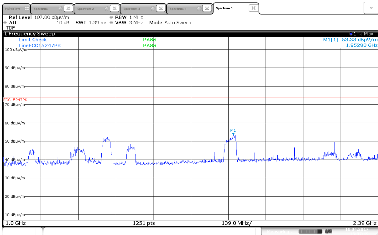
Radiated Emissions, 1000 -2390 MHz, 2412MHz, 802.11n, MCS0, MIMO, VP
