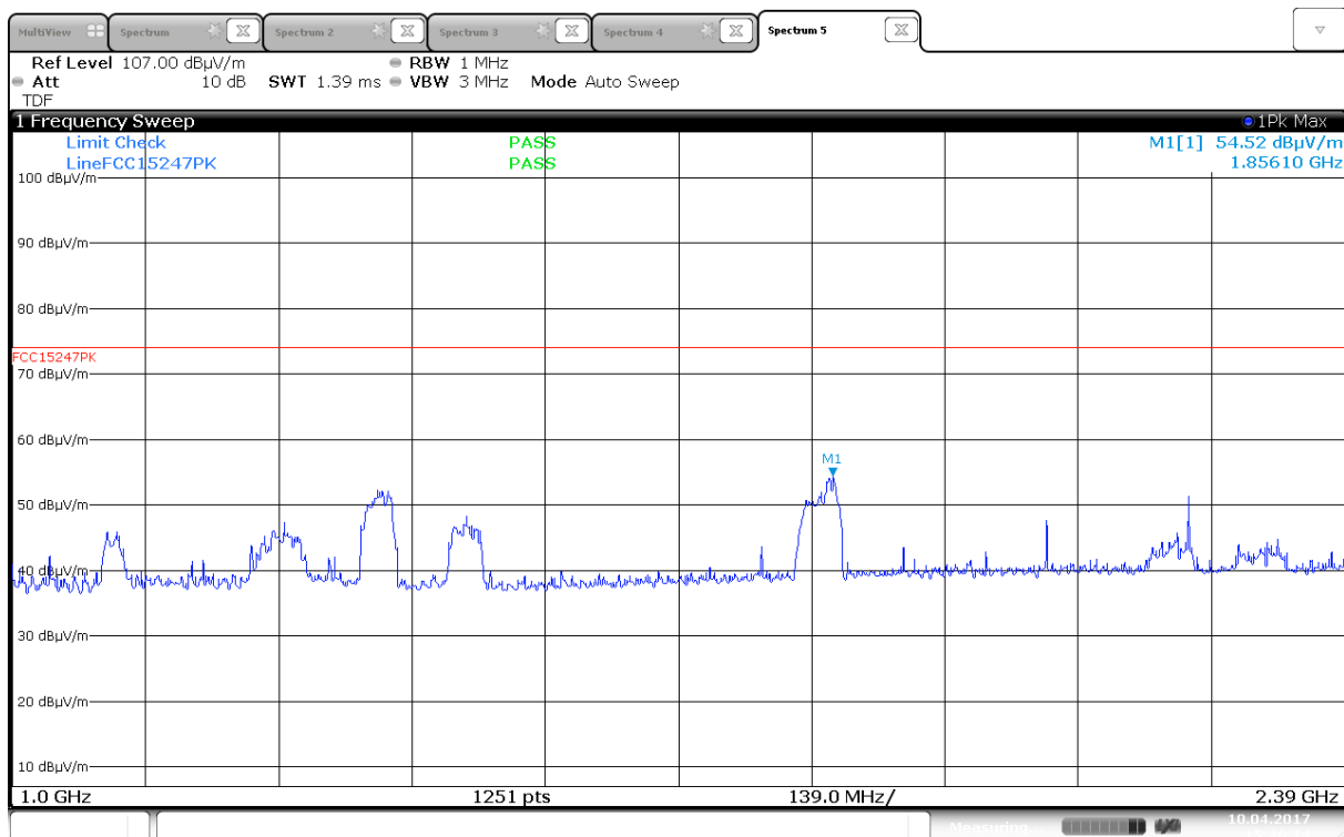
Radiated Emissions, 1000 -2390 MHz, 2412MHz, 802.11b, 1Mb, Ant1, VP
