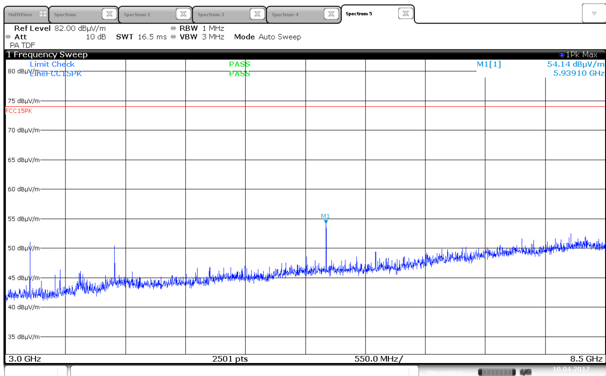
Radiated Emissions, 3000 -8500 MHz, 2437MHz, 802.11b, 1Mbps, Ant0, VP
