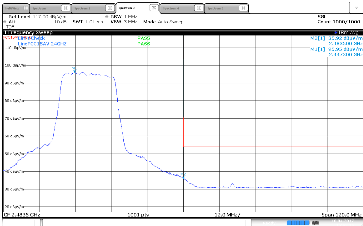
Upper Band Edge, Average, 2452 MHz, 802.11n, MCS0, MIMO (Max: HP)
