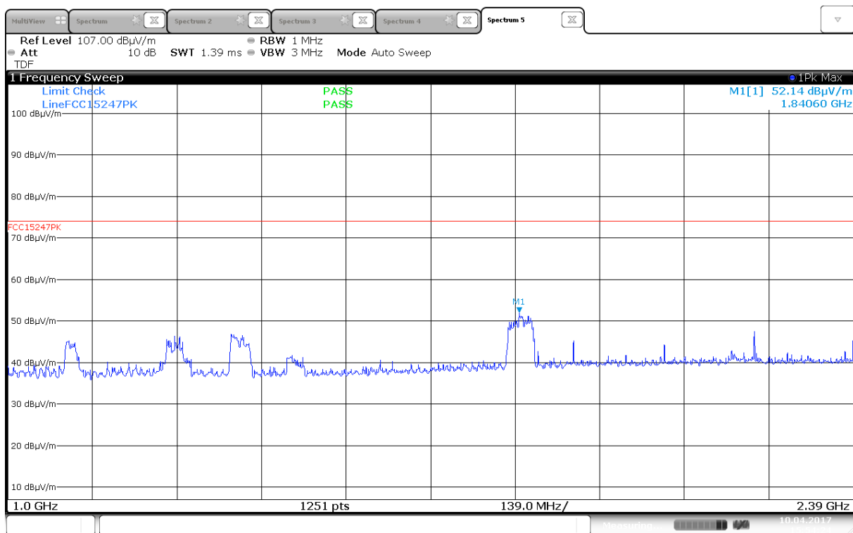
Radiated Emissions, 1000 -2390 MHz, 2412MHz, 802.11g, 6Mb, Ant1, HP
