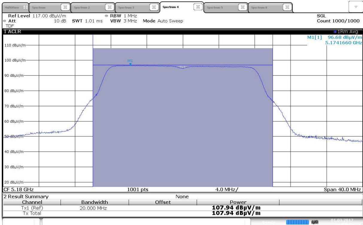
Maximum EIRP, 5180 MHz, 802.11a 6Mbps, Ant 1
