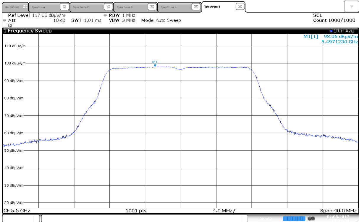
Power Spectral Density, 5500 MHz, 802.11a 6Mbps, Ant 0
