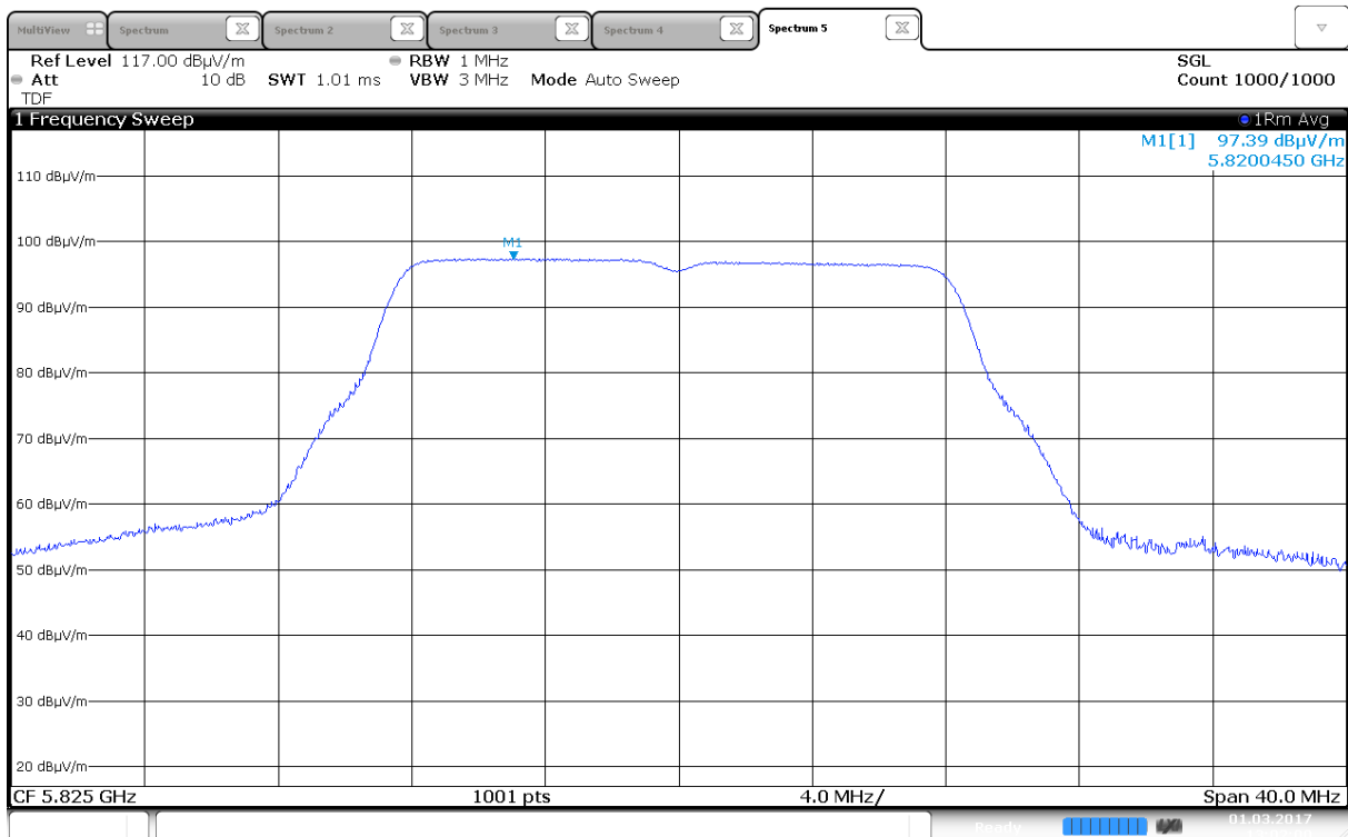
Power Spectral Density, 5825 MHz, 802.11a 6Mbps, Ant 1
