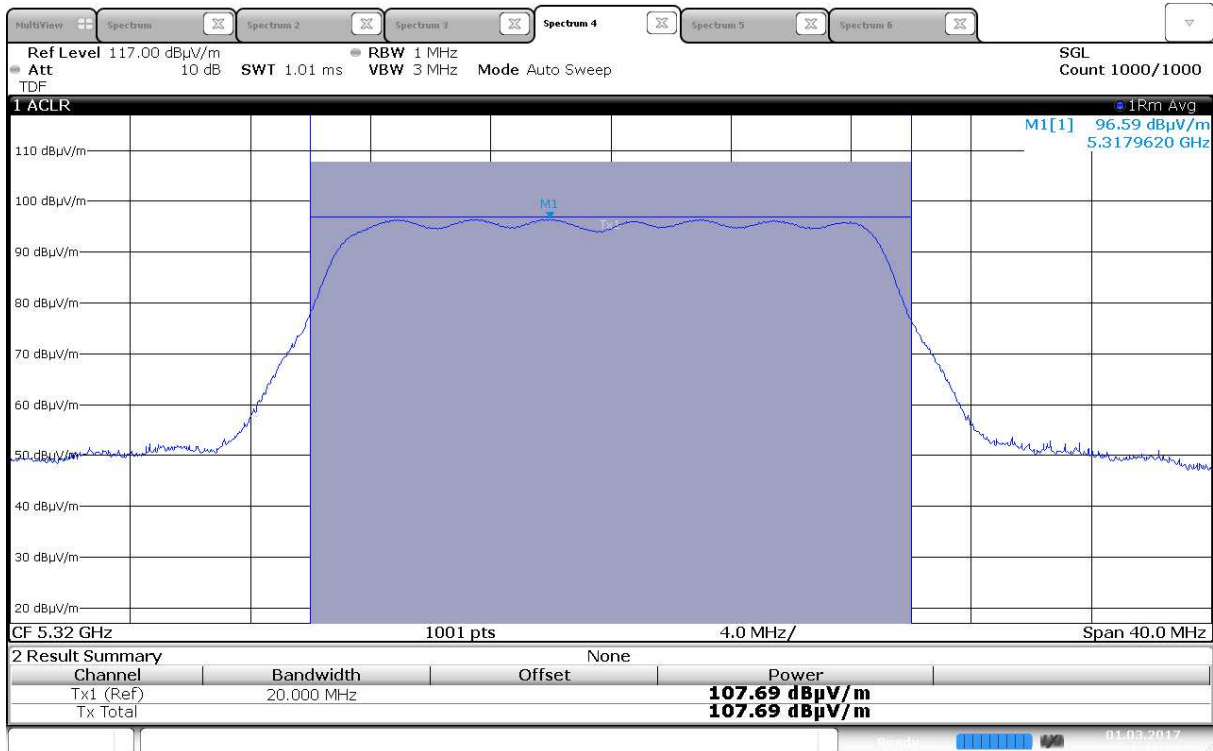
Maximum EIRP, 5320 MHz, 802.11n HT20, MIMO
