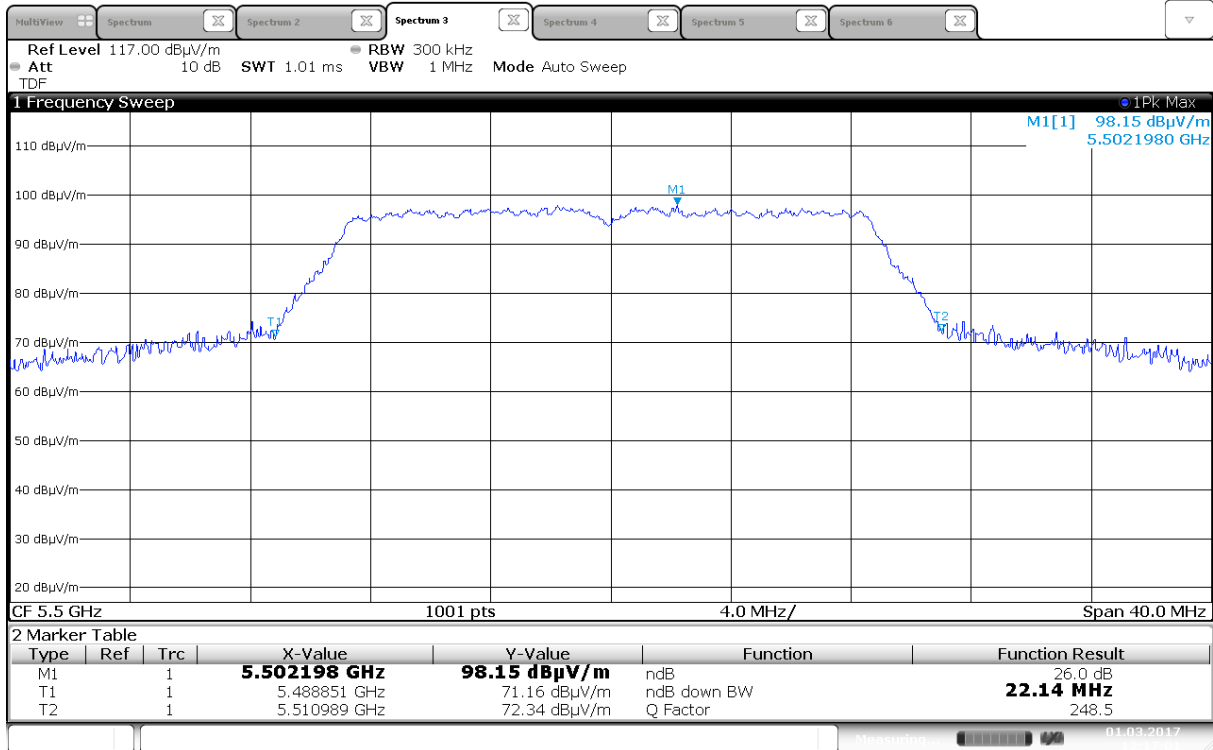
Emission Bandwidth B, 5500 MHz, 802.11n HT20, MIMO
