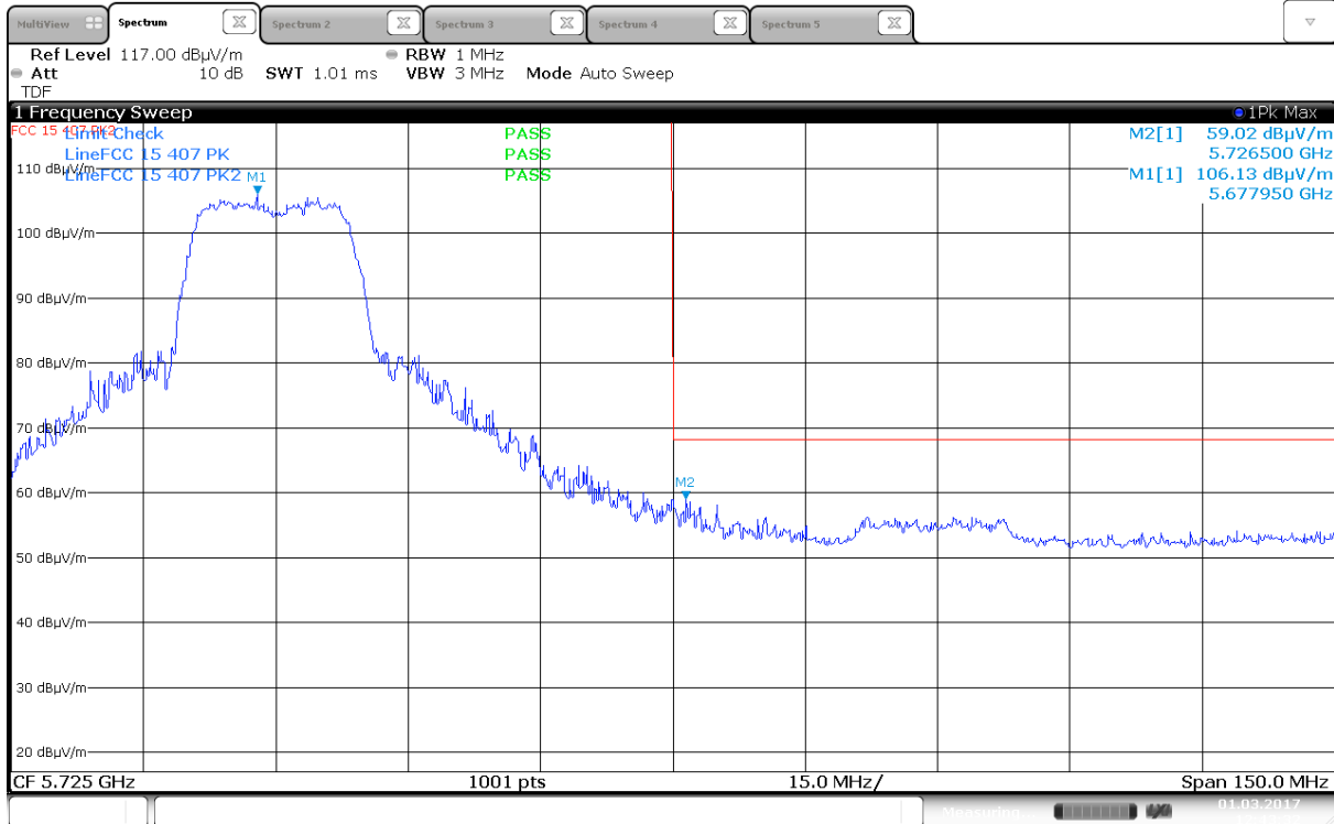
Unwanted Emissions, Band Edge, 5725MHz, ch136, 802.11n MCS0 HT20, MIMO
