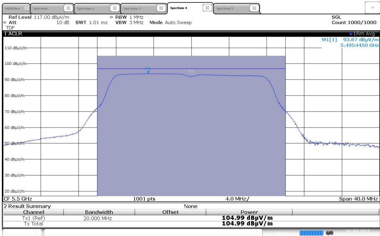
Maximum EIRP, 5500 MHz, 802.11a 6Mbps, Ant 1
