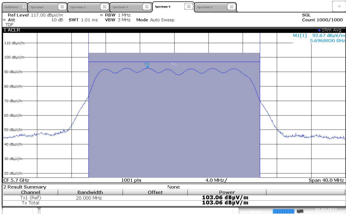
Maximum EIRP, 5700 MHz, 802.11n HT20, MIMO
