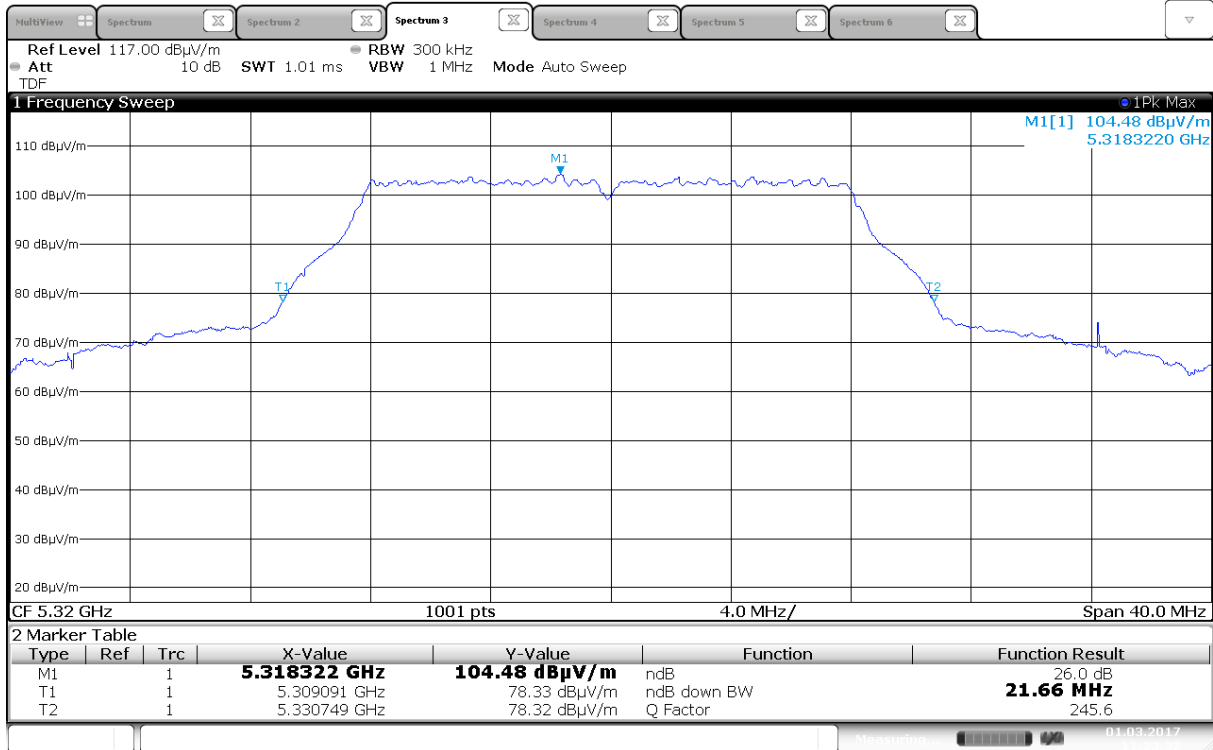
Emission Bandwidth B, 5320 MHz, 802.11a 6Mbps, Ant 0
