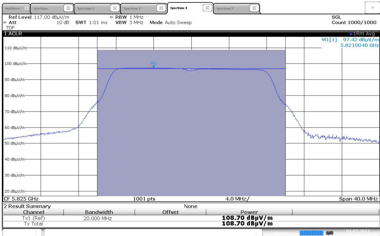
Maximum EIRP, 5825 MHz, 802.11a 6Mbps, Ant 1
