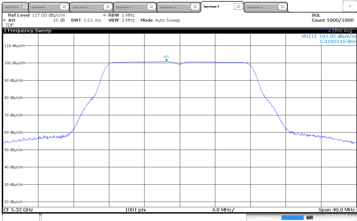
Power Spectral Density, 5320 MHz, 802.11a 6Mbps, Ant 0
