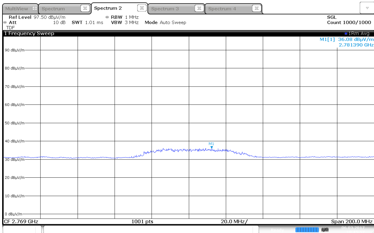
Radiated Emissions Av, 2777MHz, 2442MHz (Max: HP) (Same for all RF-modulations and frequencies)
