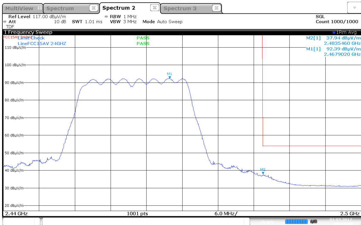
Upper Band Edge, Average, 2462 MHz, 802.11n, MCS0, (Max: Ant 0, HP)
