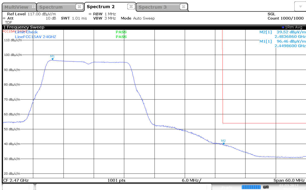
Upper Band Edge, Average, 2457 MHz, 802.11g, 6Mbps, (Max: Ant 0, HP)
