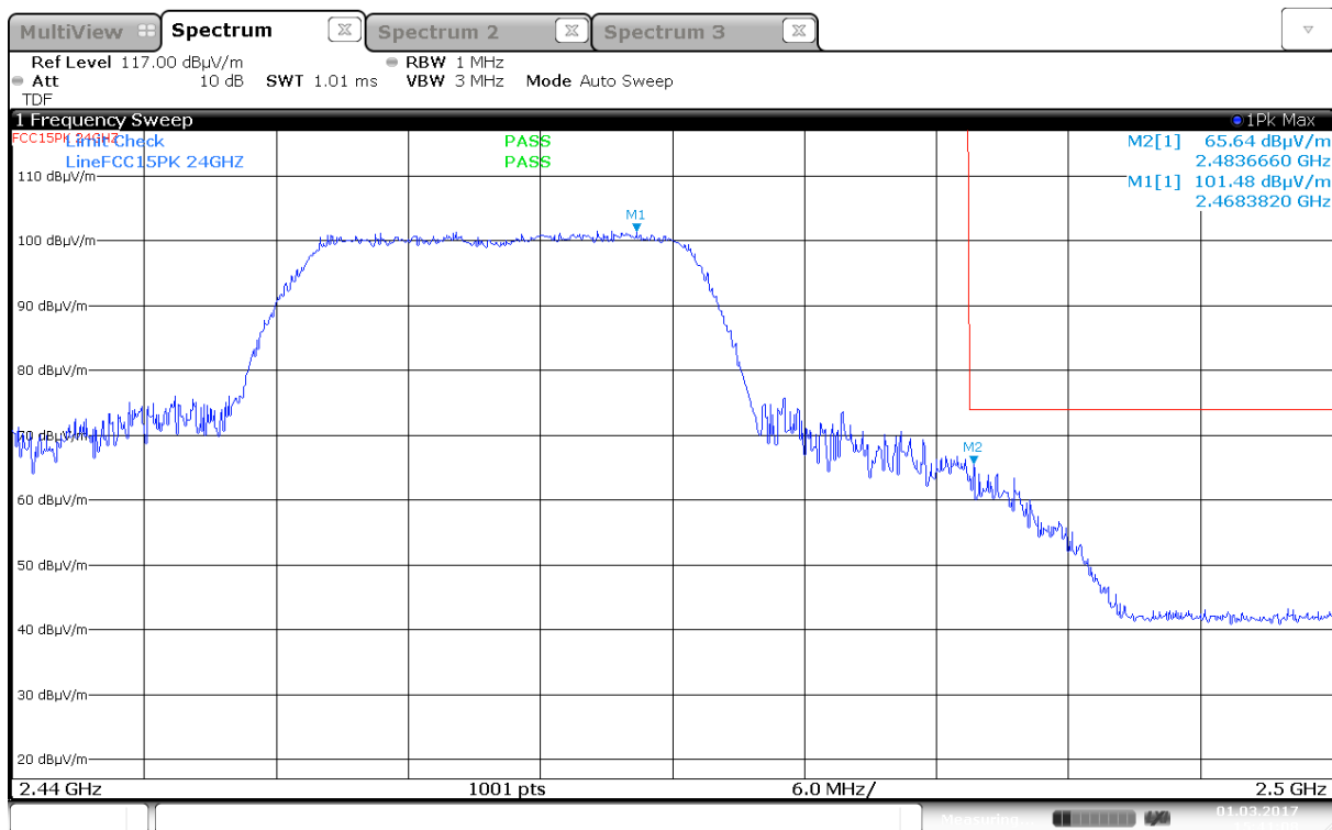
Upper Band Edge, Peak, 2462 MHz, 802.11n, MCS0, (Max: Ant 0, HP)
