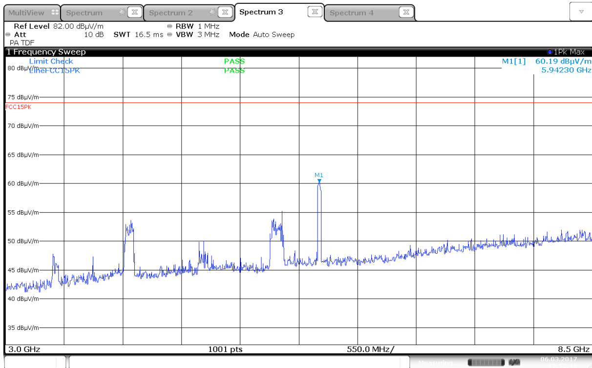
Radiated Emissions, 3000 -8500 MHz, 2442MHz, VP, 802.11g, 6Mbps, Ant0
