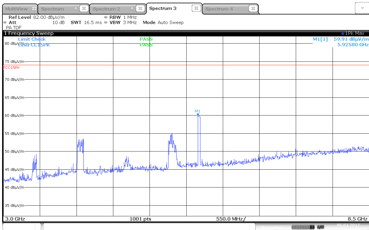
Radiated Emissions, 3000 -8500 MHz, 2442MHz, VP, 802.11b, 6Mbps, Ant0
