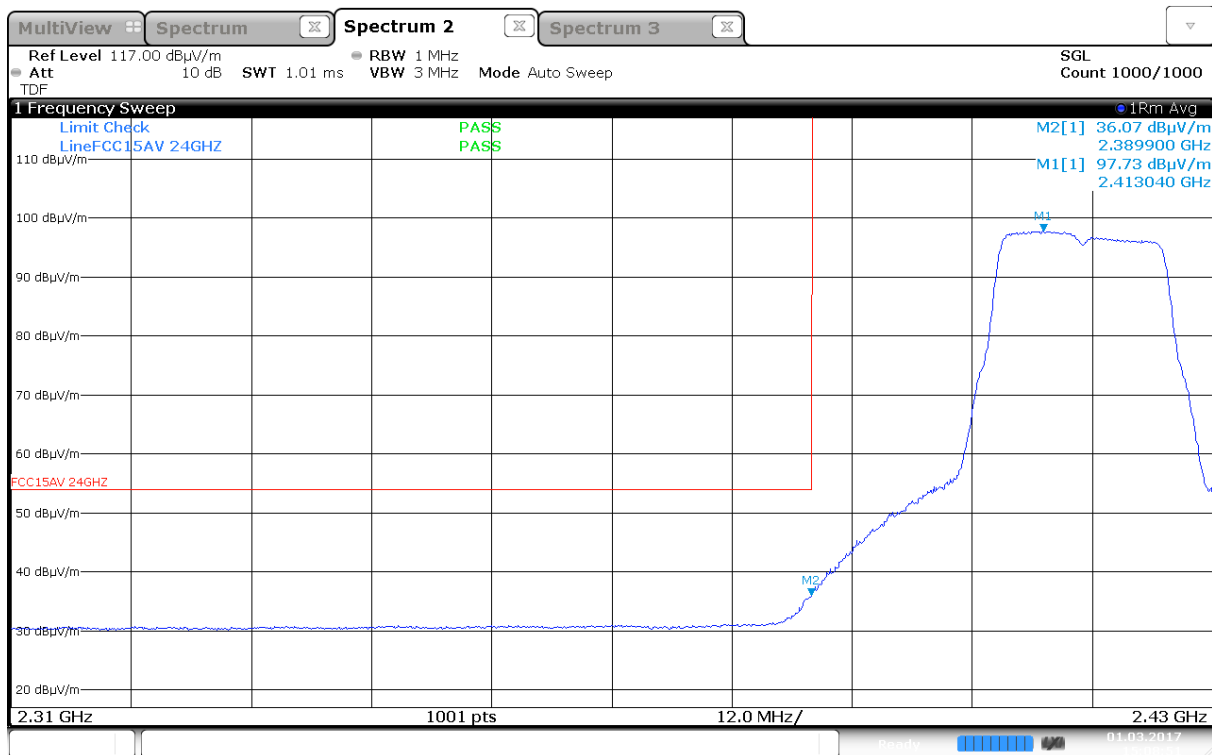
Lower Band Edge, Average, 2417 MHz, 802.11g, 6Mbps, (Max: Ant 0, HP)
