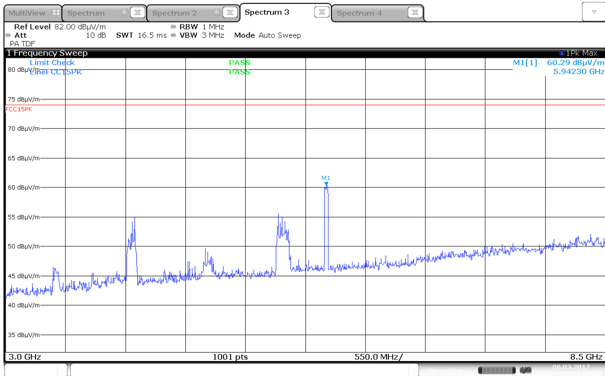
Radiated Emissions, 3000 -8500 MHz, 2442MHz, VP, 802.11n, MCS0, MIMO
