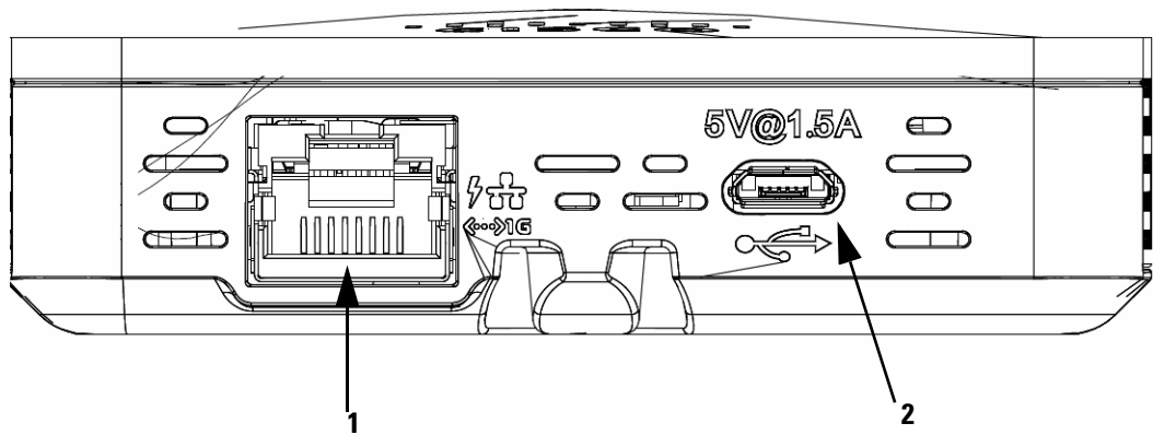
Figure 2 Power-over-Ethernet and USB Ports on the Base
