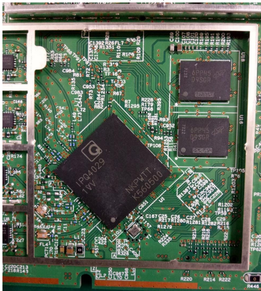
Close-up RF chip
