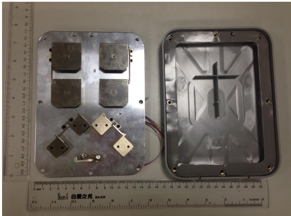
1542D antenna
