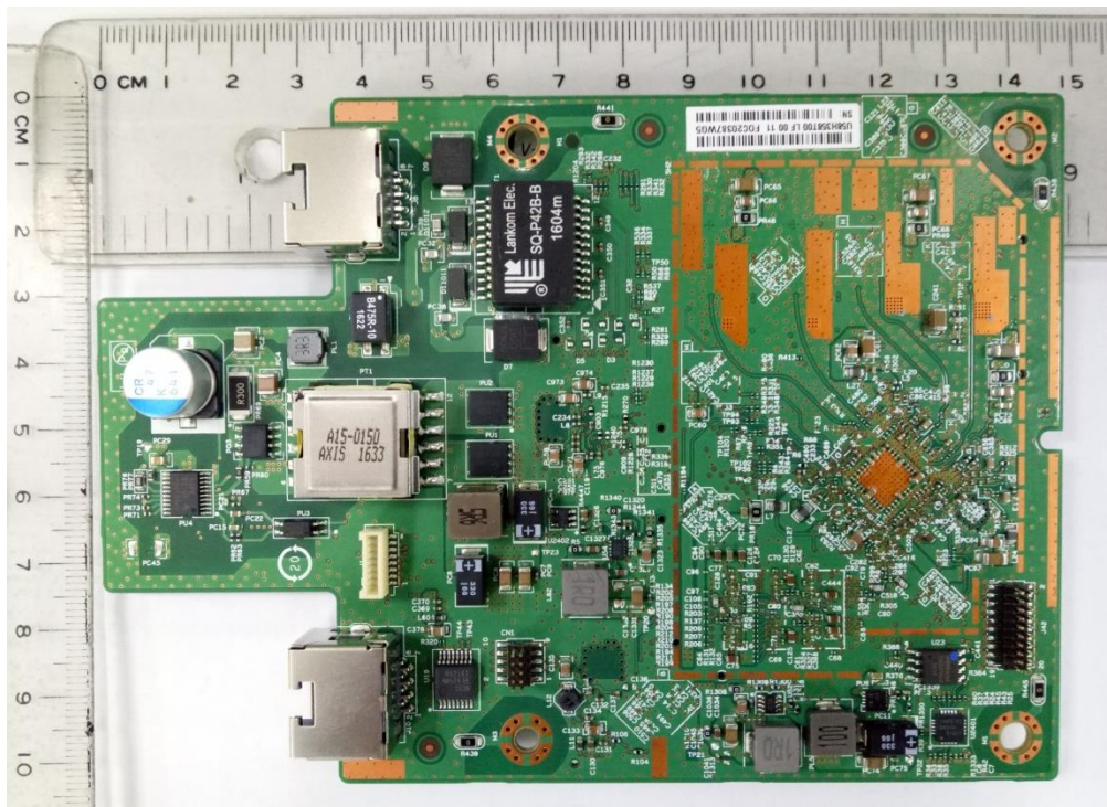
Bottom Side RF Board
