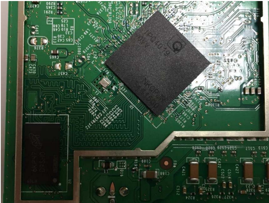
Close-up RF chip (Main Chip – CPU – QCA, IPQ4019)
