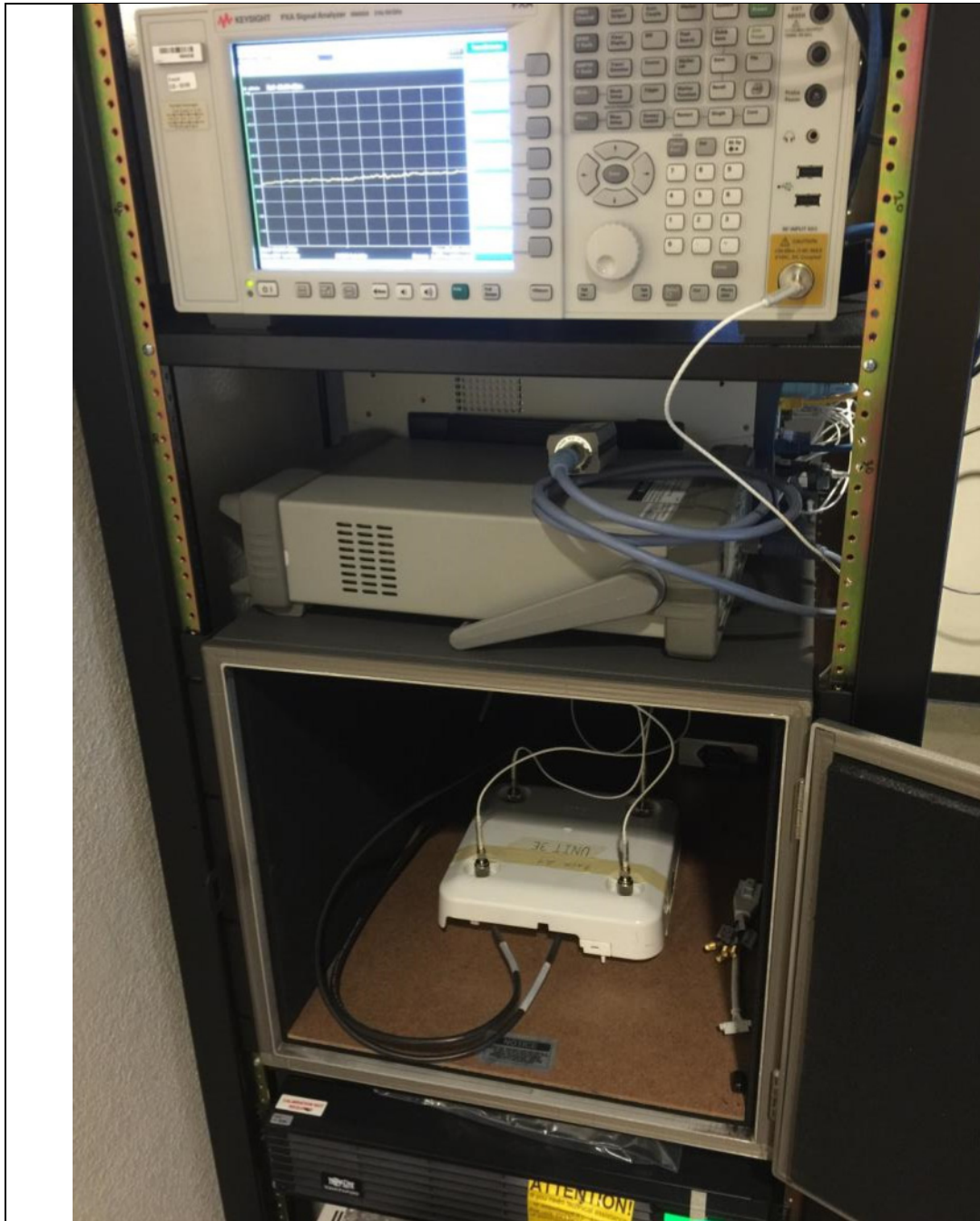
Title: Conducted Test Setup
