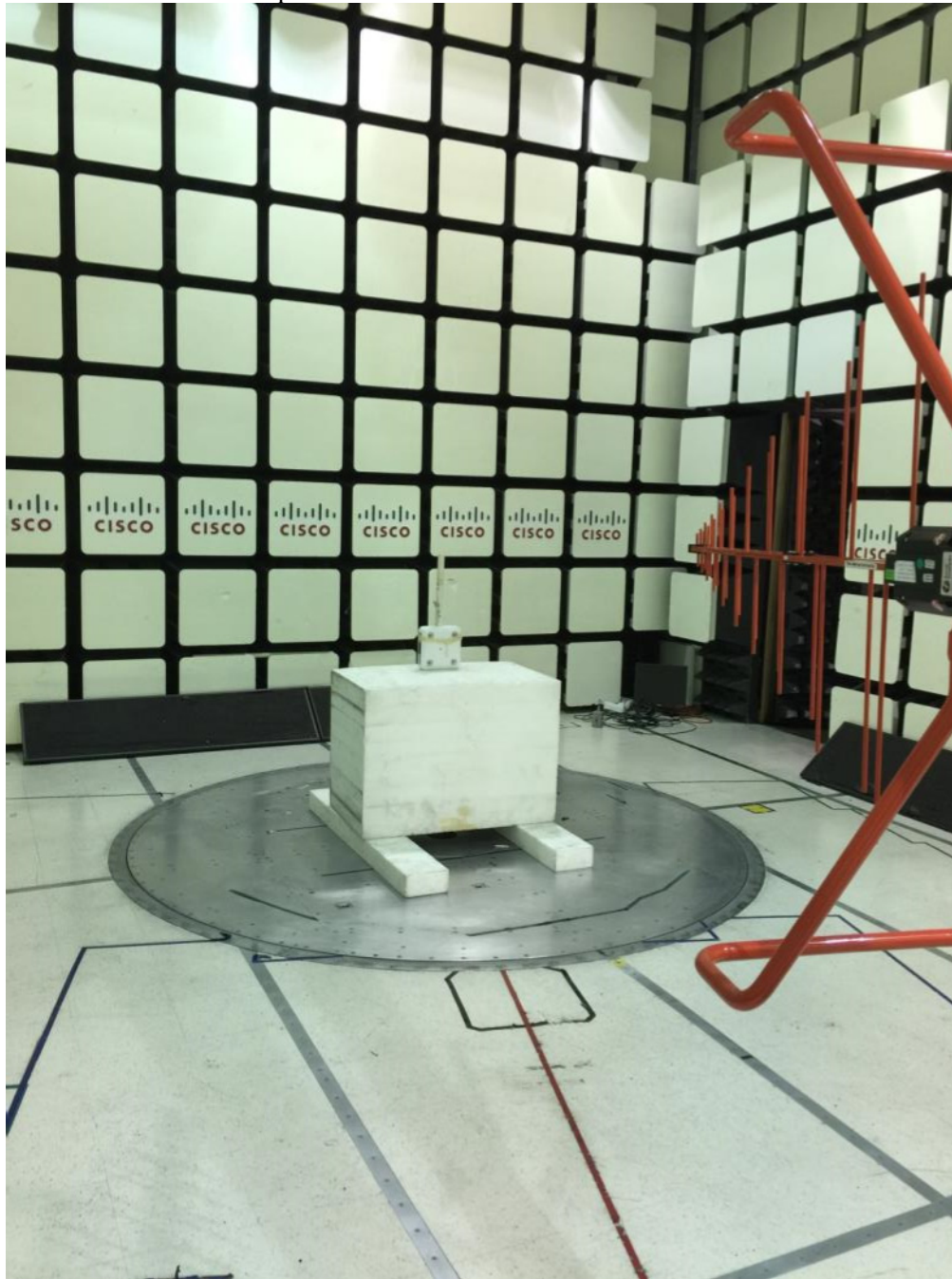
Radiated Emissions setup 30MHz – 1GHz
