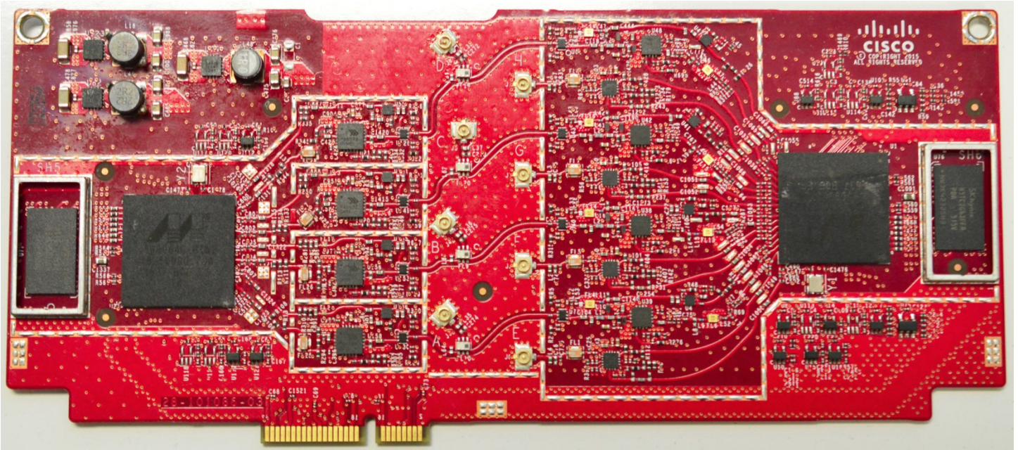
Top Side RF Board without Shields
