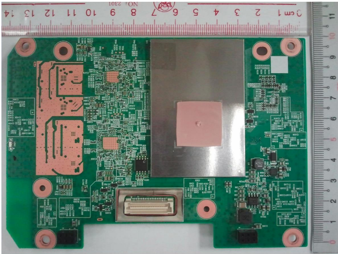
Bottom Side RF Board without Shields
