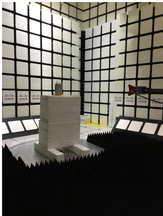
AIR-AP1572EAC-B-K9 Radiated Emissions setup above 1GHz
