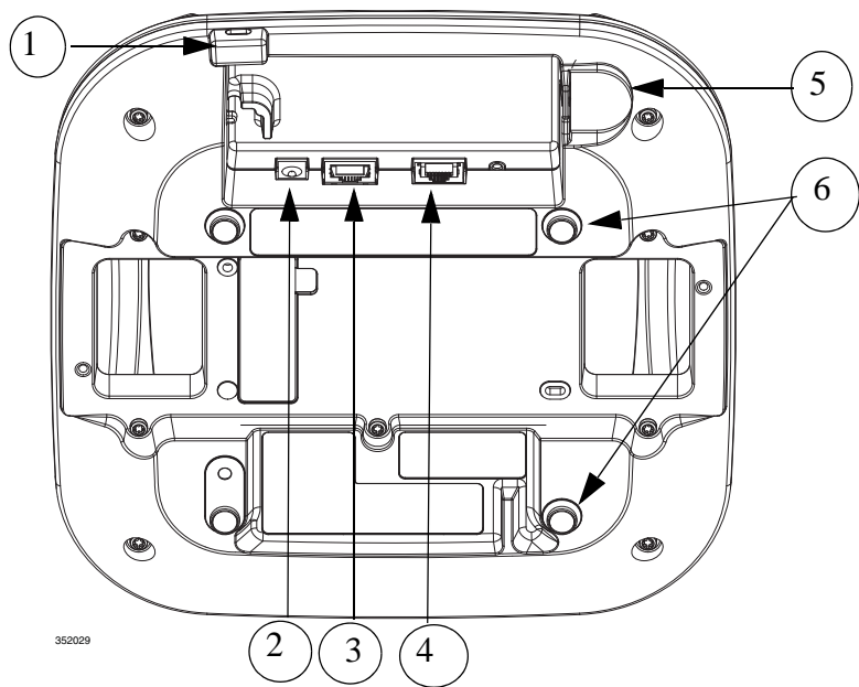
Figure 2 Access Point Ports and Connections (bottom)-AIR3702P
