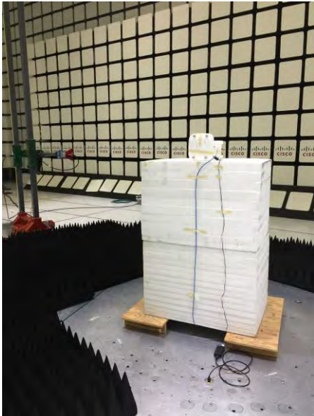
AIR-CAP2602E-B-K9 Radiated Test setup photo above 1GHz
