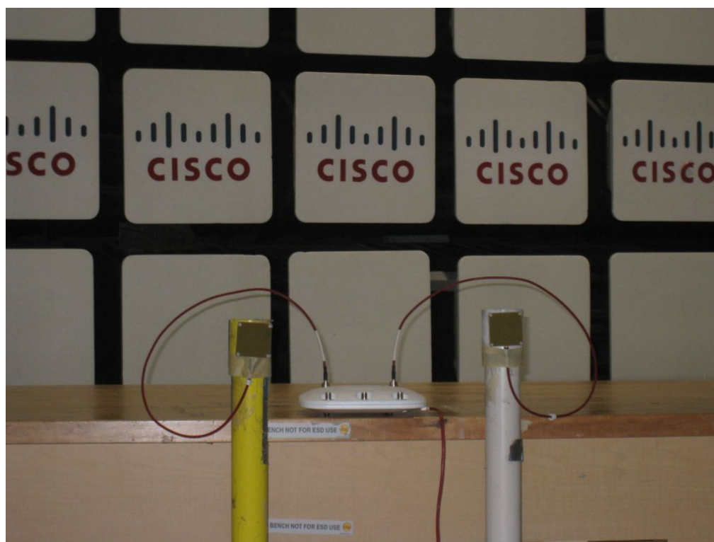
5GHz 7dBi Patch antenna
