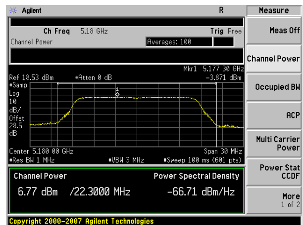
Antenna B
