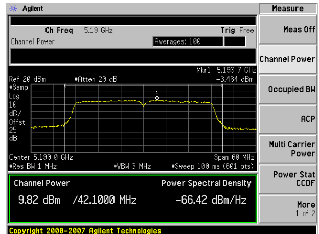
Antenna B
