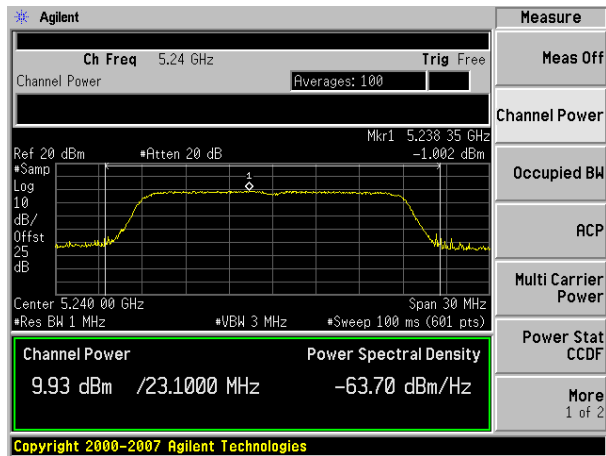
Antenna B
