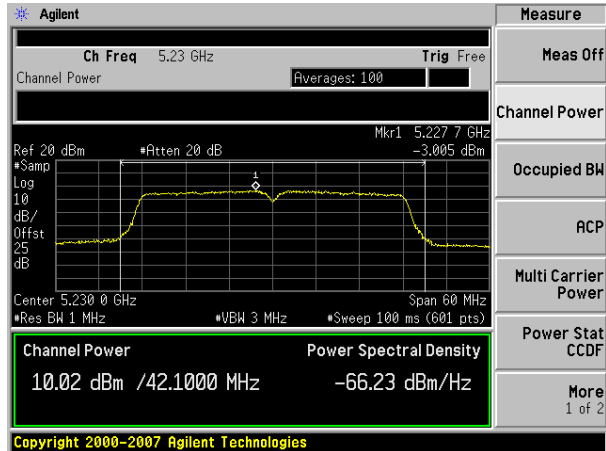
Antenna B
