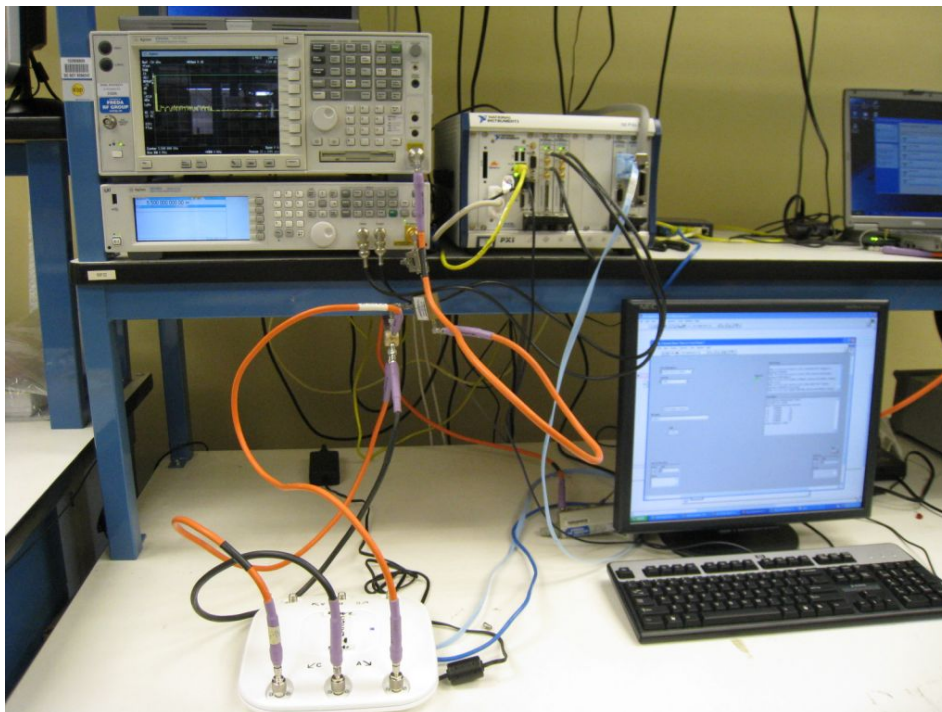
DFS Setup
