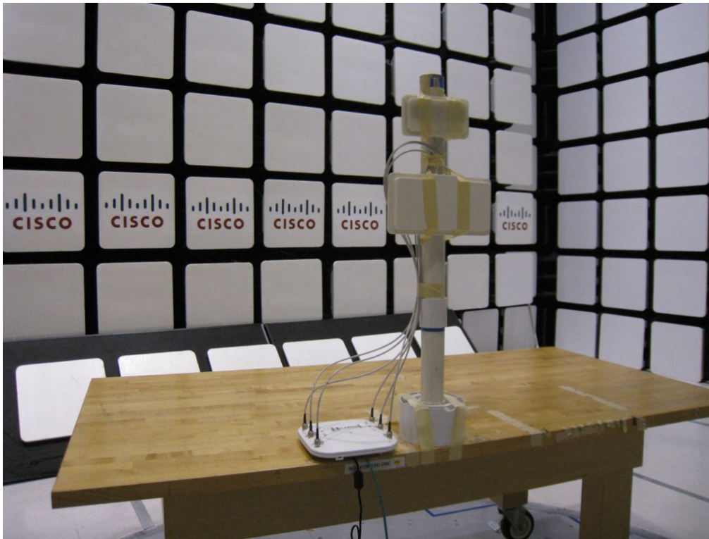
2.4GHz 6dBi MIMO patch co-located with 5GHz 6dBi MIMO patch
