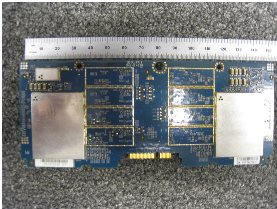
Shielded Radio Board Bottom
