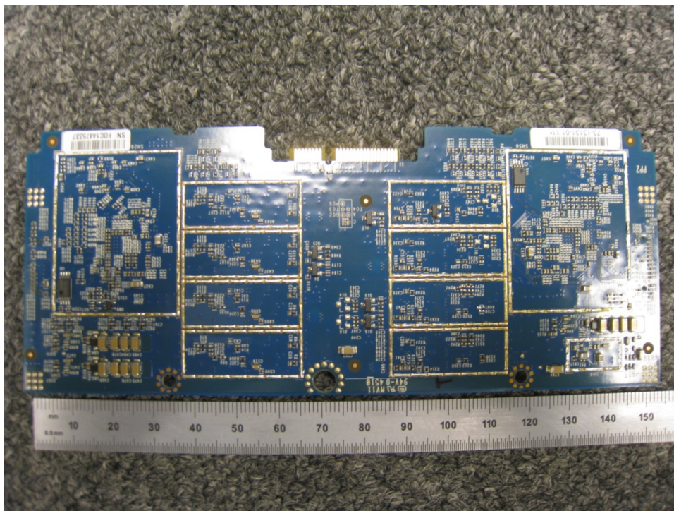
Unshielded Radio Board Bottom
