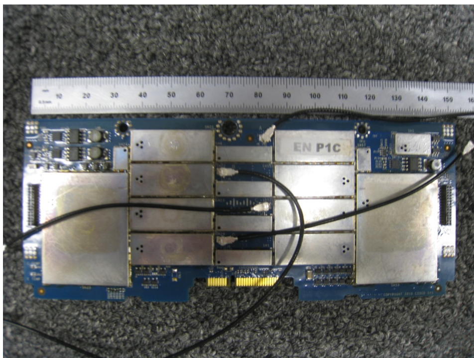
Shielded Radio Board Top
