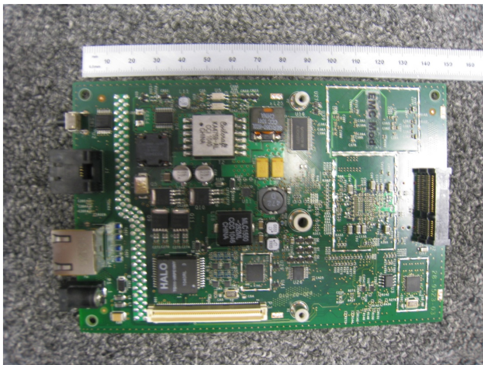
Motherboard Top
