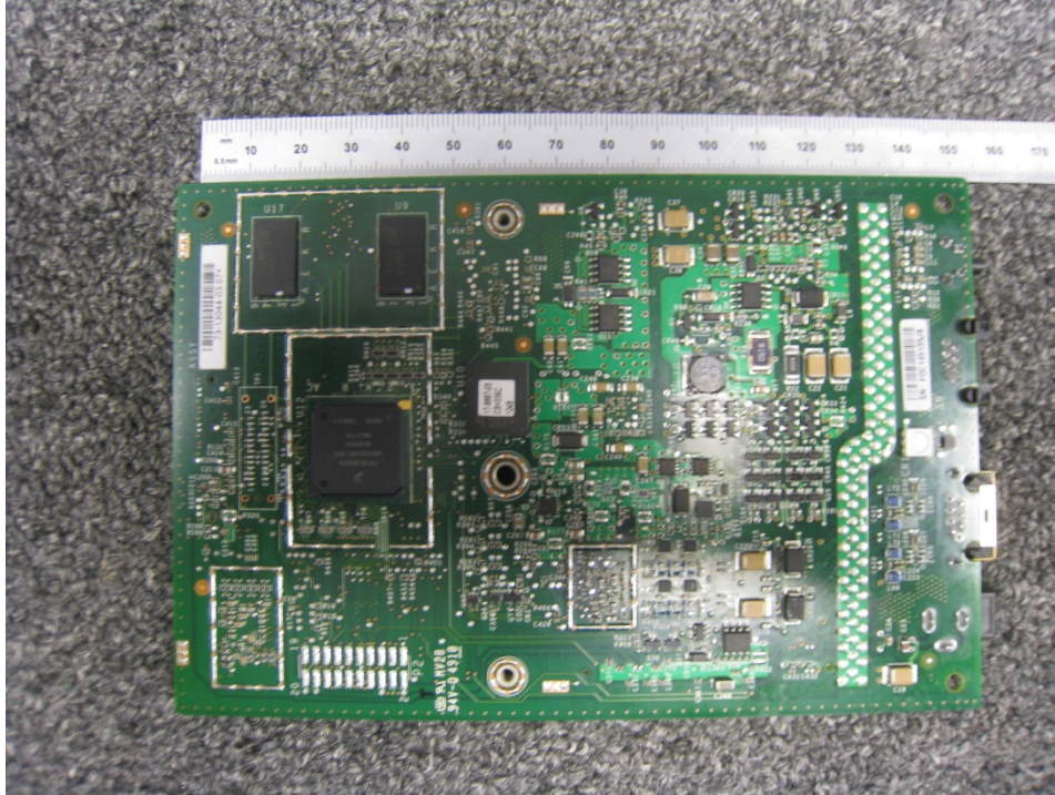
Motherboard Bottom
