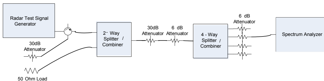
Conducted Calibration Setup
