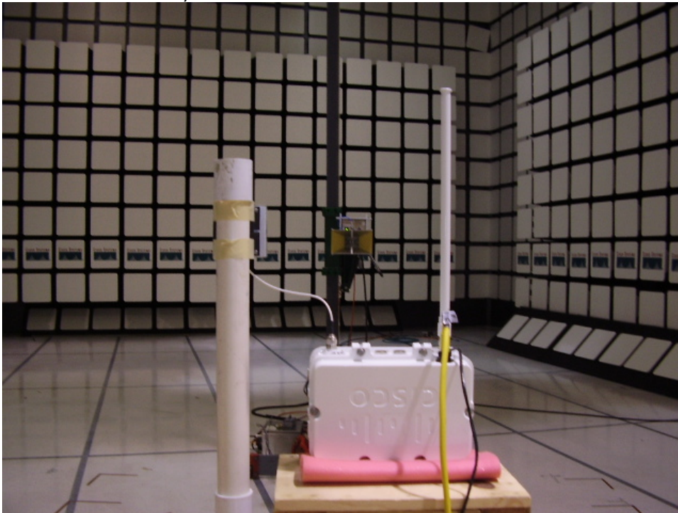
Radiated Emissions, 5GHz 14dBi Patch Antenna with 2.4GHz 8dBi Omni Antenna
