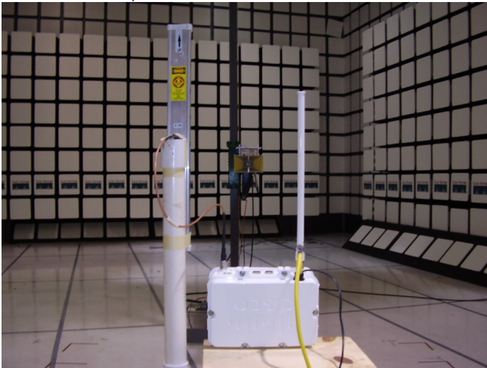
Radiated Emissions, 5GHz 17dBi Sector Antenna with 2.4GHz 8dBi Omni Antenna
