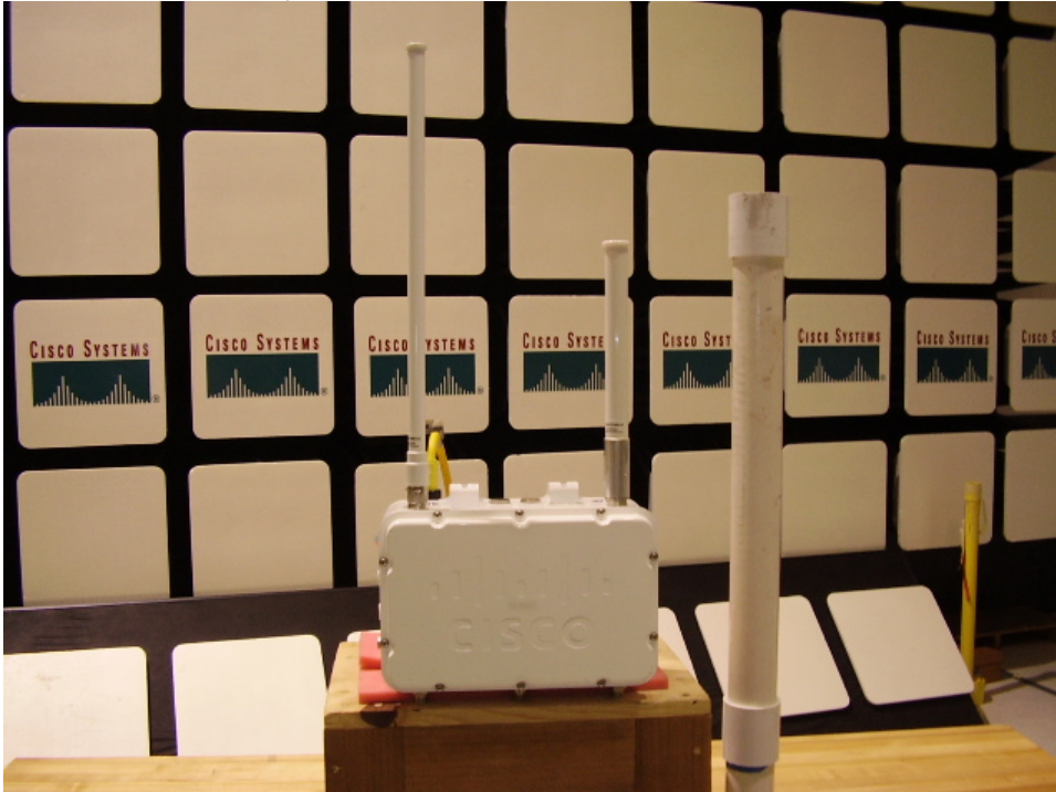
Radiated Emissions, 5GHz 8dBi Omni Antenna with 2.4GHz 8dBi Omni Antenna
