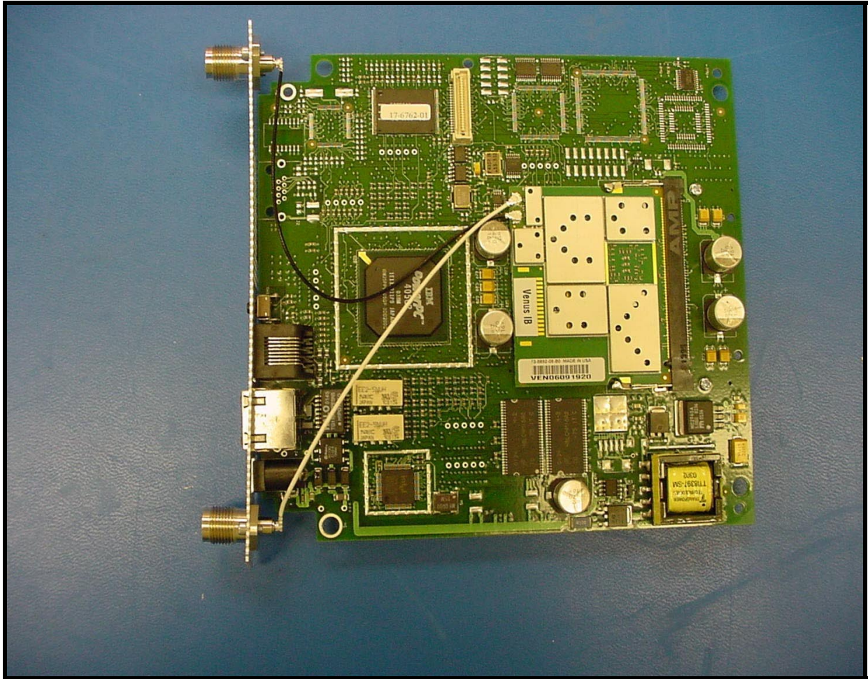
PHOTOGRAPH 9: AP1200 MOTHER BOARD WITH 2.4GHZ TX MODULE INSTALLED
