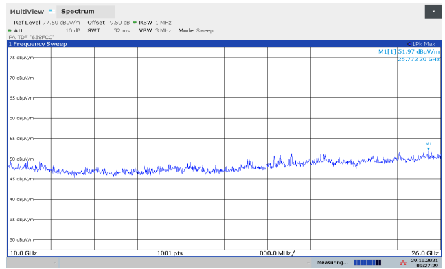
Prescan 18 - 26 GHz, 2440 MHz, 1Mb, HP, @1m
