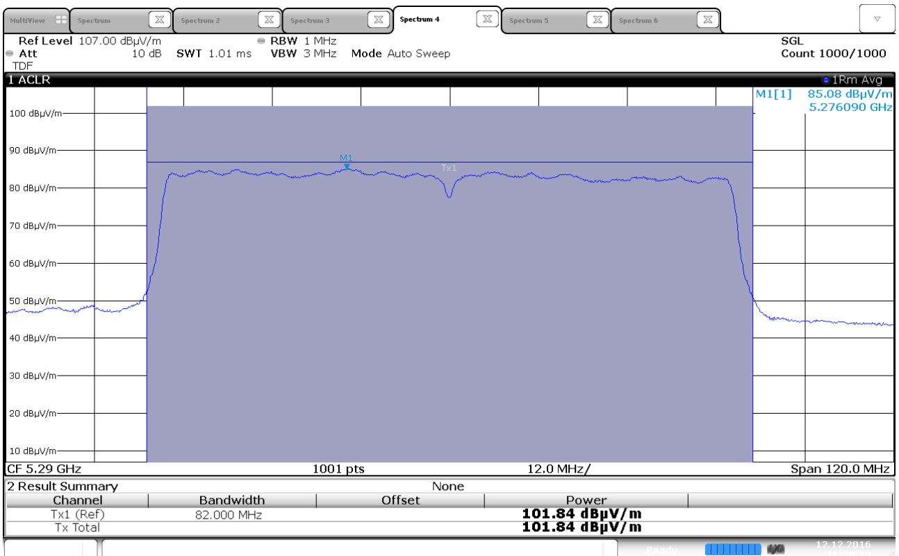
Maximum EIRP, 5290 MHz, 802.11n HT80, MIMO
