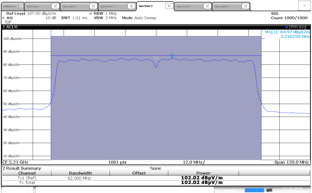
Maximum EIRP, 5210 MHz, 802.11n HT80, MIMO
