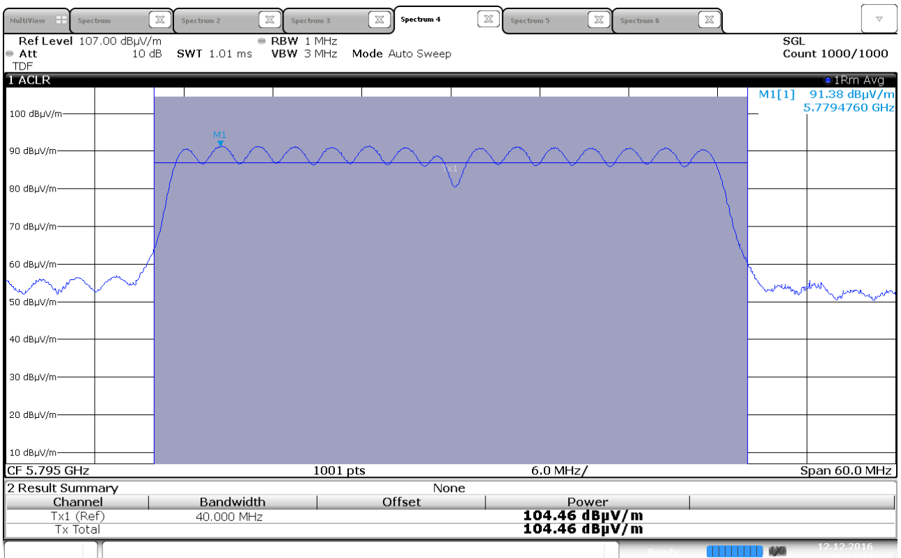
Maximum EIRP, 5795 MHz, 802.11n HT40, MIMO
