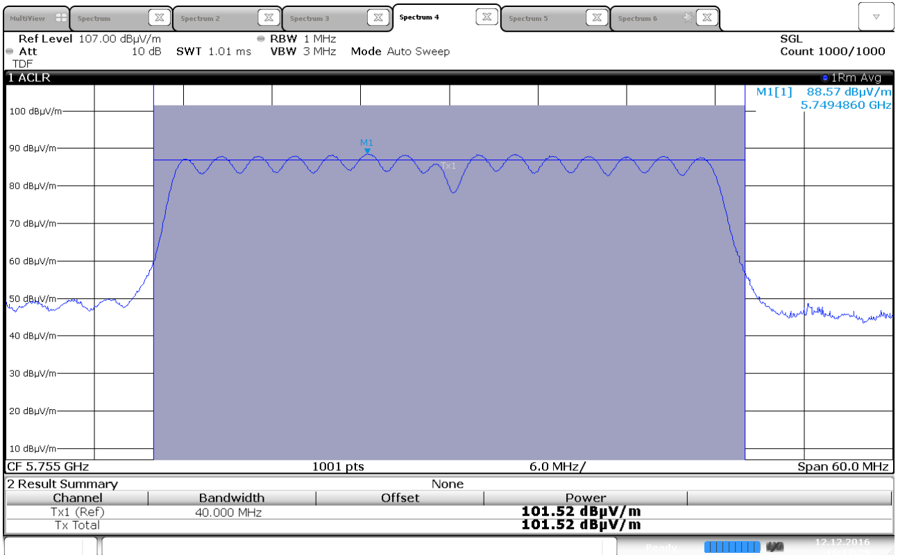
Maximum EIRP, 5755 MHz, 802.11n HT40, MIMO
