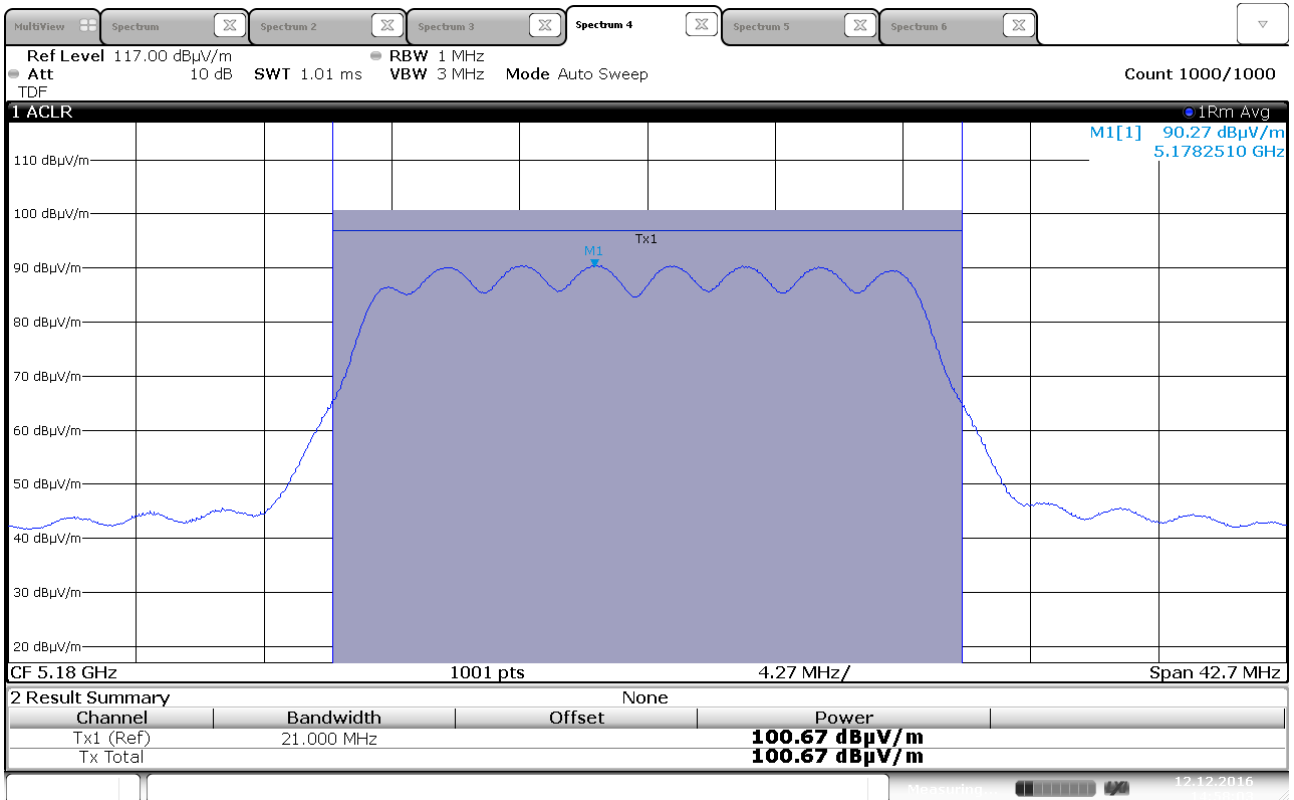
Maximum EIRP, 5180 MHz, 802.11n HT20, MIMO
