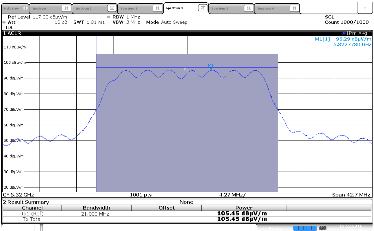
Maximum EIRP, 5320 MHz, 802.11n HT20, MIMO
