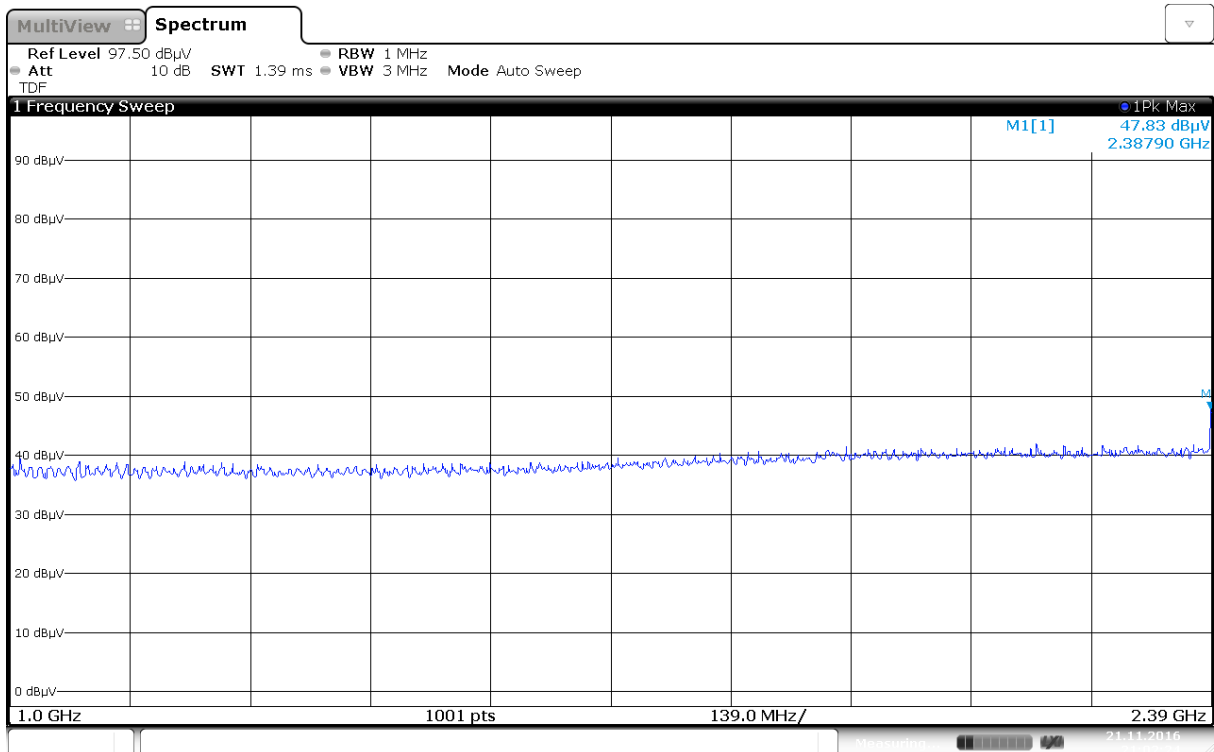
Radiated Emissions, 1000 -2390 MHz, 2412MHz, VP, 802.11g, 6Mb, Ant0
