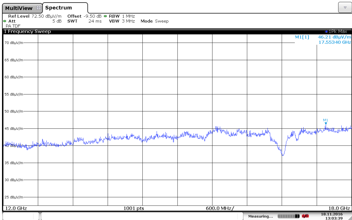
Radiated Emissions, 12000 -18000 MHz, 2437MHz, HP, 802.11b, 6Mbps, Ant0
