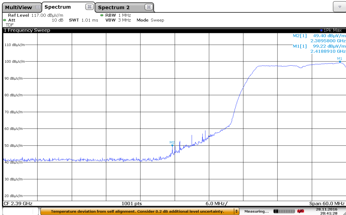
Band Edge, Lower, Peak, 2412 MHz, 802.11g, 6Mbps, Ant 1
