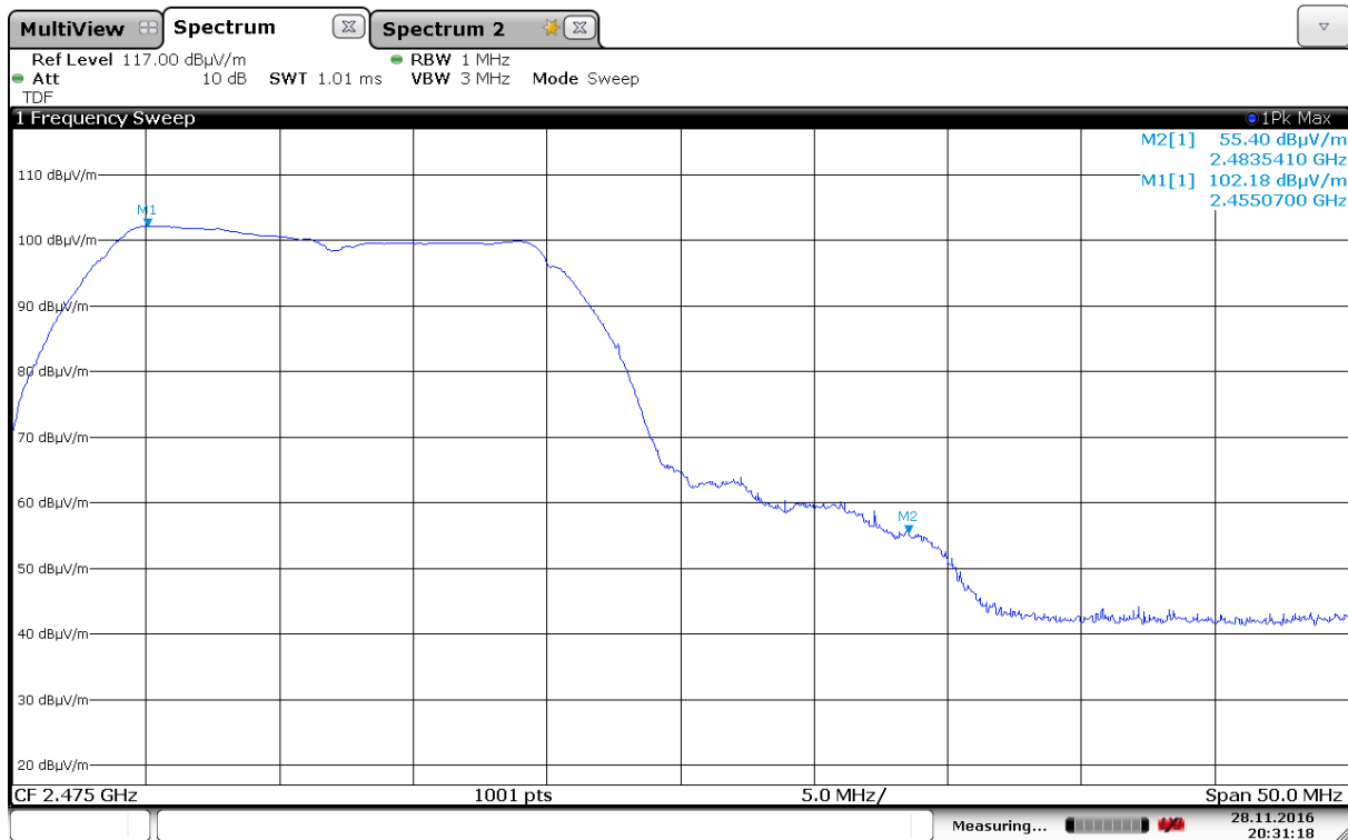
Band Edge, Upper, Peak, 2462 MHz, 802.11g, 6Mbps, Ant 1
