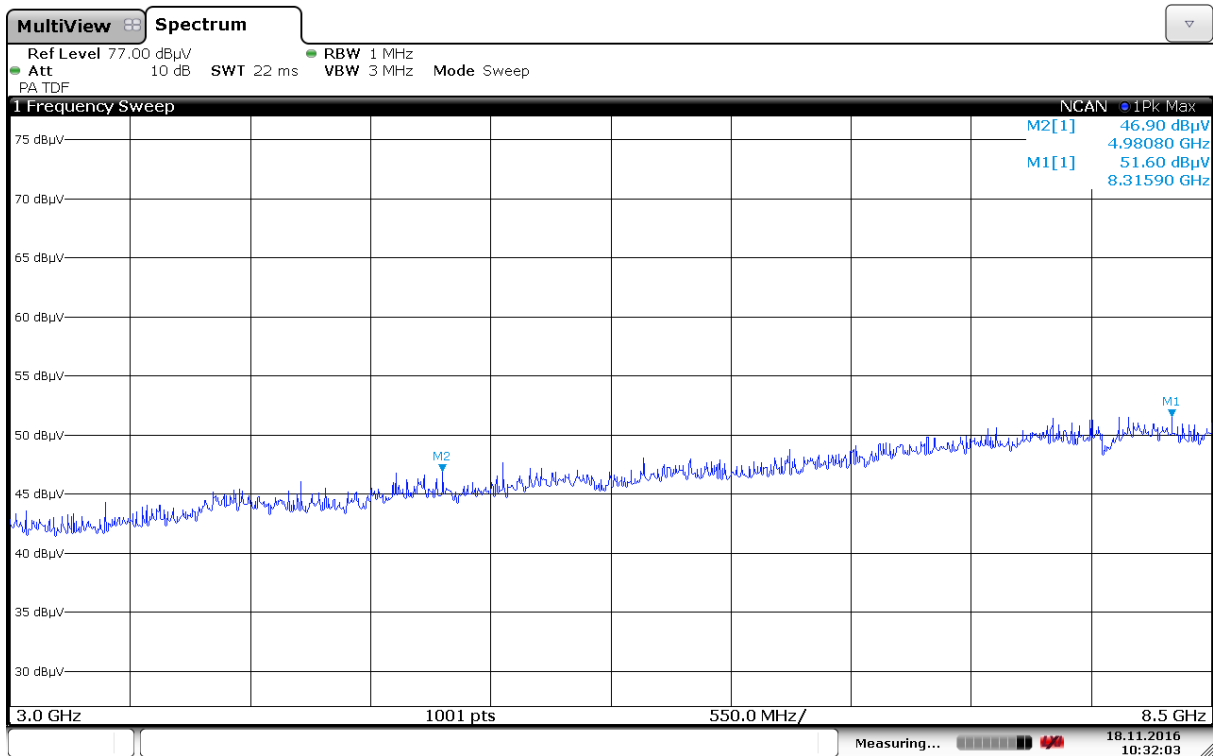
Radiated Emissions, 3000 -8500 MHz, 2442MHz, VP, 802.11g, 6Mbps, Ant1
