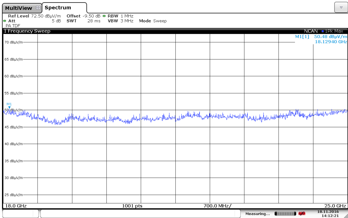
Radiated Emissions, 18000 -25000 MHz, 2437MHz, HP, 802.11n, MCS0, MIMO
