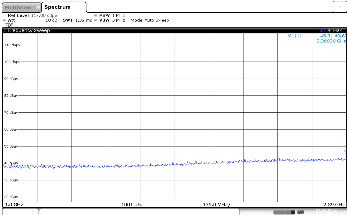
Radiated Emissions, 1000 -2390 MHz, 2412MHz, VP, 802.11b, 1Mb, Ant0
