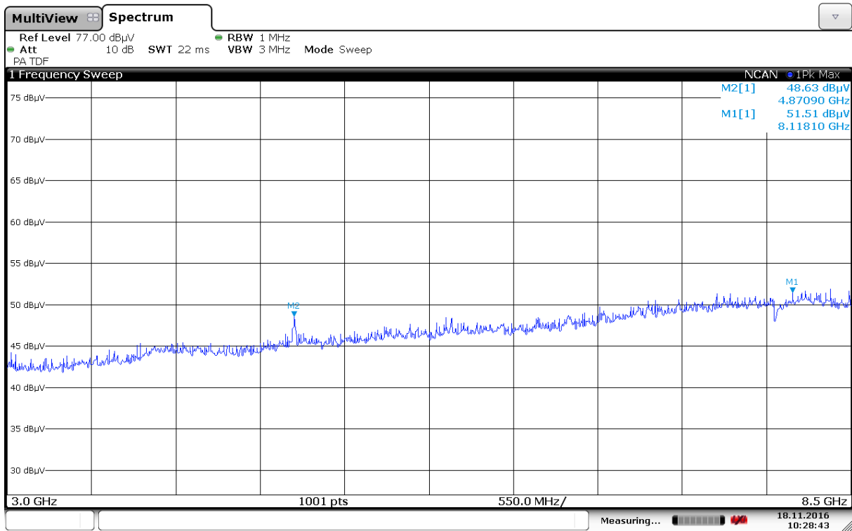
Radiated Emissions, 3000 -8500 MHz, 2442MHz, HP, 802.11g, 6Mbps, Ant1
