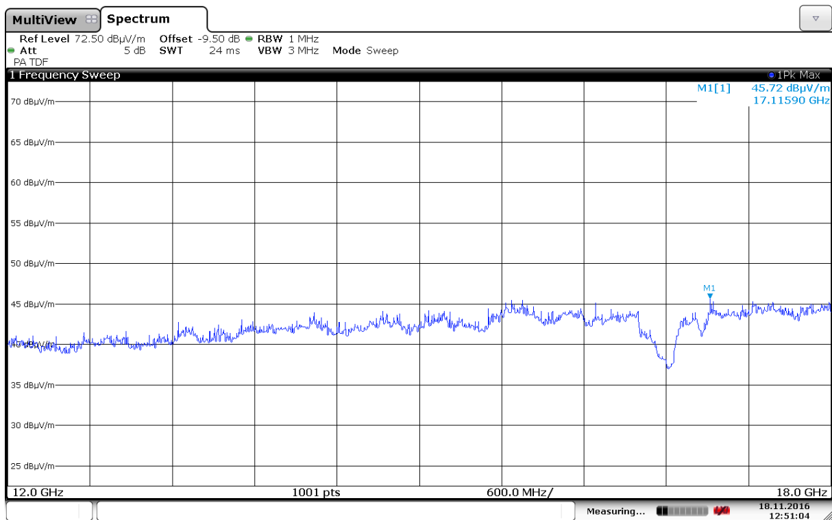
Radiated Emissions, 12000 -18000 MHz, 2437MHz, VP, 802.11n, MCS0, MIMO
