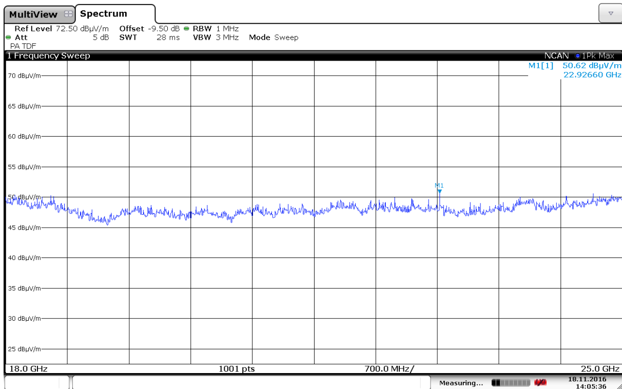
Radiated Emissions, 18000 -25000 MHz, 2437MHz, VP, 802.11b, 6Mbps, Ant1
