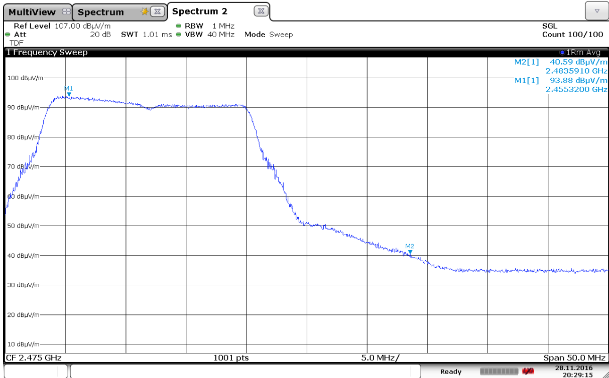
Band Edge, Upper, Average, 2462 MHz, 802.11g, 6Mbps, Ant 1
