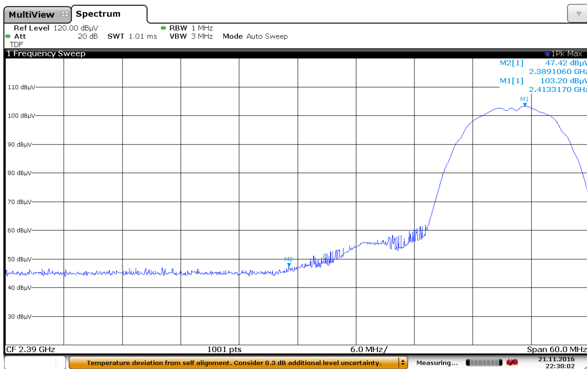
Band Edge, Lower, Peak, 2412 MHz, 802.11b, 1Mbps, Ant 0
