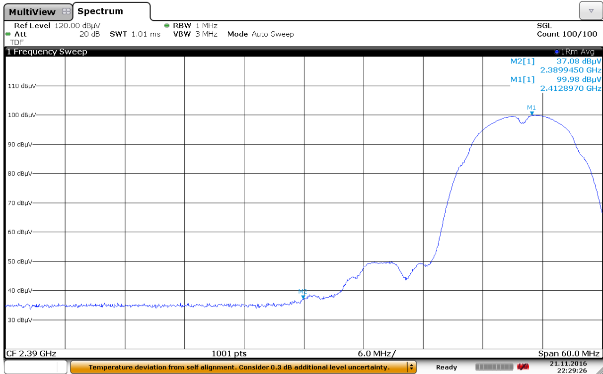
Band Edge, Lower, Average, 2412 MHz, 802.11b, 1Mbps, Ant 0
