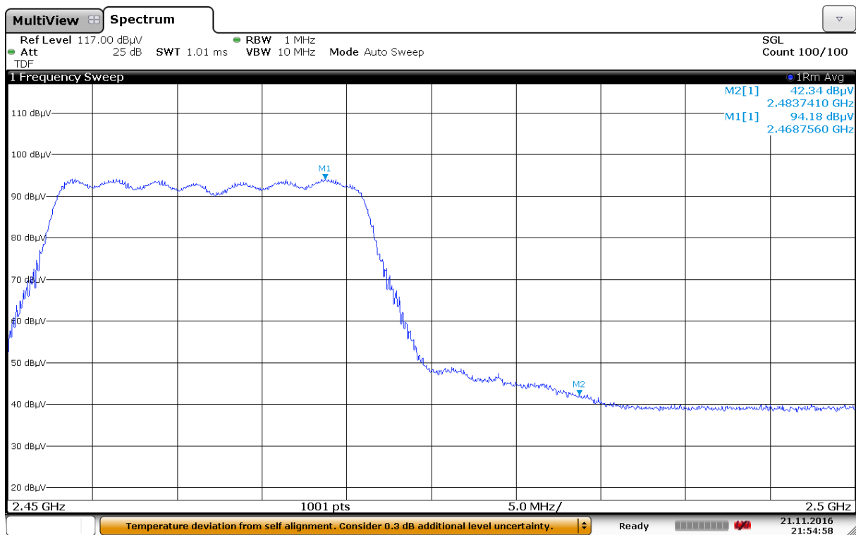
Band Edge, Upper, Average, 2462 MHz, 802.11n, MCS0, MIMO
