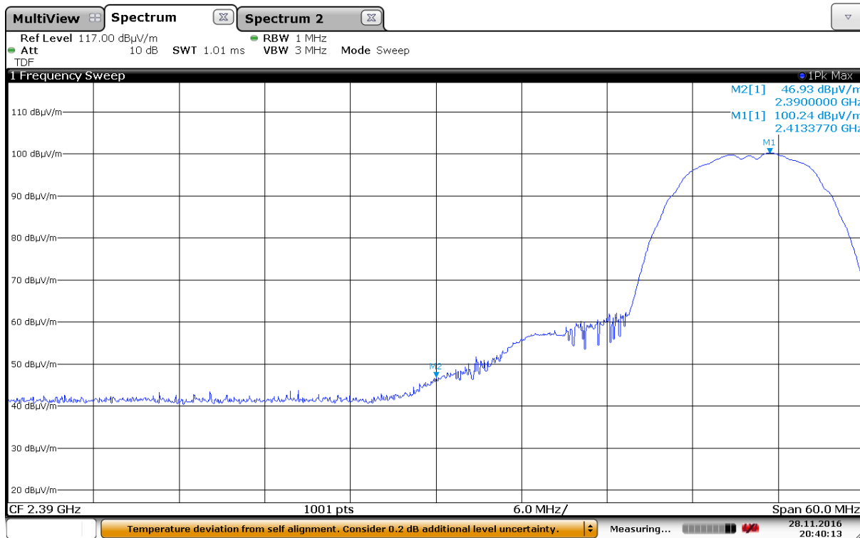
Band Edge, Lower, Peak, 2412 MHz, 802.11b, 1Mbps, Ant 1
