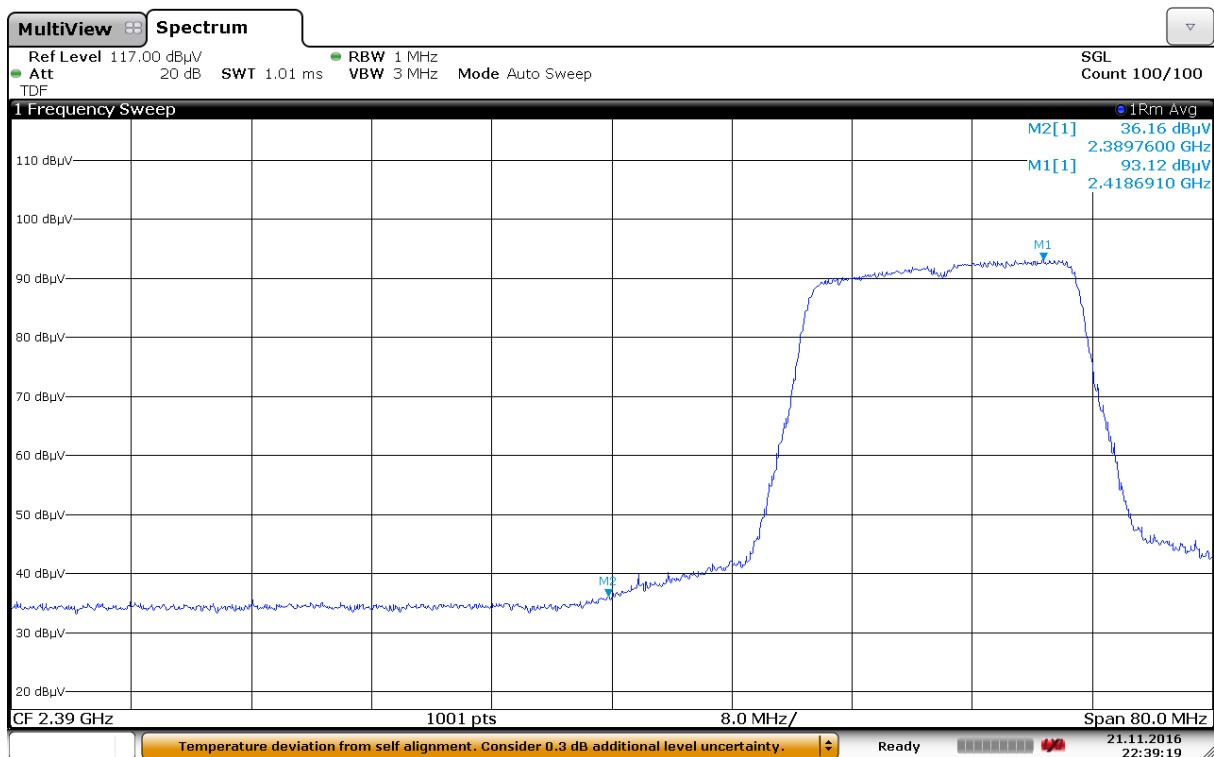
Band Edge, Lower, Average, 2412 MHz, 802.11n, MCS0, MIMO
