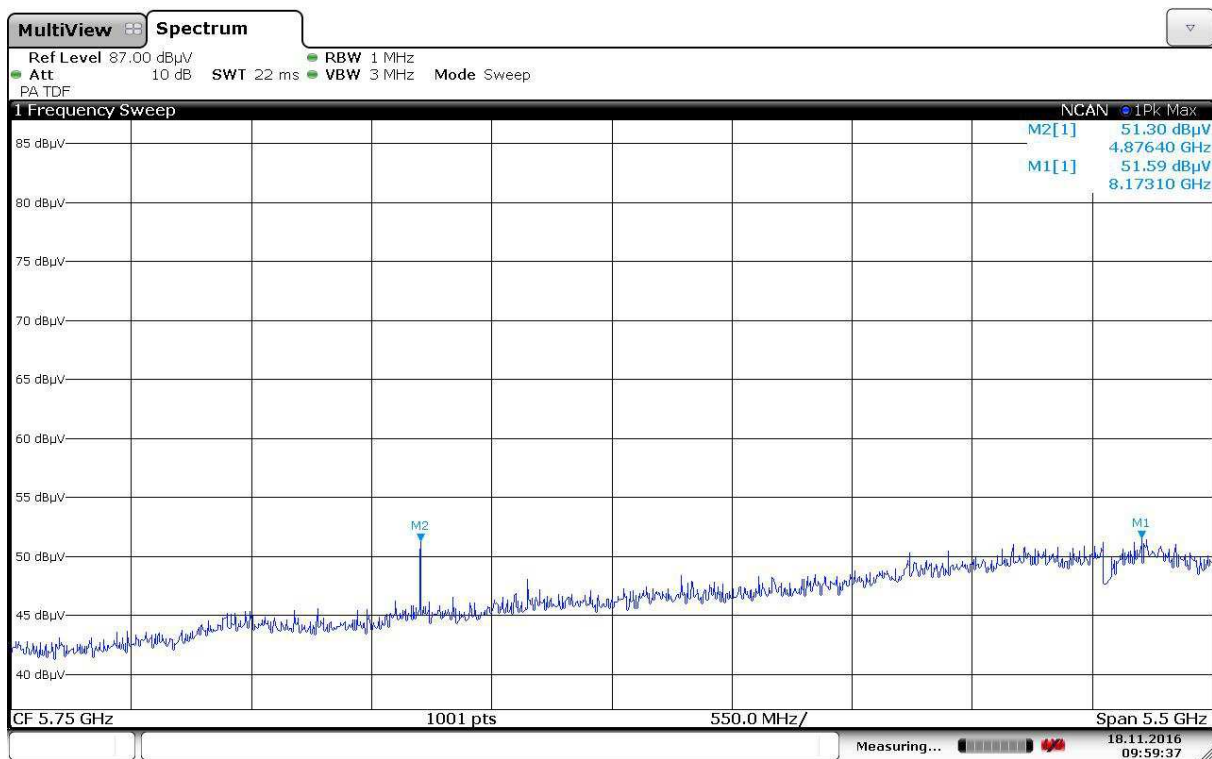
Radiated Emissions, 3000 -8500 MHz, 2442MHz, HP, 802.11b, 6Mbps, Ant1
