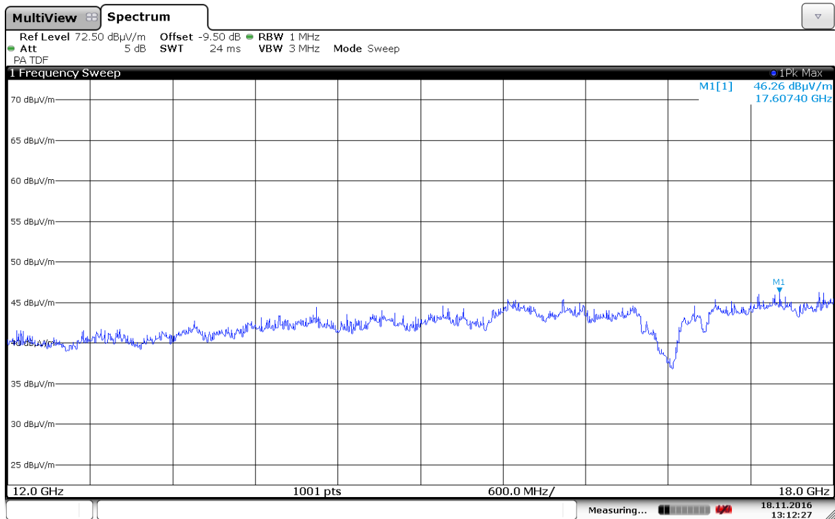
Radiated Emissions, 12000 -18000 MHz, 2437MHz, VP, 802.11b, 6Mbps, Ant1
