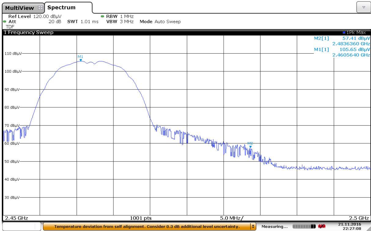
Band Edge, Upper, Peak, 2462 MHz, 802.11b, 1Mbps, Ant 0
