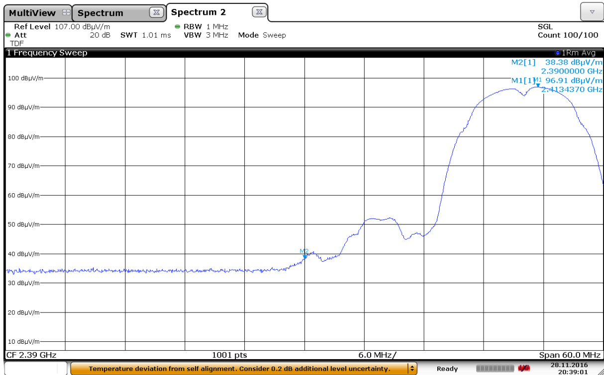
Band Edge, Lower, Average, 2412 MHz, 802.11b, 1Mbps, Ant 1
