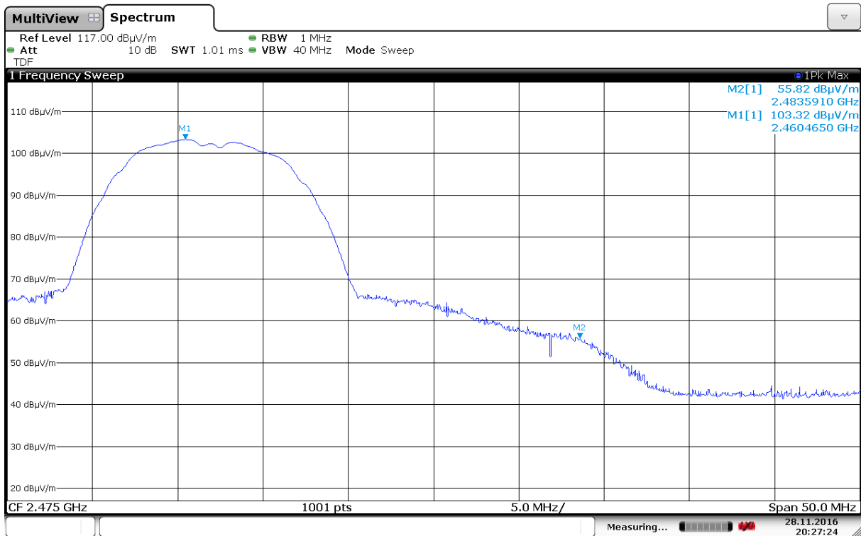
Band Edge, Upper, Peak, 2462 MHz, 802.11b, 1Mbps, Ant 1
