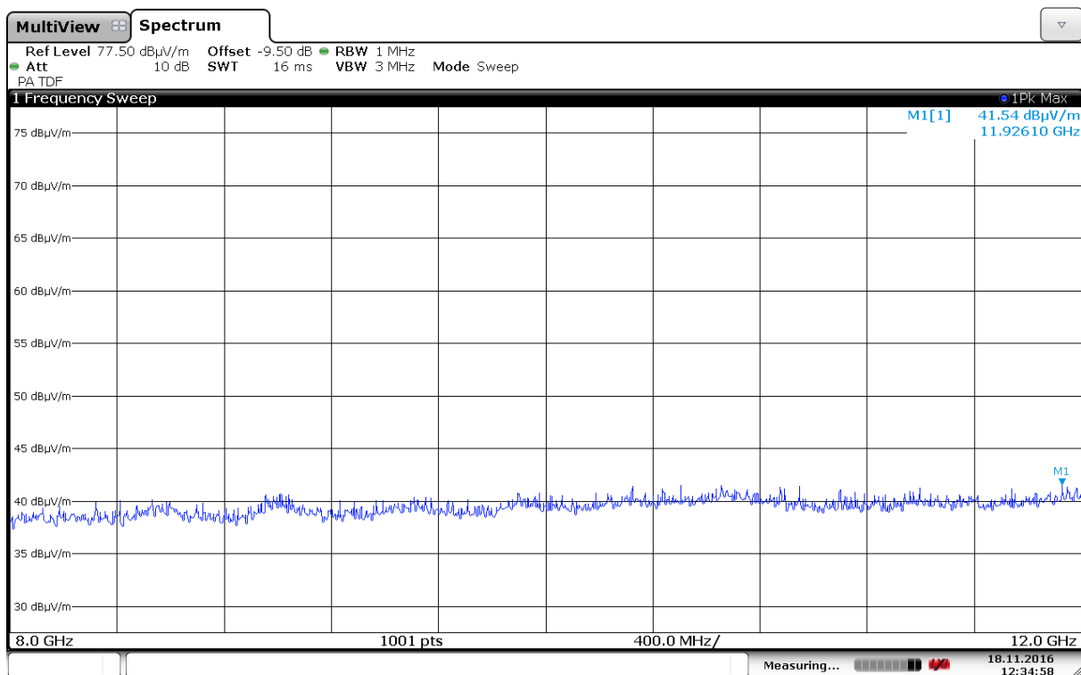
Radiated Emissions, 8000 -12000 MHz, 2437MHz, HP, 802.11b, 6Mbps, Ant1
