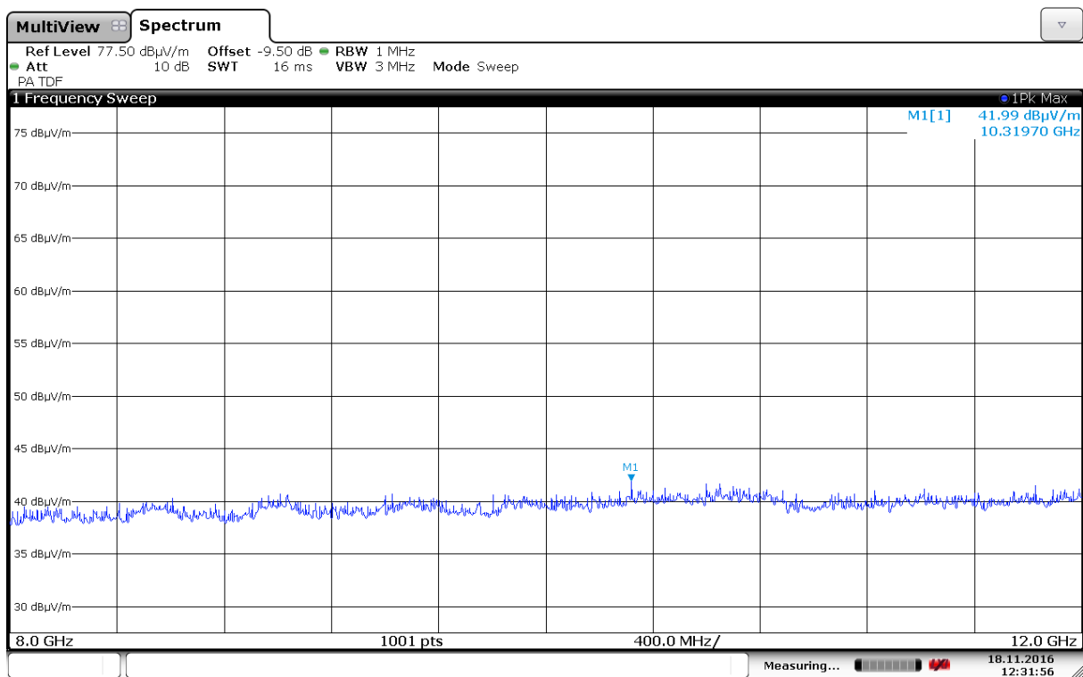
Radiated Emissions, 8000 -12000 MHz, 2437MHz, HP, 802.11b, 6Mbps, Ant0
