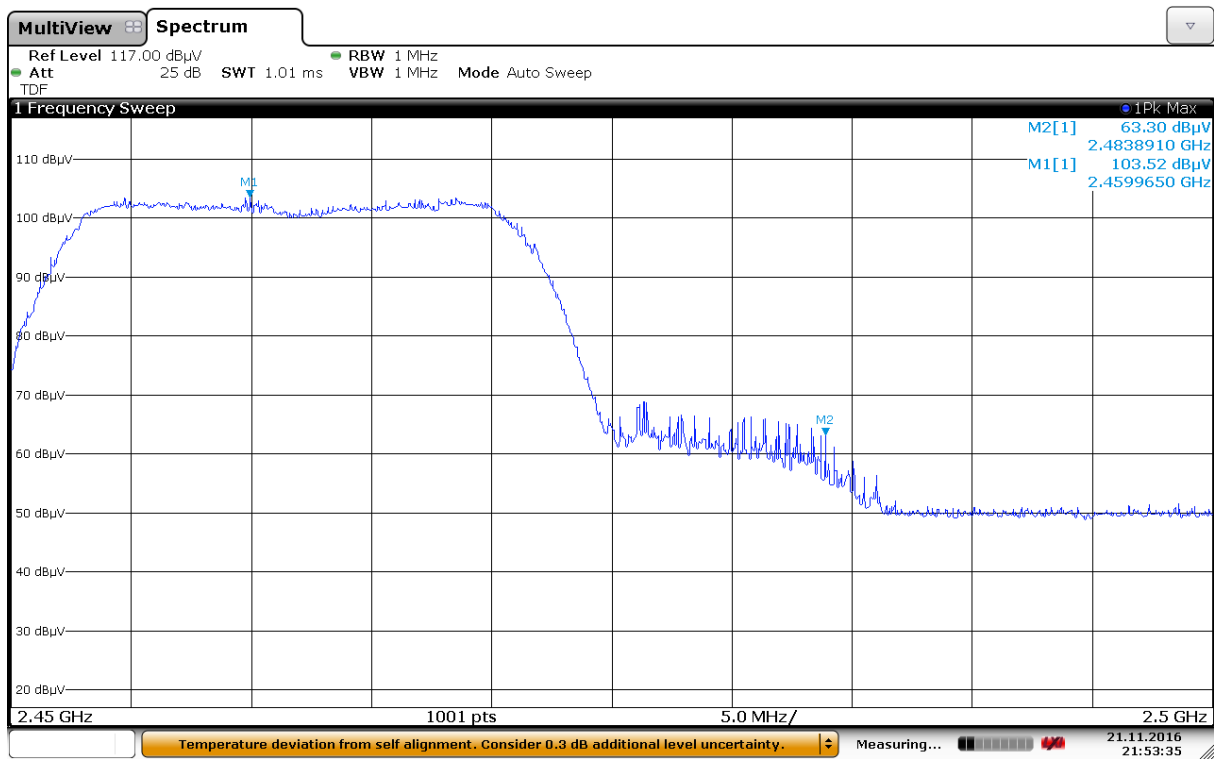
Band Edge, Upper, Peak, 2462 MHz, 802.11n, MCS0, MIMO
