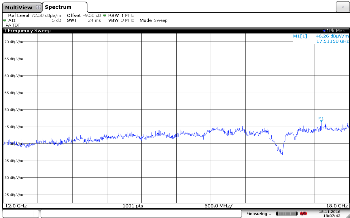
Radiated Emissions, 12000 -18000 MHz, 2437MHz, HP, 802.11b, 6Mbps, Ant1
