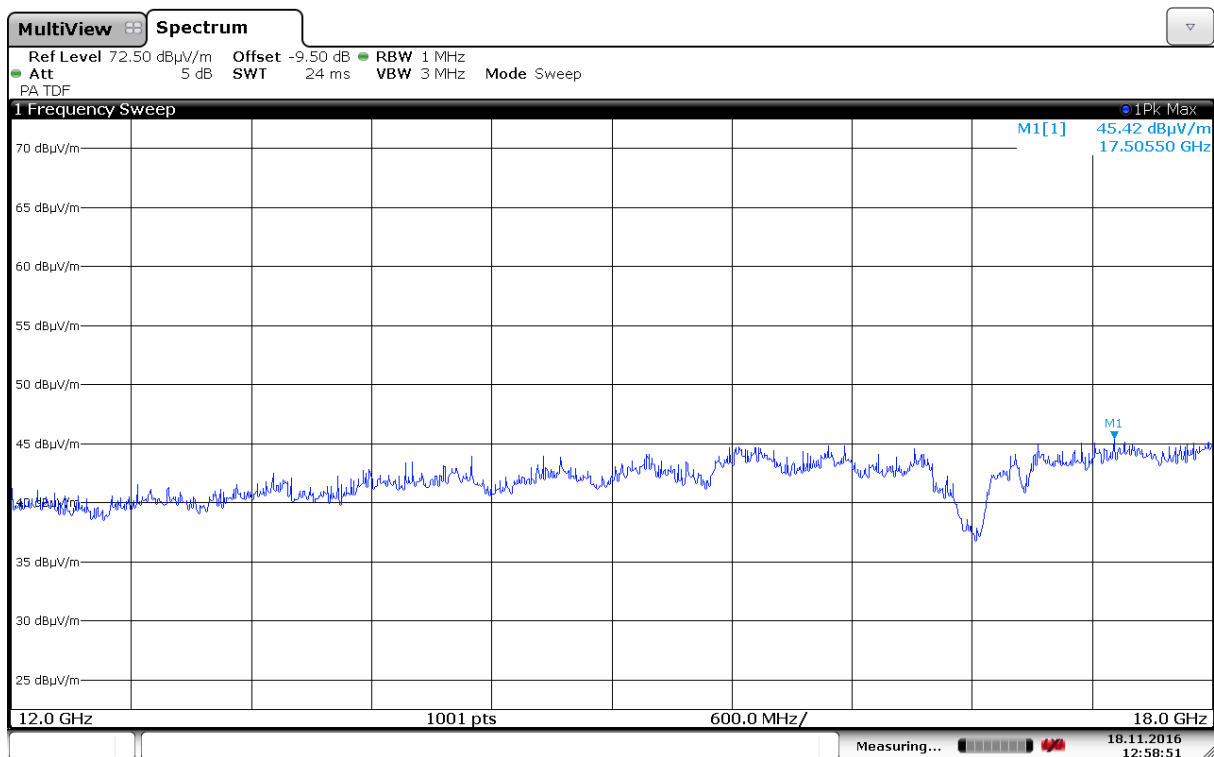
Radiated Emissions, 12000 -18000 MHz, 2437MHz, VP, 802.11b, 6Mbps, Ant0
