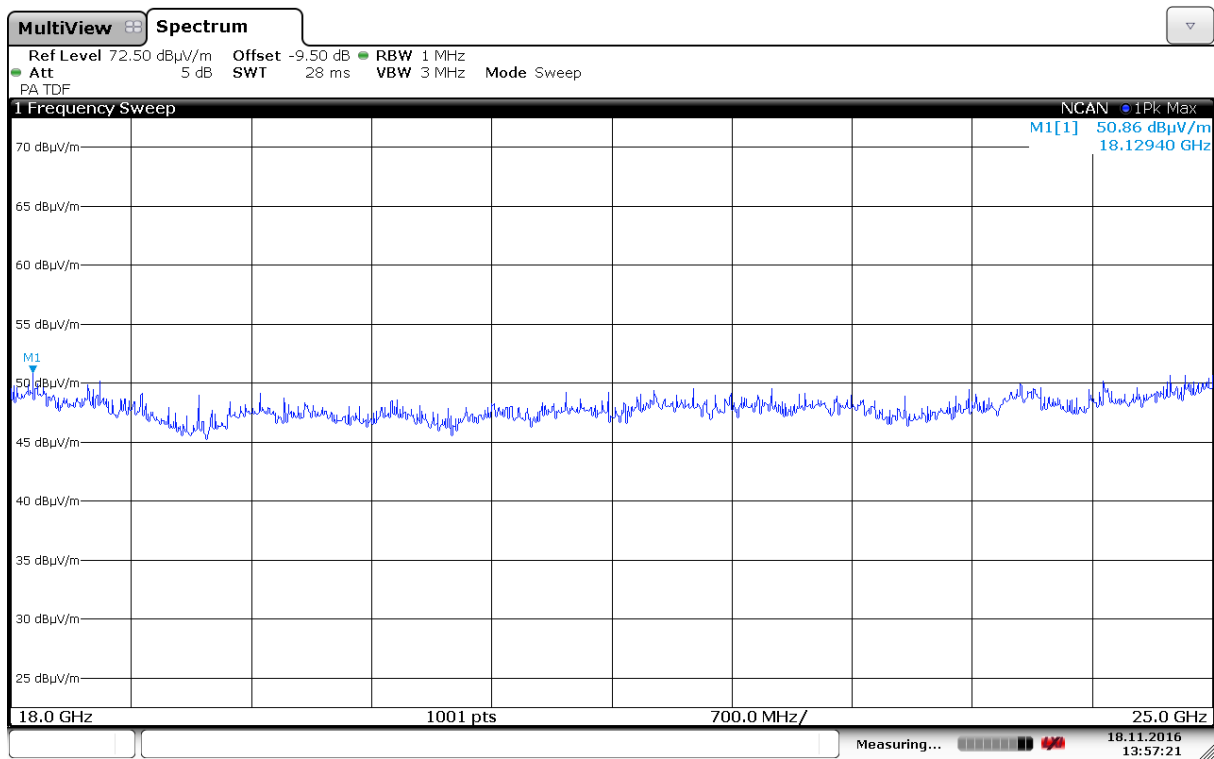
Radiated Emissions, 18000 -25000 MHz, 2437MHz, HP, 802.11b, 6Mbps, Ant0
