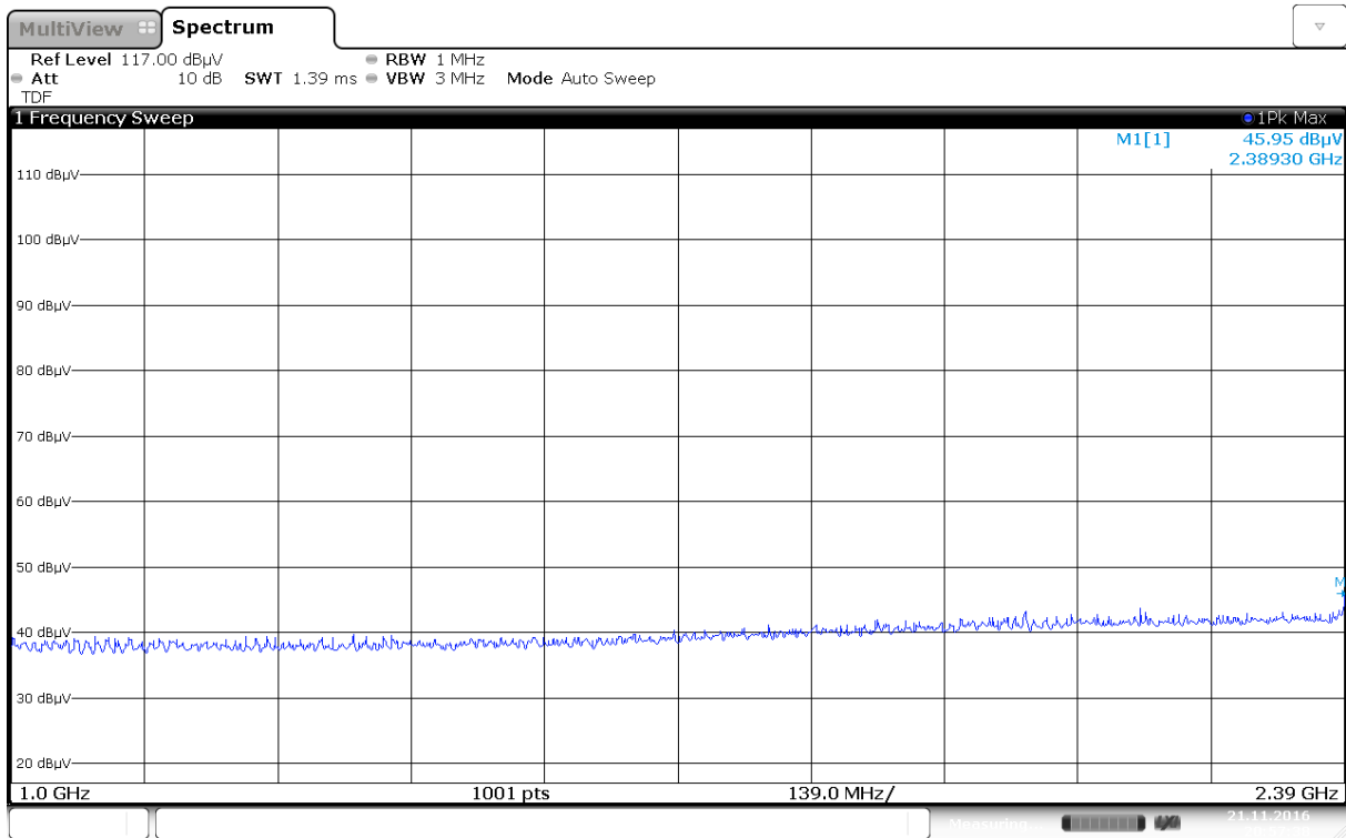
Radiated Emissions, 1000 -2390 MHz, 2412MHz, HP, 802.11b, 1Mb, Ant1
