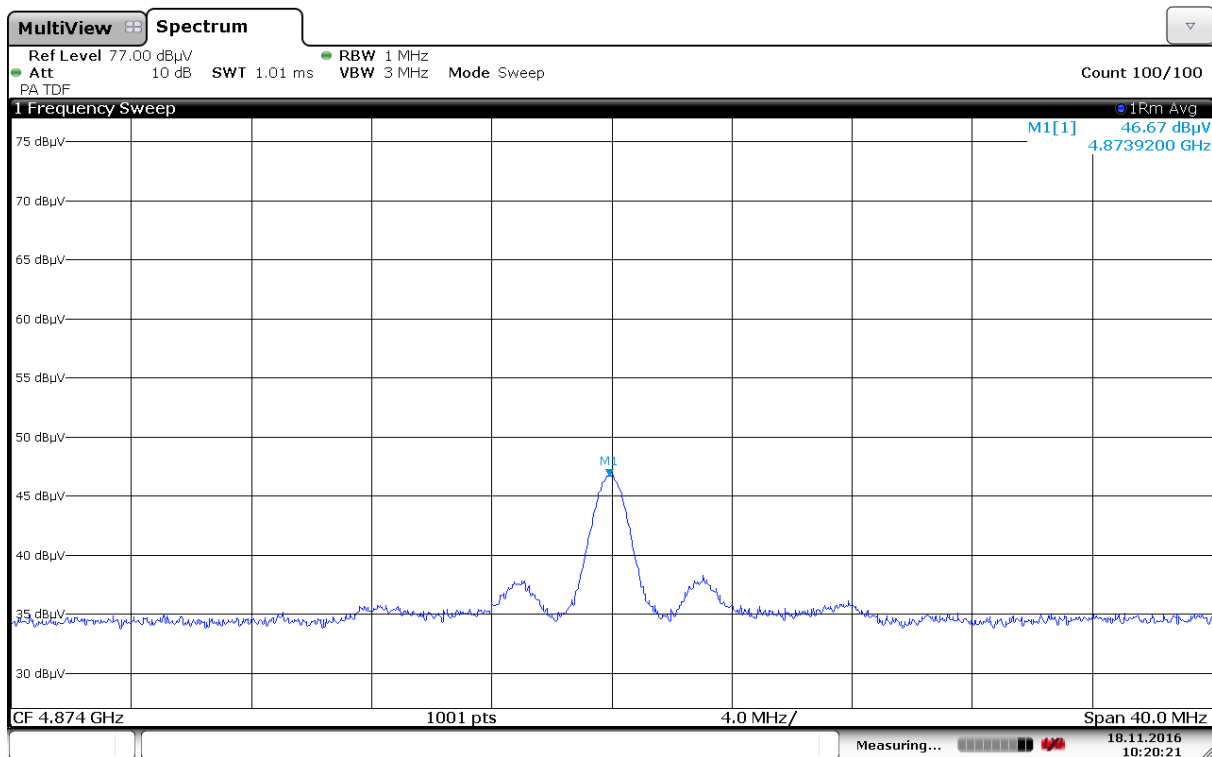
Radiated Emissions Av, 4874MHz, 2437MHz, HP, 802.11b, 1Mb, Ant1
