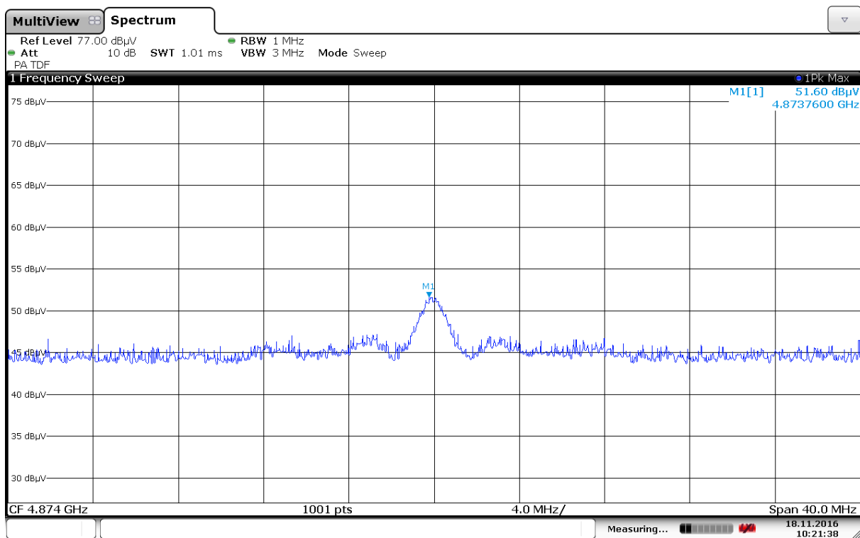
Radiated Emissions Pk, 4874MHz, 2437MHz, HP, 802.11b, 1Mb, Ant1
