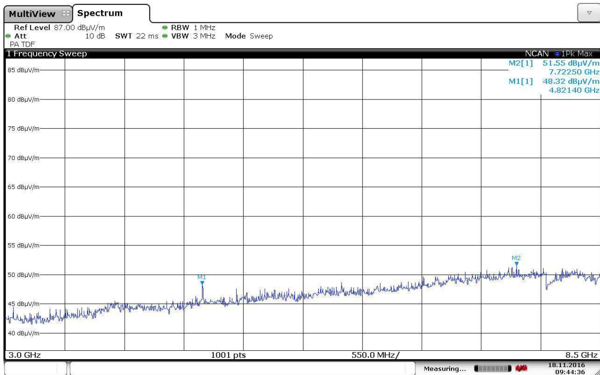
Radiated Emissions, 3000 -8500 MHz, 2412MHz, HP, 802.11b, 6Mbps, Ant0
