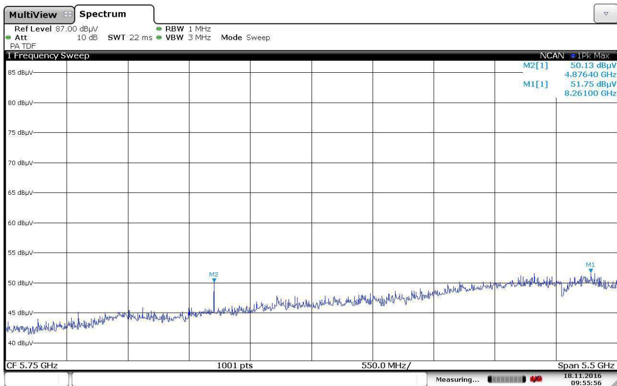
Radiated Emissions, 3000 -8500 MHz, 2442MHz, VP, 802.11b, 6Mbps, Ant1
