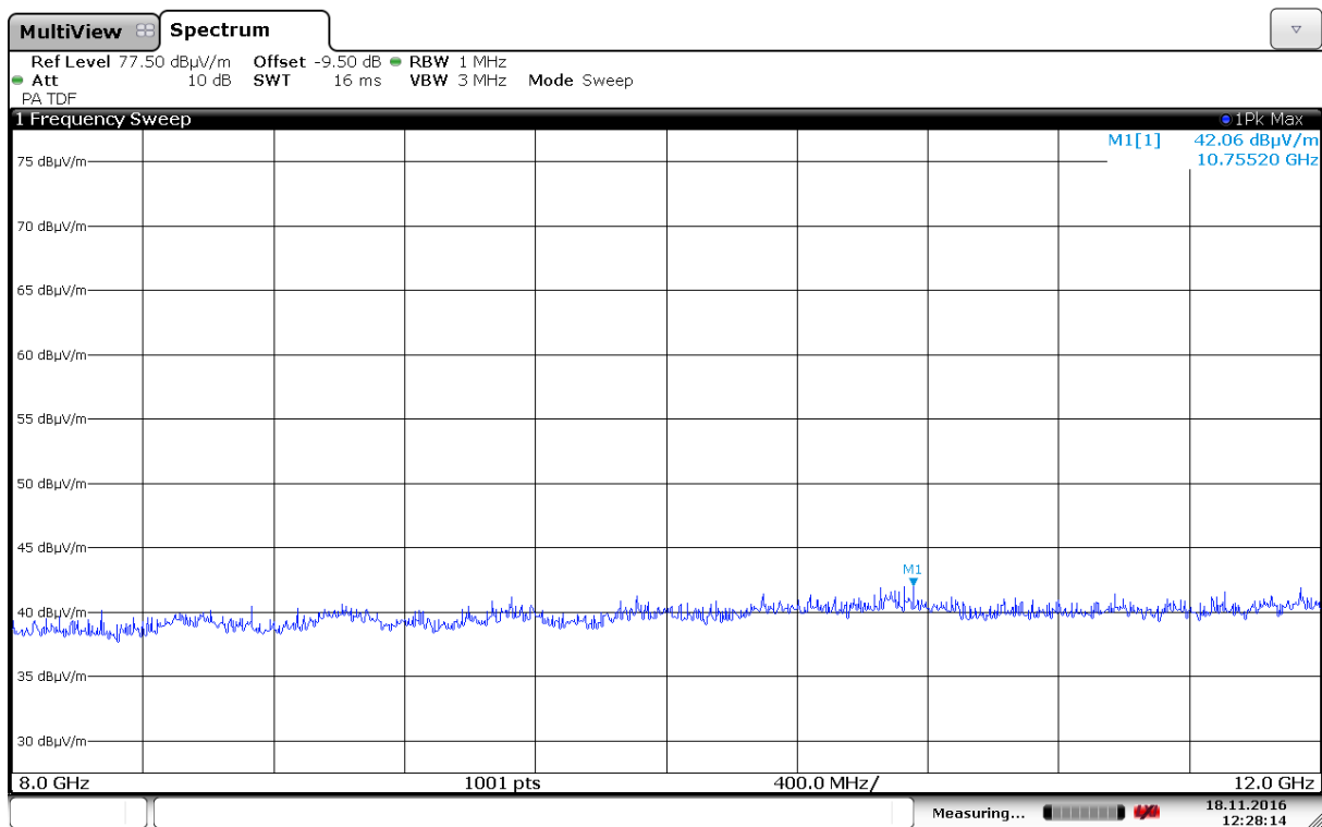
Radiated Emissions, 8000 -12000 MHz, 2437MHz, VP, 802.11b, 6Mbps, Ant0
