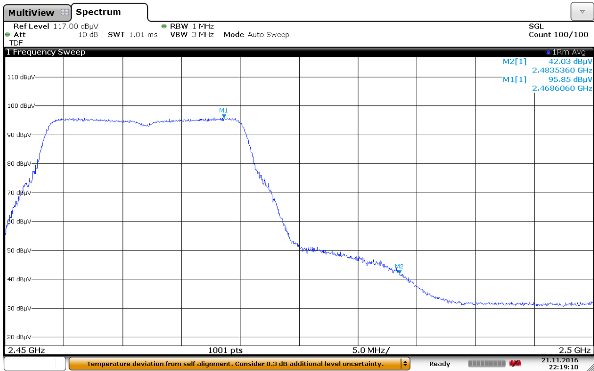
Band Edge, Upper, Average, 2462 MHz, 802.11g, 6Mbps, Ant 0
