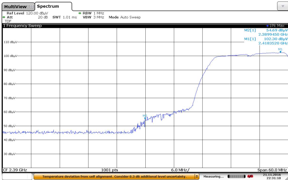
Band Edge, Lower, Peak, 2412 MHz, 802.11g, 6Mbps, Ant 0
