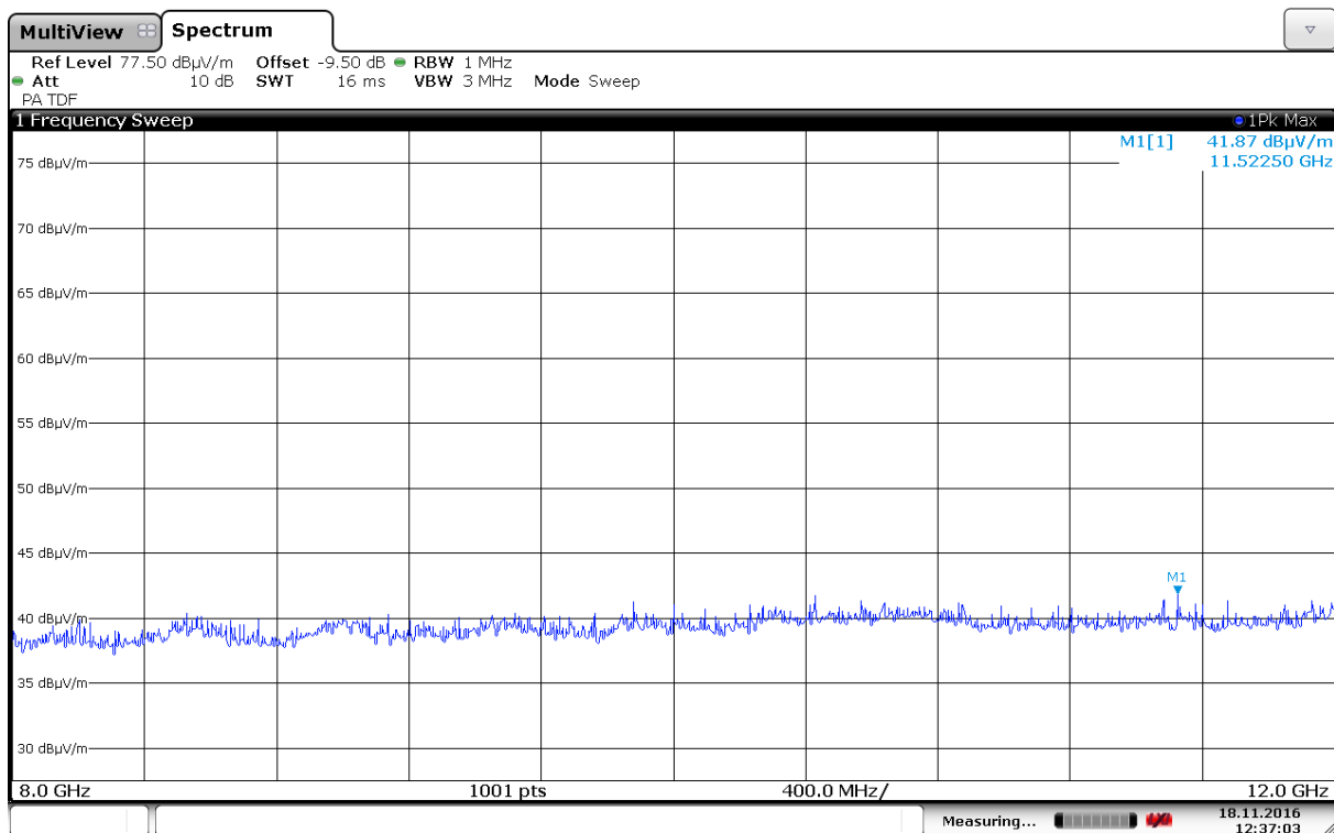
Radiated Emissions, 8000 -12000 MHz, 2437MHz, VP, 802.11b, 6Mbps, Ant1
