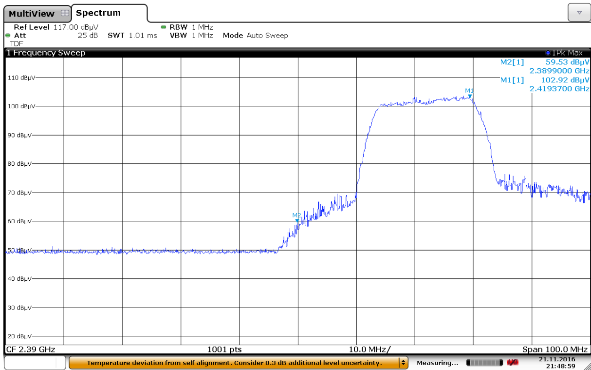
Band Edge, Lower, Peak, 2412 MHz, 802.11n, MCS0, MIMO
