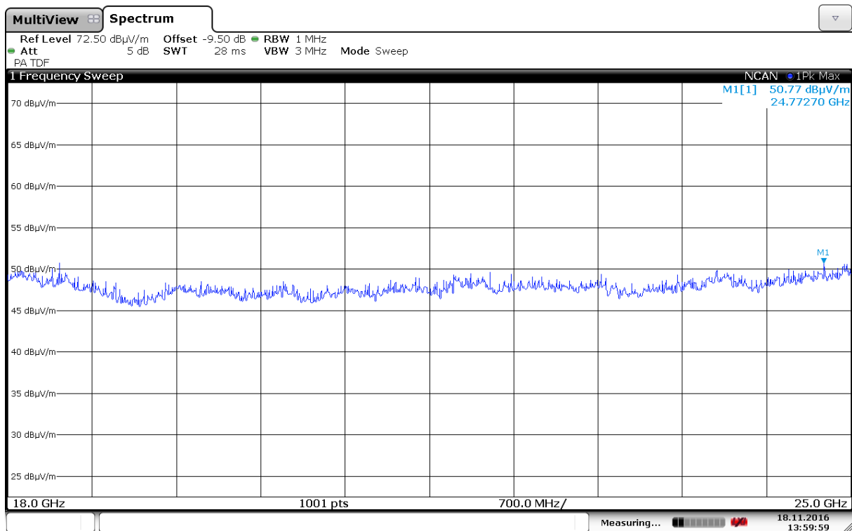
Radiated Emissions, 18000 -25000 MHz, 2437MHz, VP, 802.11b, 6Mbps, Ant0
