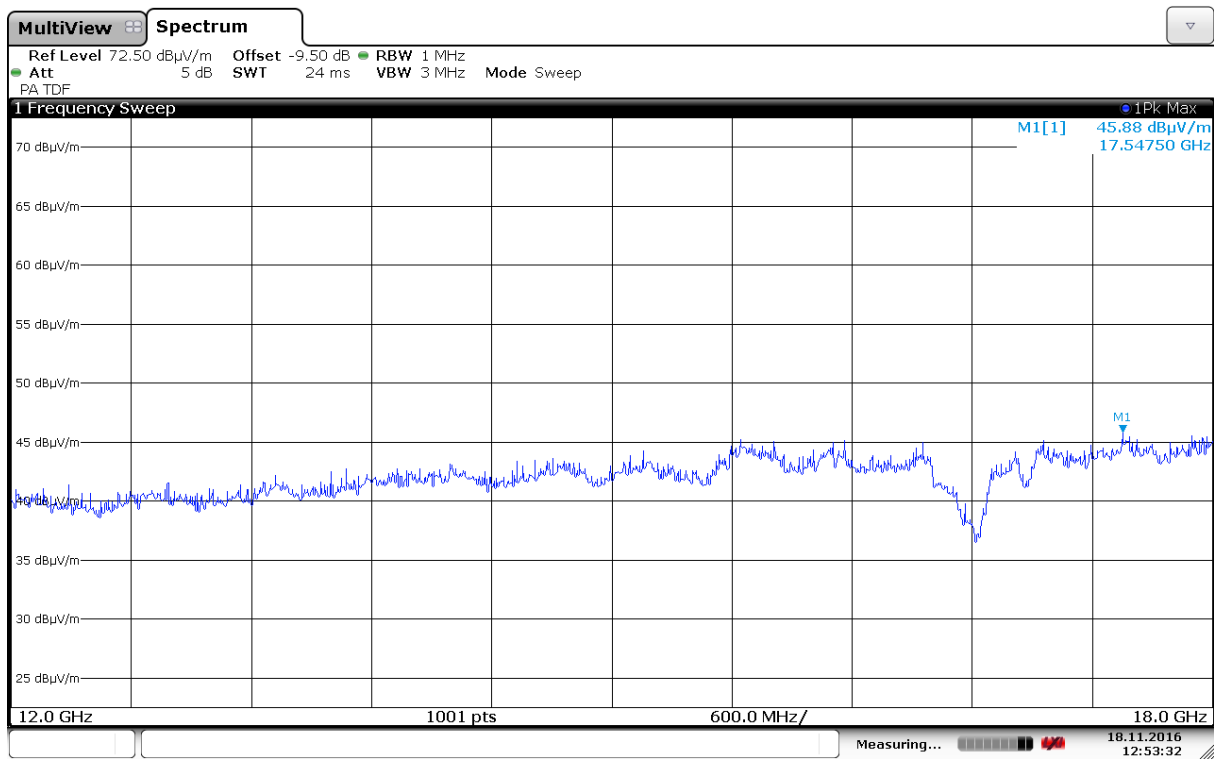
Radiated Emissions, 12000 -18000 MHz, 2437MHz, HP, 802.11n, MCS0, MIMO
