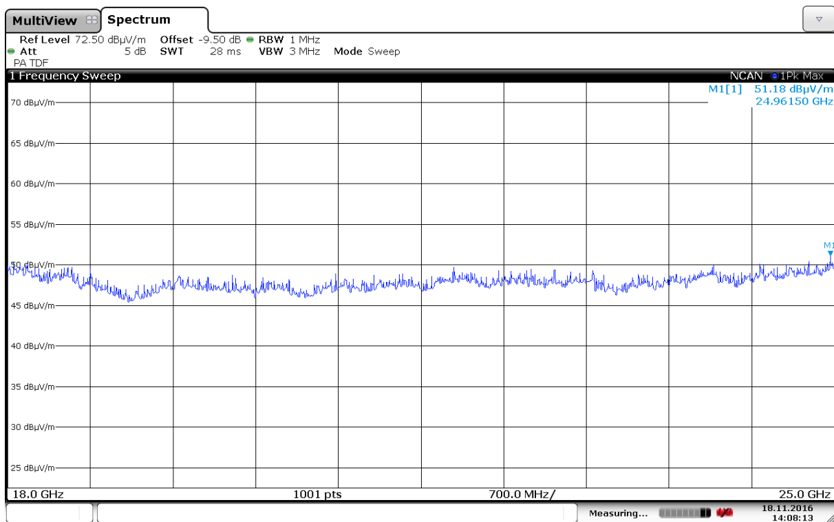
Radiated Emissions, 18000 -25000 MHz, 2437MHz, HP, 802.11b, 6Mbps, Ant1
