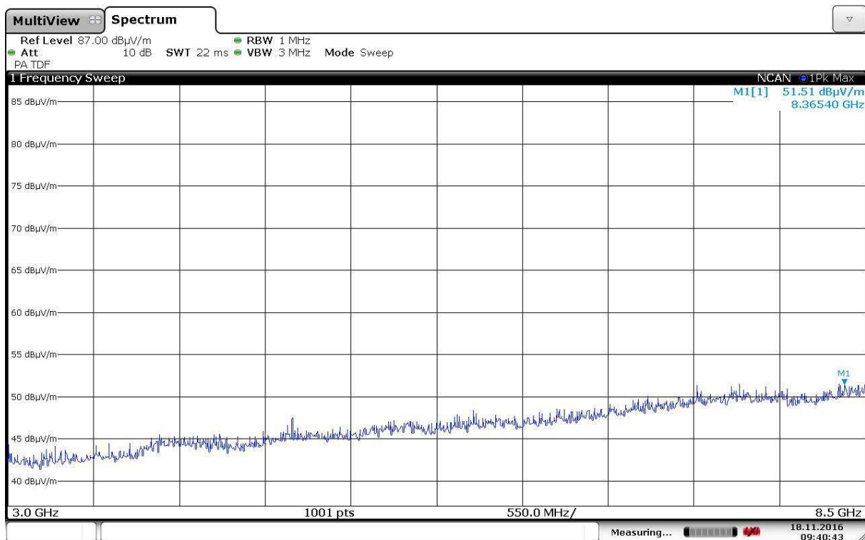
Radiated Emissions, 3000 -8500 MHz, 2412MHz, VP, 802.11b, 6Mbps, Ant0
