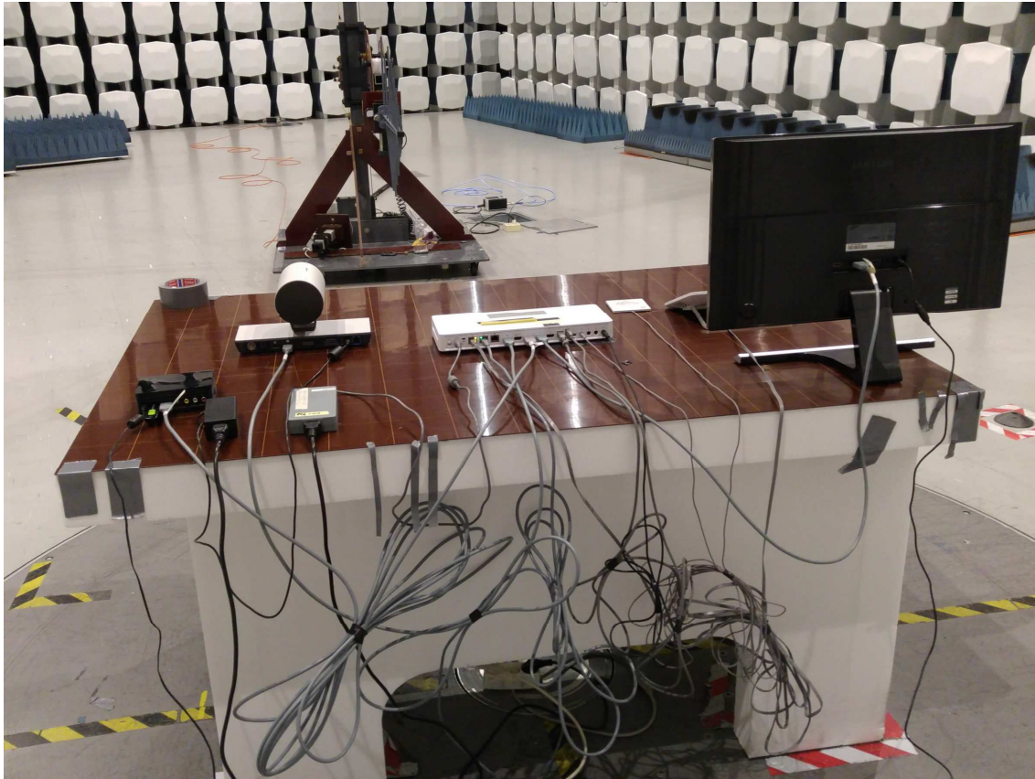
Radiated Emissions, 30 - 200 MHz
