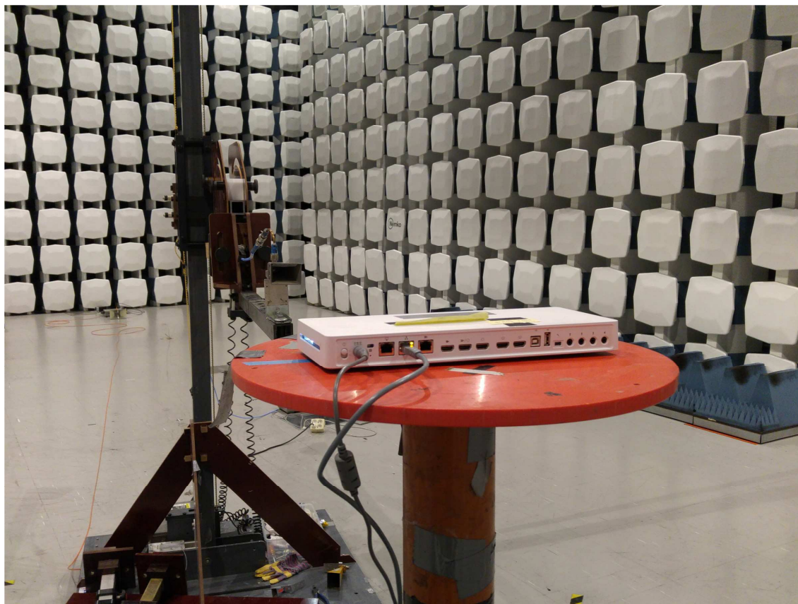
Radiated Emissions, 8 – 18 GHz
