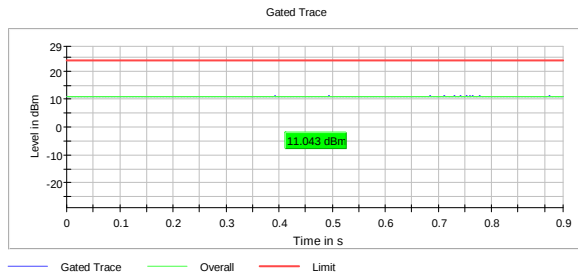
RMS Conducted Power, 5500 MHz, 802.11a, 6Mb
