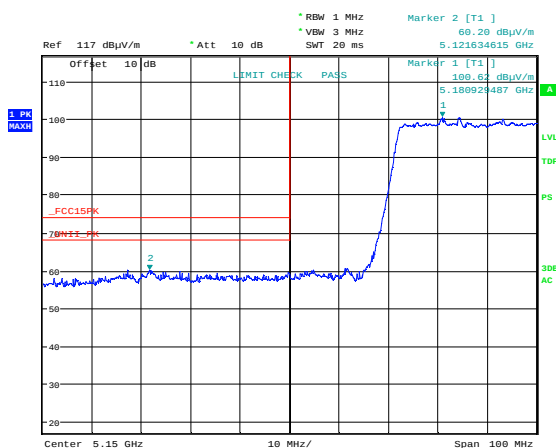
Band Edge 5150 MHz, ch042, 802.11ac MCS0 MIMO, Radiated, Max
