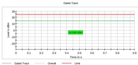
RMS Conducted Power, 5580 MHz, 802.11a, 6Mb
