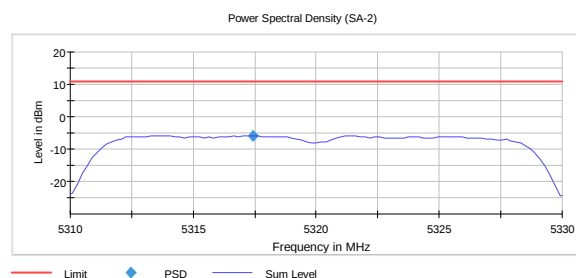
MCS15 -5.9 dBm
