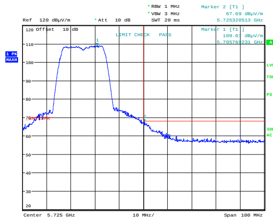
Band Edge 5725 MHz, ch140, 802.11n MCS0, Radiated, Max
