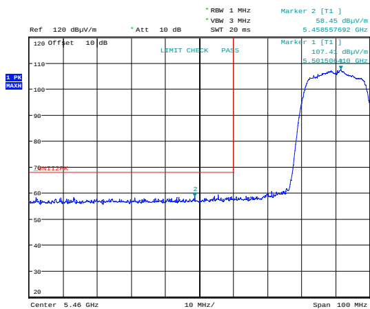
Band Edge 5470 MHz, ch100, 802.11n MCS7, Radiated, Max
