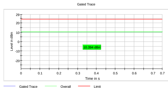
RMS Conducted Power, 5690 MHz, 802.11ax, HT80, MCS0, SISO
