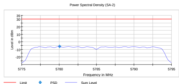
MCS15 -6.1 dBm
