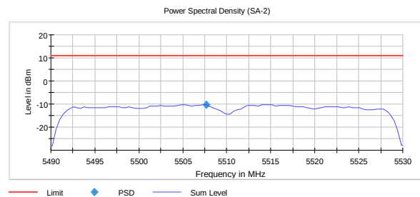
MCS11 -10.3 dBm
