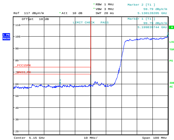
Band Edge 5150 MHz, ch042, 802.11ac MCS0, Radiated, Max
