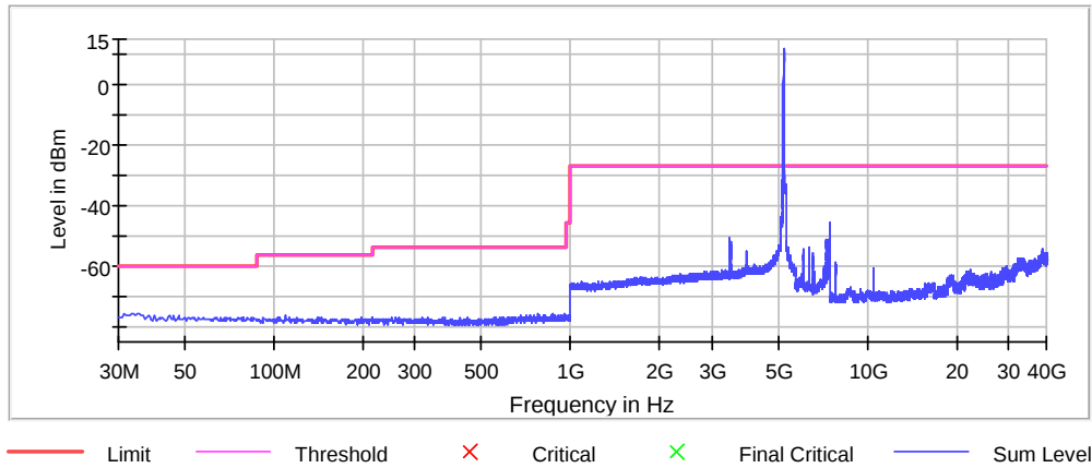
Spurious
