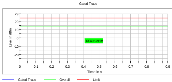
RMS Conducted Power, 5220 MHz, 802.11a, 6Mb
