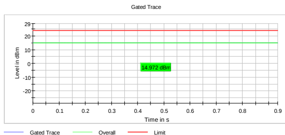
RMS Conducted Power, 5700 MHz, 802.11a, 6Mb
