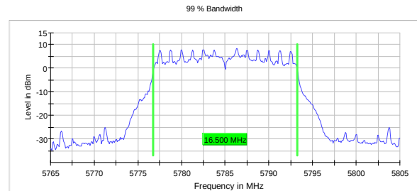
Occupied BW (99%), 5785 MHz, 802.11a, 6Mb
