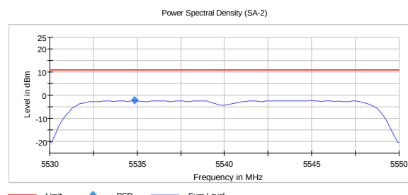
MCS15 -2.3 dBm
