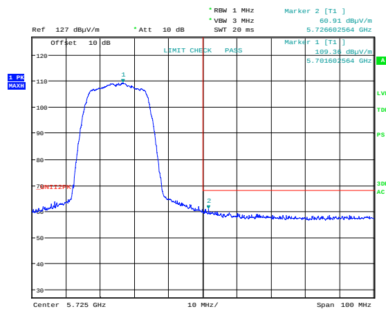
Band Edge 5725 MHz, ch140, 802.11n MCS7, Radiated, Max
