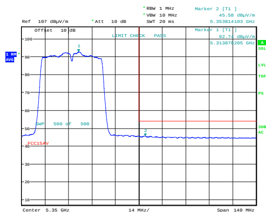
Band Edge, 5350 MHz, Ch062, 802.11n MCS0, Av, Max
