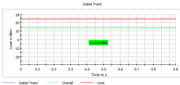
RMS Conducted Power, 5260 MHz, 802.11a, 6Mb
