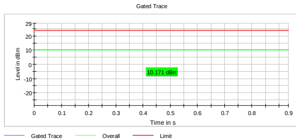
RMS Conducted Power, 5180 MHz, 802.11a, 6Mb
