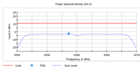
MCS15 -2.6 dBm
