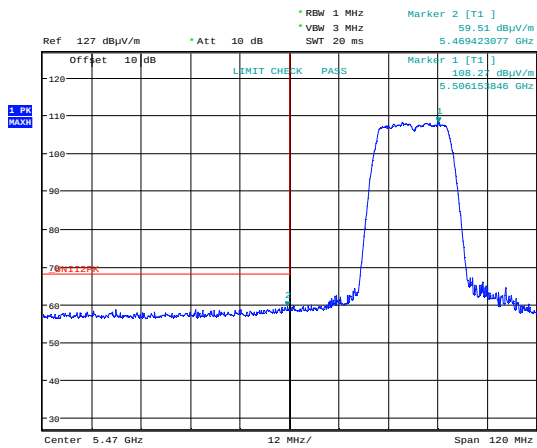
Band Edge 5470 MHz, ch100, 802.11n MCS0, Radiated, Max
