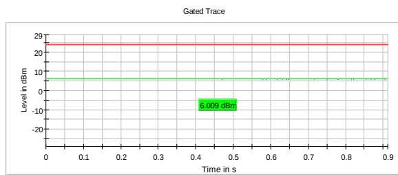
RMS Conducted Power, 5320 MHz, 802.11ax, HT20, MCS0, MIMO
