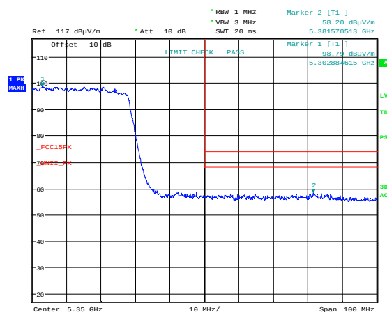
Band Edge 5350 MHz, ch058, 802.11ac MCS0 MIMO, Radiated, Max
