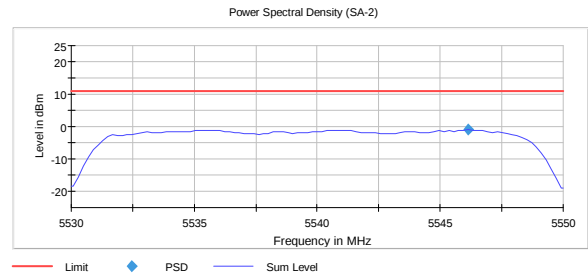
MCS7 -1.1 dBm
