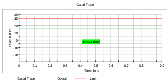
RMS Conducted Power, 5745 MHz, 802.11a, 6Mb
