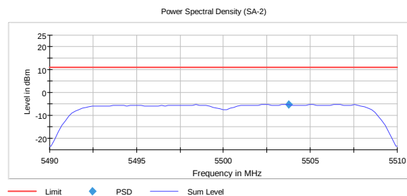
MCS15 -5.2 dBm
