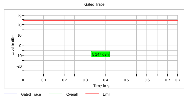
RMS Conducted Power, 5290 MHz, 802.11ax, HT80, MCS0, SISO
