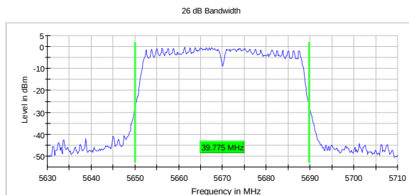
Emission BW (26 dB), 5670 MHz, 802.11ac, HT40, MCS0
