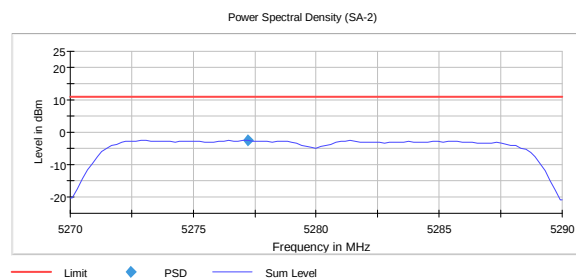
MCS15 -2.5 dBm
