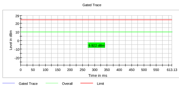
RMS Conducted Power, 5580 MHz, 802.11ax, HT20, MCS7, MIMO
