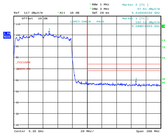
Band Edge 5350 MHz, ch058, 802.11ac MCS0, Radiated, Max
