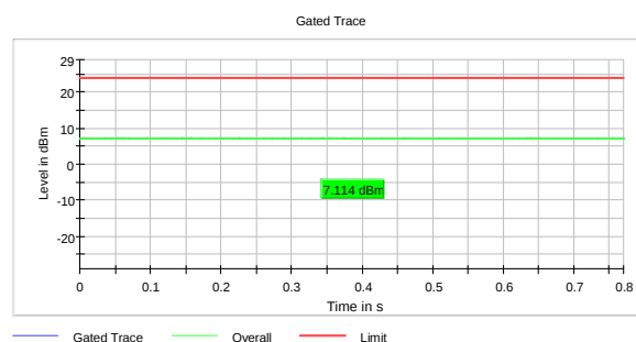
RMS Conducted Power, 5290 MHz, 802.11ac, HT80, MCS0, SISO
