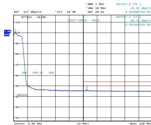
Band Edge, 5350 MHz, Ch056, 802.11n MCS7, Av, Max
