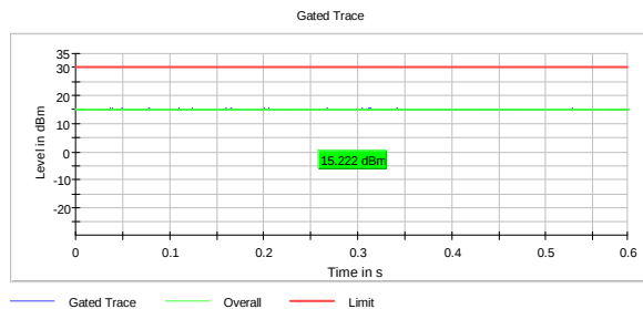
Output Power, 2437 MHz, 802.11ax MCS8
