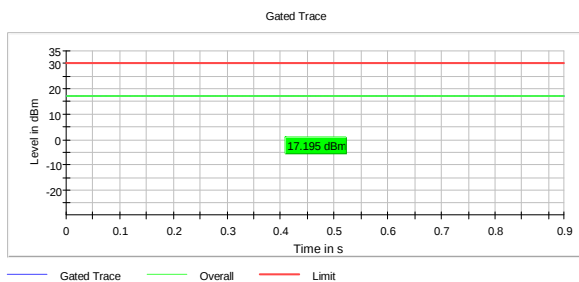
Output Power, 2452 MHz, 802.11n MCS0
