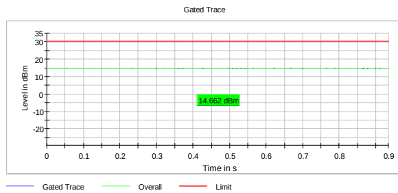
Output Power, 2462 MHz, 802.11g 6M
