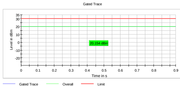
Output Power, 2447 MHz, 802.11g 6M
