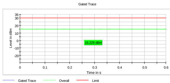
Output Power, 2422 MHz, 802.11ax MCS8
