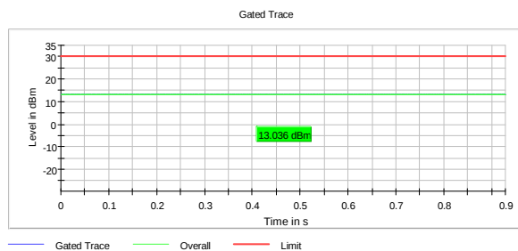
Output Power, 2412 MHz, 802.11n MCS0
