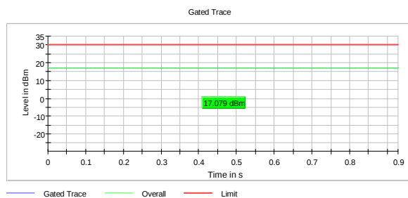
Output Power, 2422 MHz, 802.11n MCS0
