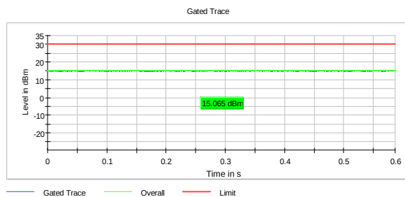
Output Power, 2452 MHz, 802.11ax MCS8
