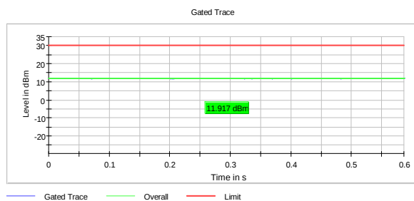
Output Power, 2462 MHz, 802.11ax MCS8
