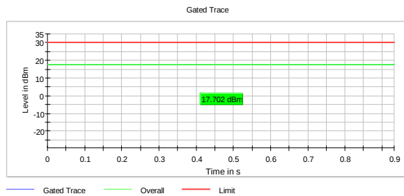
Output Power, 2452 MHz, 802.11g 6M
