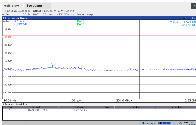
Conducted Emissions 10-2350 MHz, 2480 MHz, 1Mb
