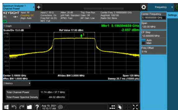
Antenna B
