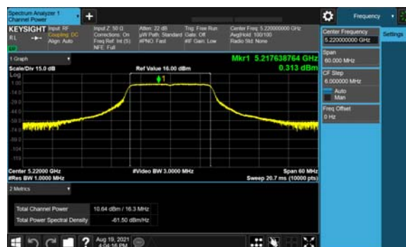
Antenna B
