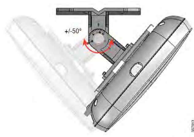
Figure 26: Single Axis Mount Pivot Adjustment
