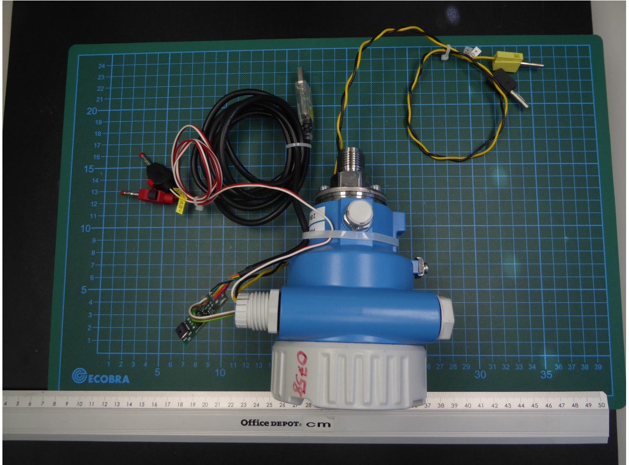
EUT (EUT VE101_A_03) in dedicated housing – side view 2
