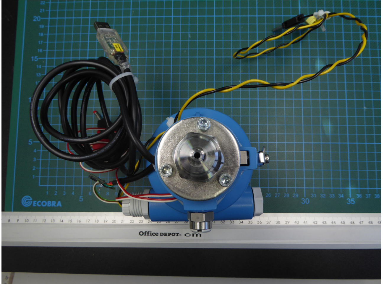
EUT (EUT VE101_A_03) in dedicated housing – top view
