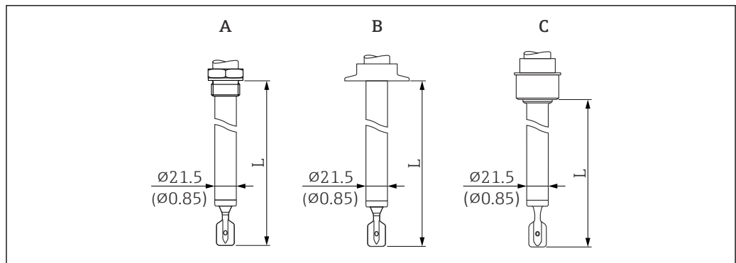
AP 17 Probe designs: pipe extension, short pipe (sensor length L). Unit of measurement mm (in)
