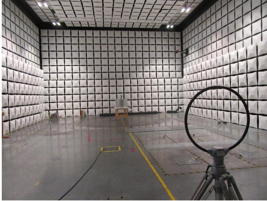
Figure 4 - Test setup for radiated emission on TLPR
