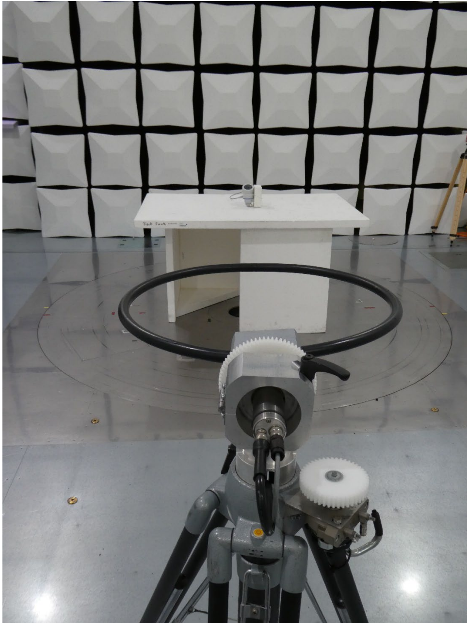
Antenna position 3, EUT Position 1
