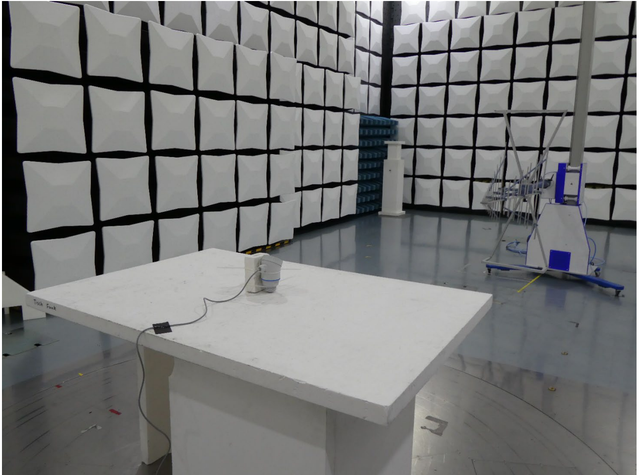
EUT – Position 1
