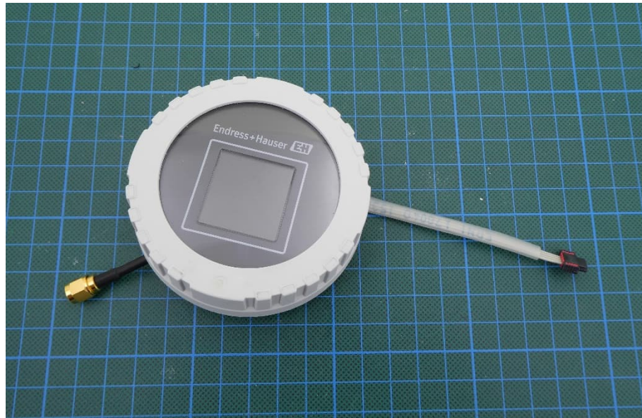
EUT for conducted tests - top view
