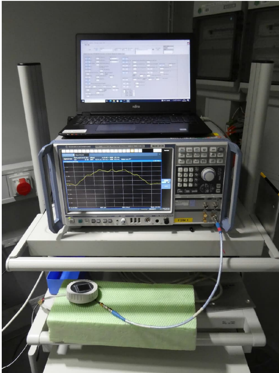
Test setup – conducted @ antenna port
