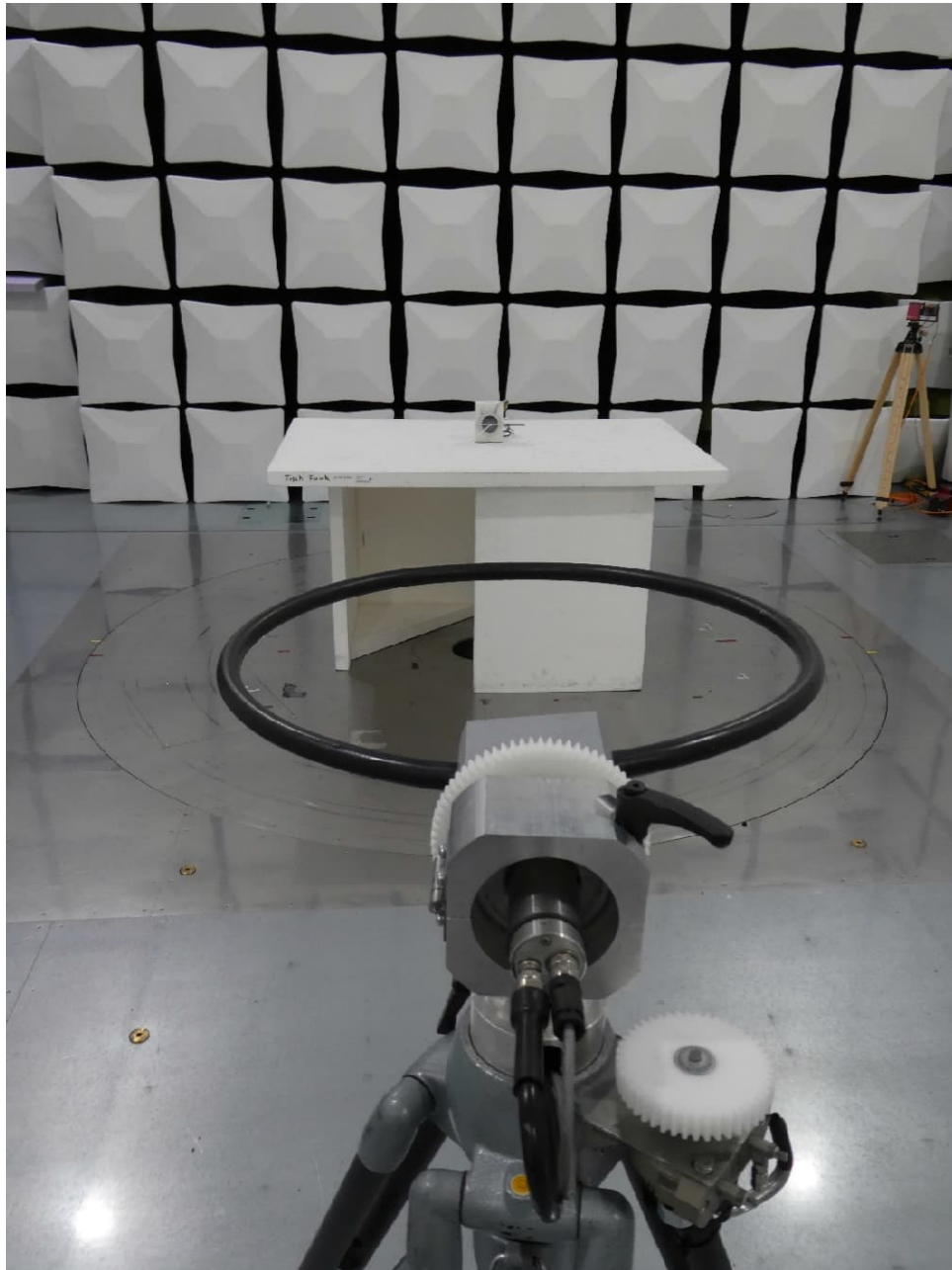
Antenna position 3, EUT position 3
