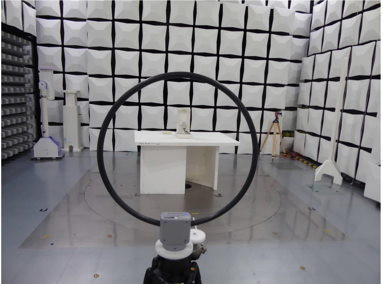
Antenna position 1
