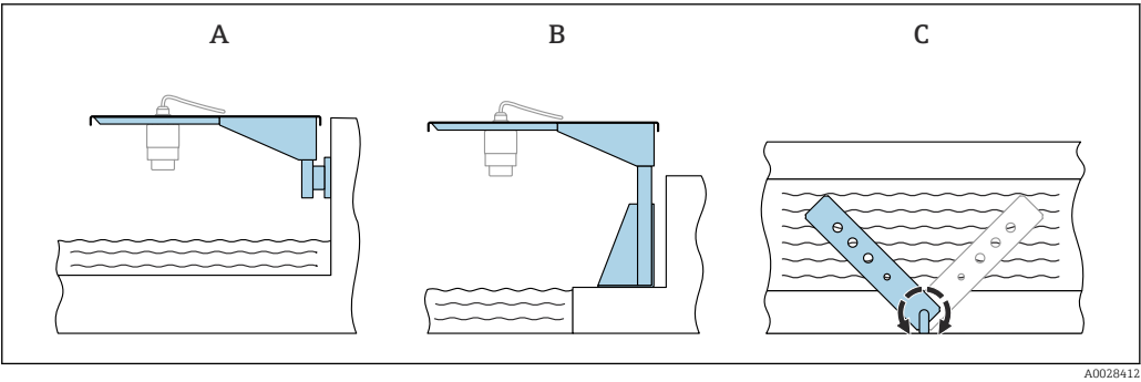
13 Cantilever installation, with pivot
