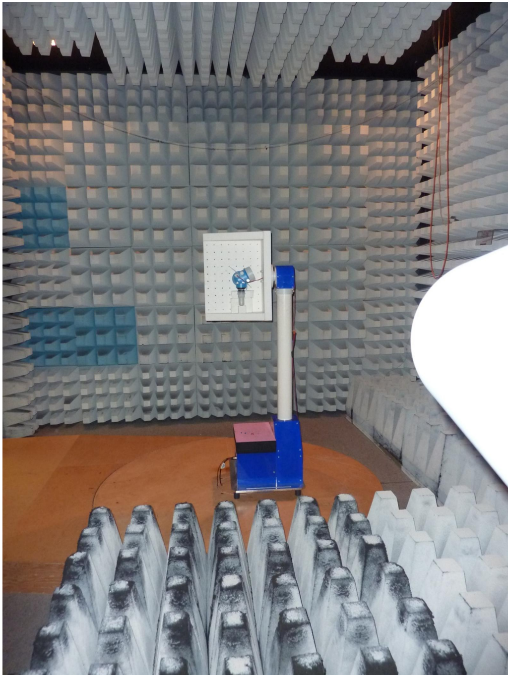
172289_203.JPG: ProTof BTLE-adaptor 2.4 GHz inside FMR50, test setup fully anechoic chamber (1 GHz to 12 GHz)
