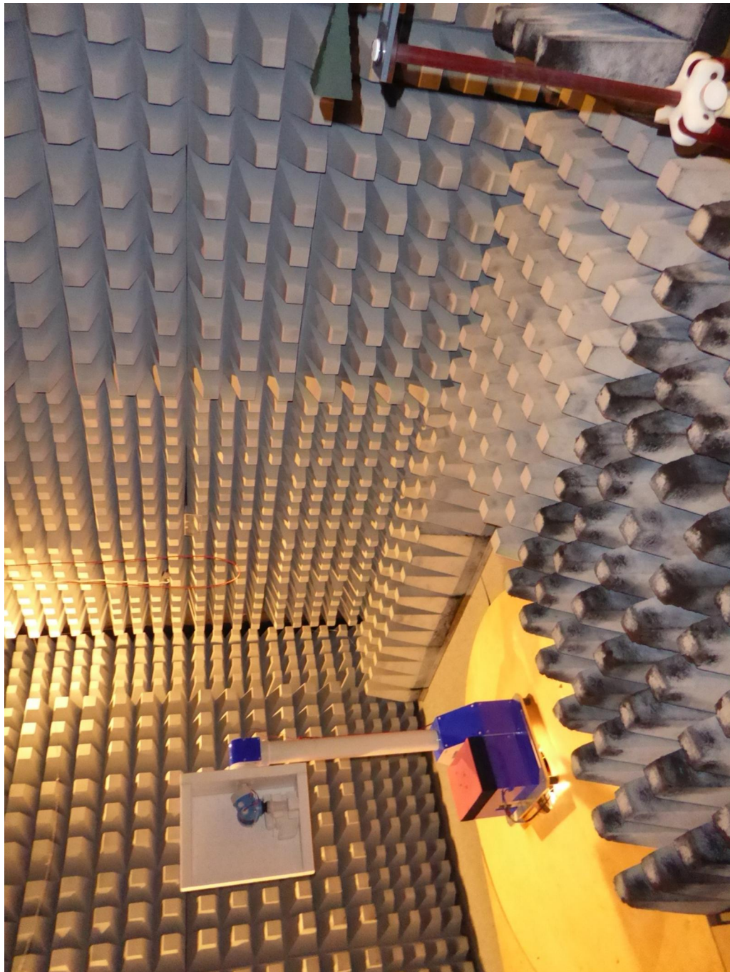
172289_204.JPG: ProTof BTLE-adaptor 2.4 GHz inside FMR50, test setup fully anechoic chamber (12 GHz to 26.5 GHz)
