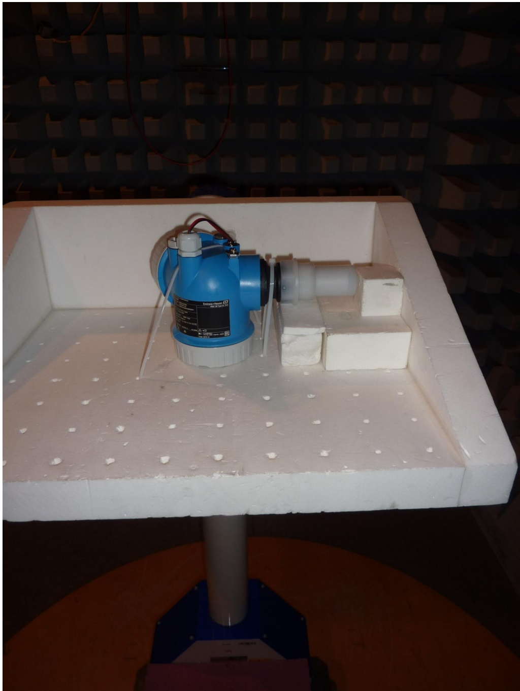
172289_202.JPG: ProToF BTLE-adaptor 2.4 GHz inside FMR50, test setup fully anechoic chamber (pos. 2)
