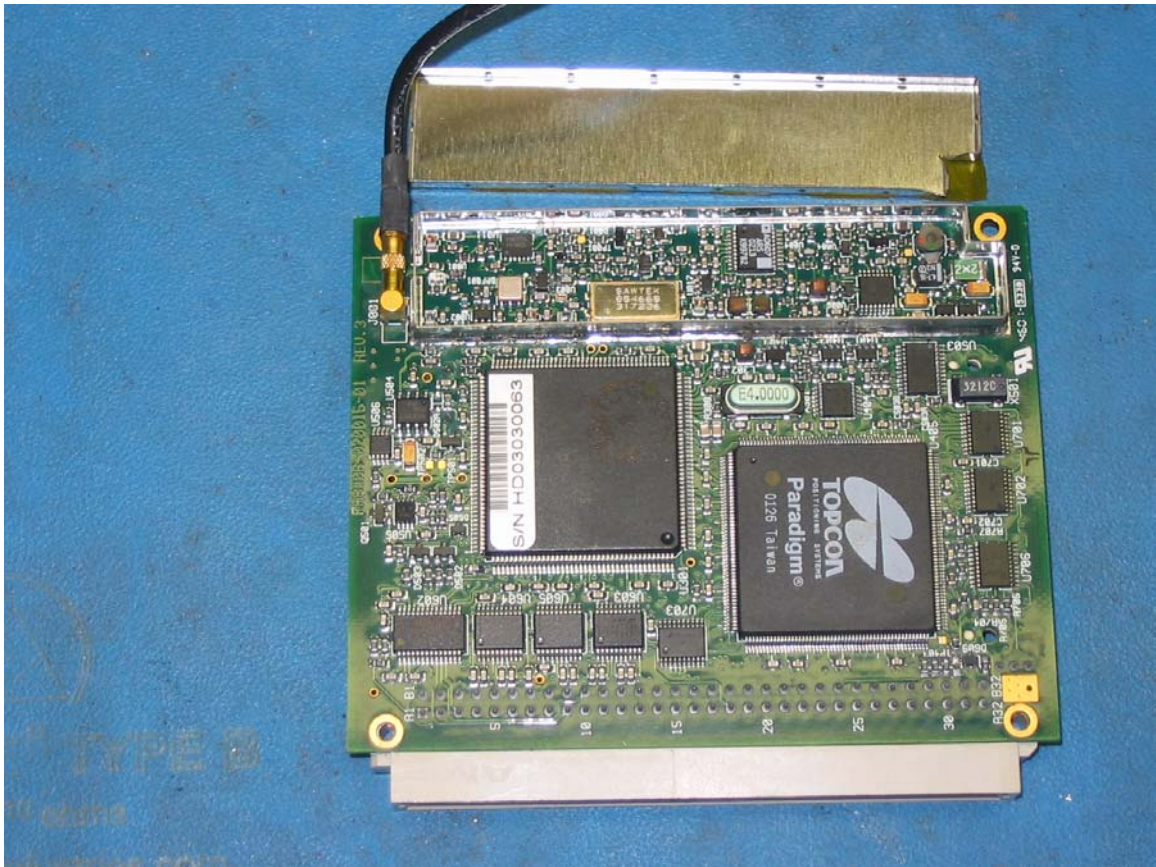
GPS Board
