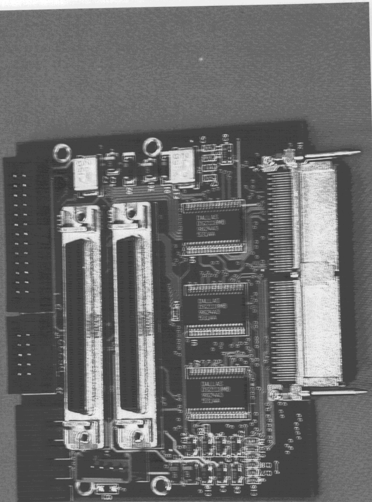
PHOTO 11. EUT COMPONENT SIDE VIEW
