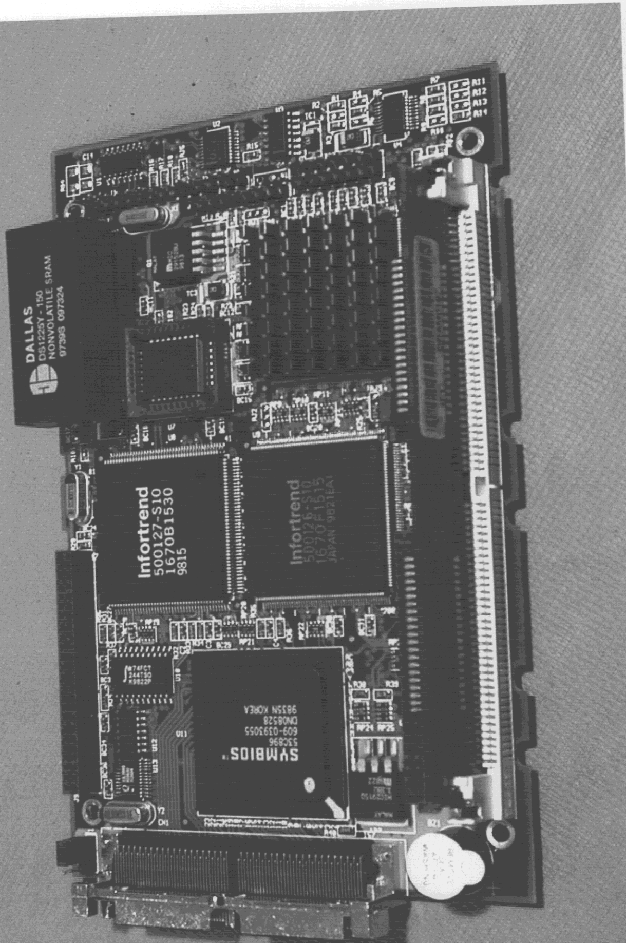
PHOTO 7. EUT COMPONENT SIDE VIEW
