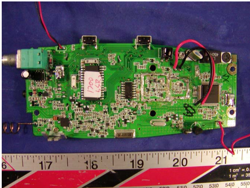
EUT – Component View with Shielding Removed
