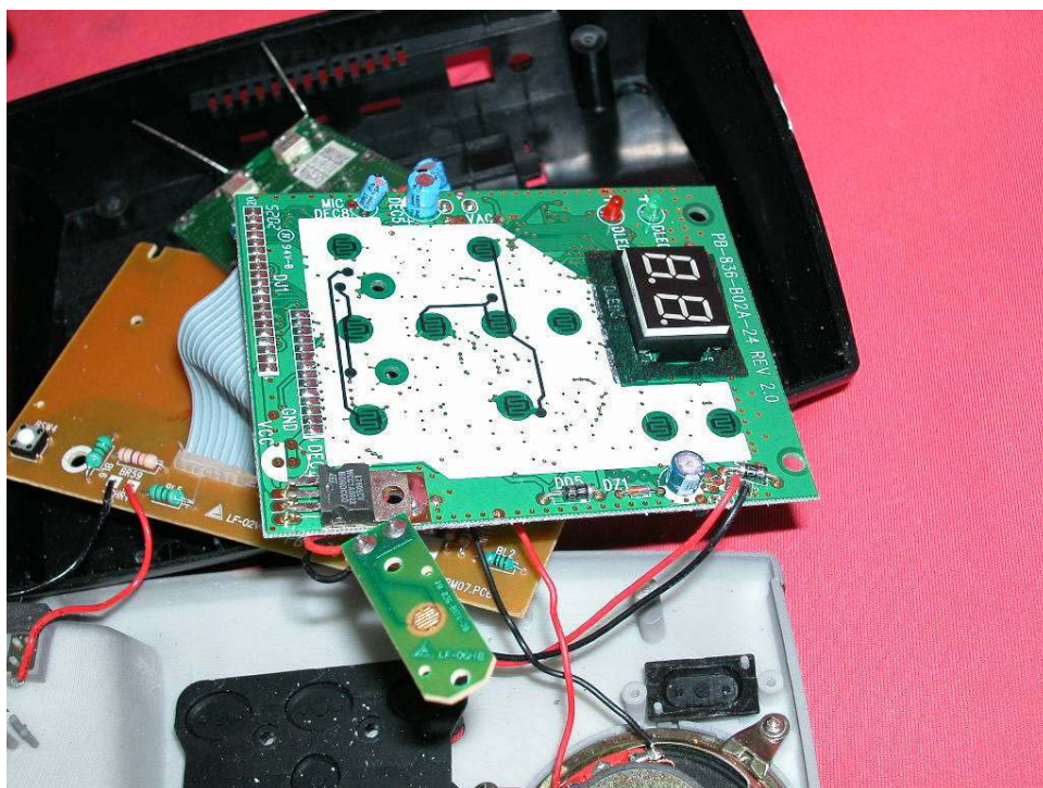
Base Answering Machine PCB keypad side
