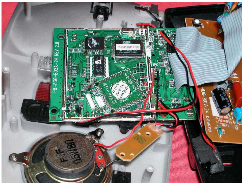
Base Answering Machine PCB comp side (View 1)
