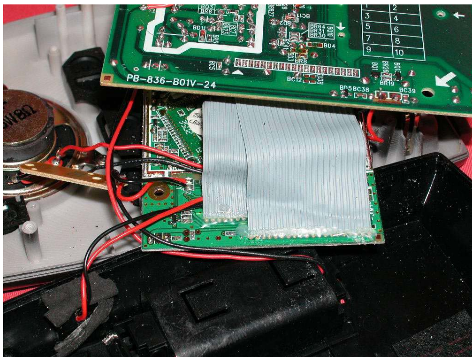
Base Answering Machine PCB comp side (View 2)
