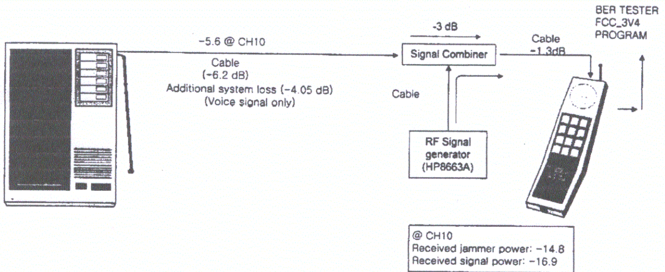
Figure 1: Test set-up
