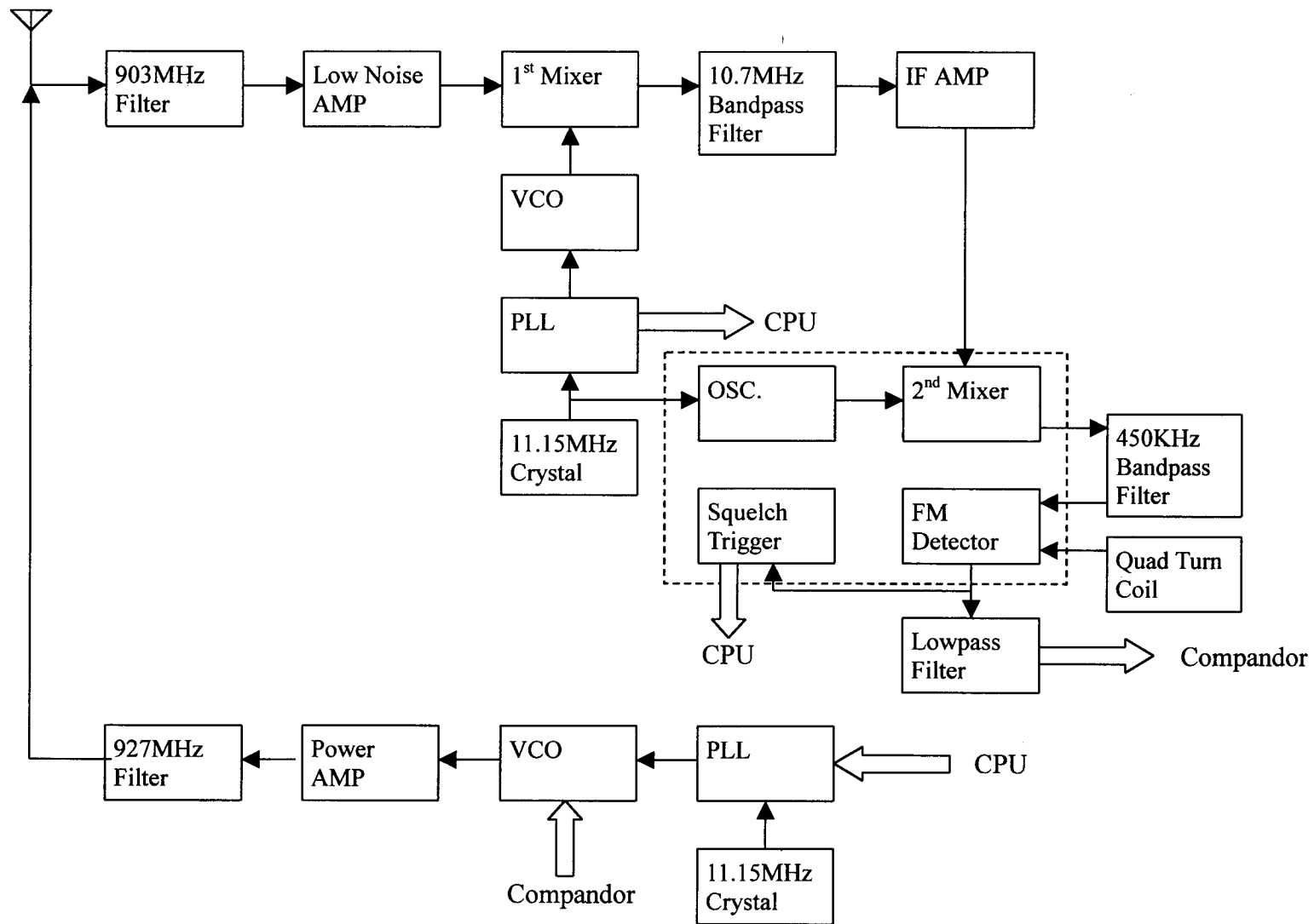
FF2125/FF2150 900MHz phone handset RF module block diagram
