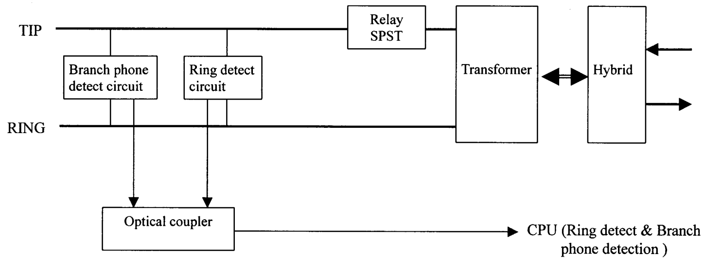
FF2125 900MHz phone base line interface block diagram
