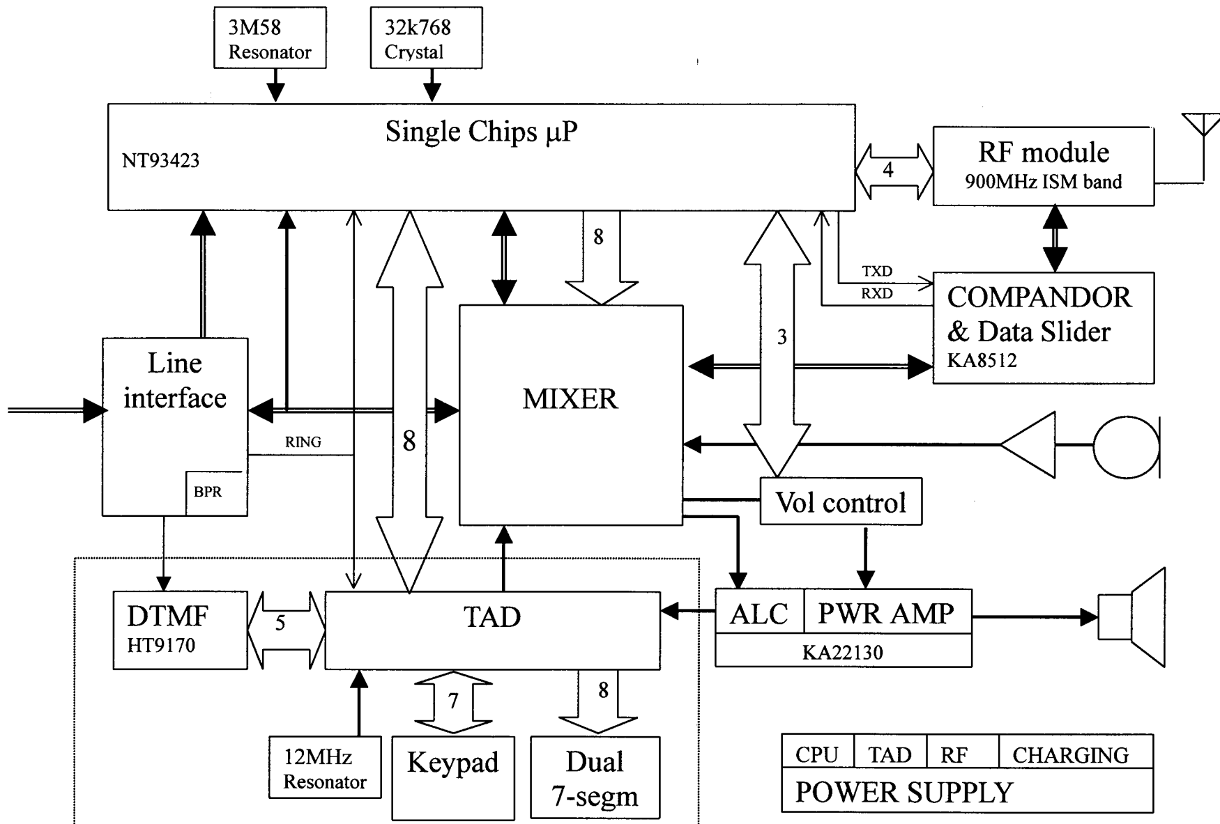
FF2125 900MHz phone Base block diagram
