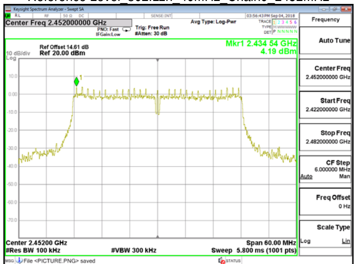
Reference Level 802.11n 40MHz Chain0 2452MHz
