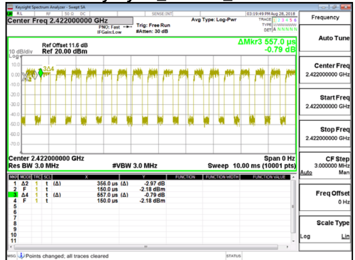
Duty Cycle_802.11n_40MHz
